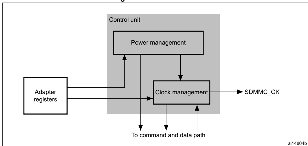
Figure 236. Control unit
