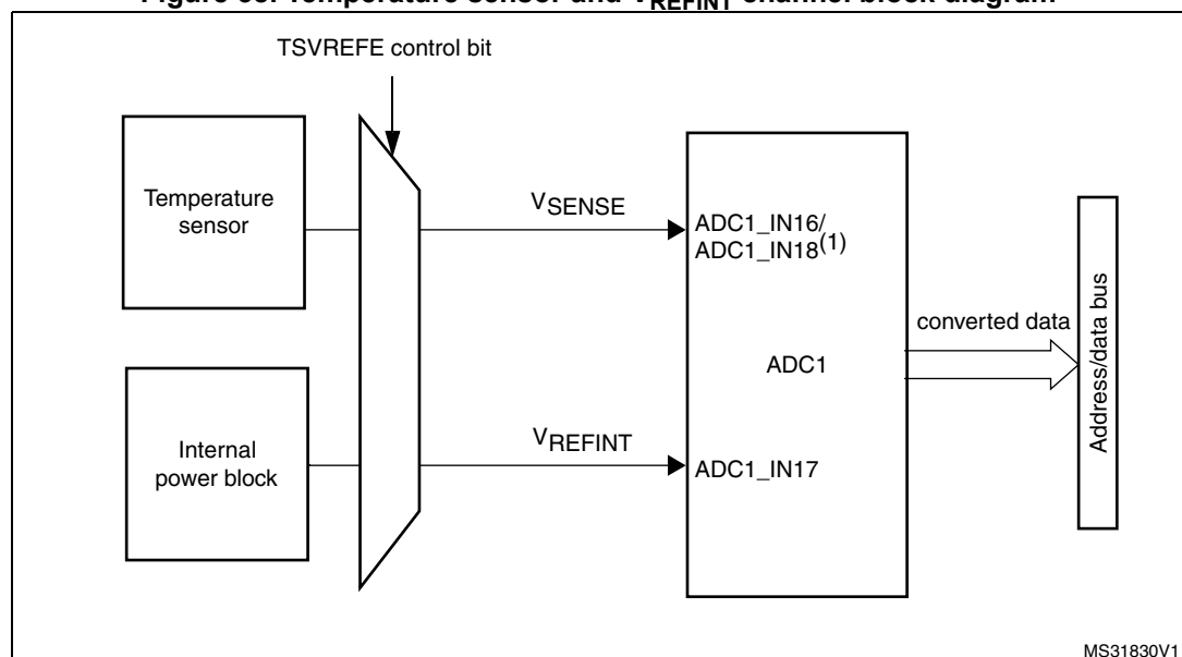
Figure 38. Temperature sensor and V_{\text{REFINT}} channel block diagram
