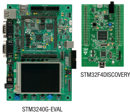
STM3240G-EVAL
