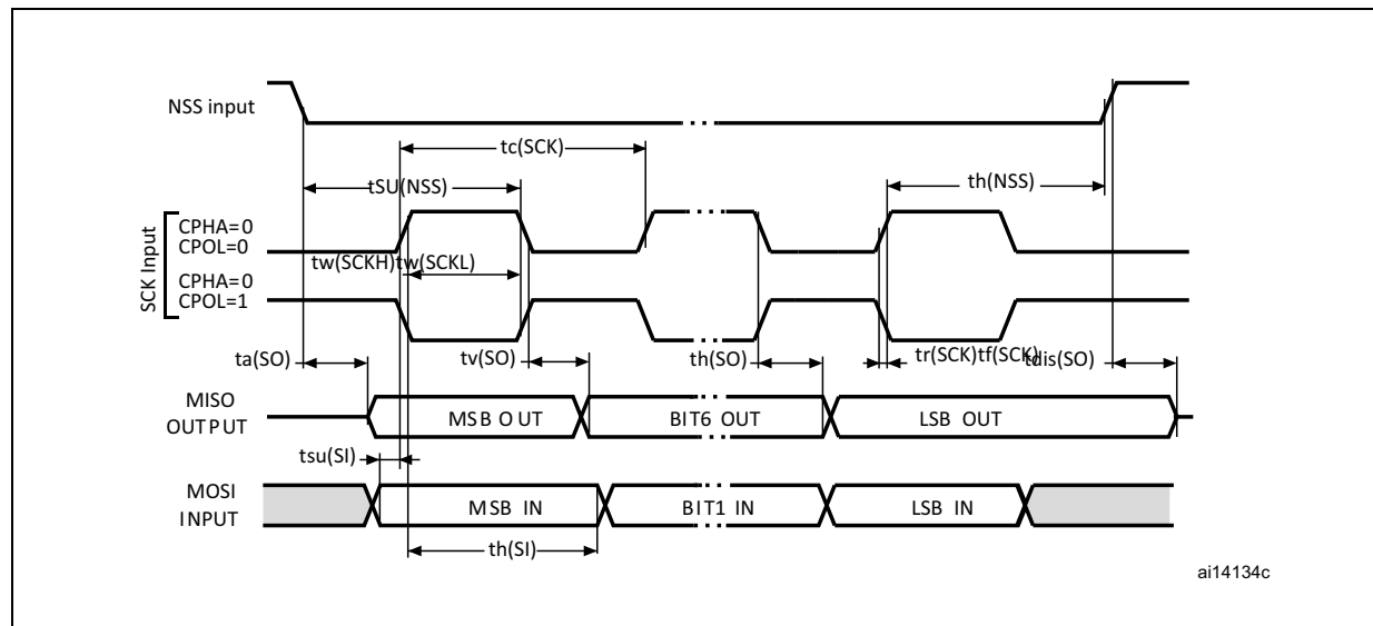
Figure 20. SPI timing diagram - slave mode and CPHA = 0
