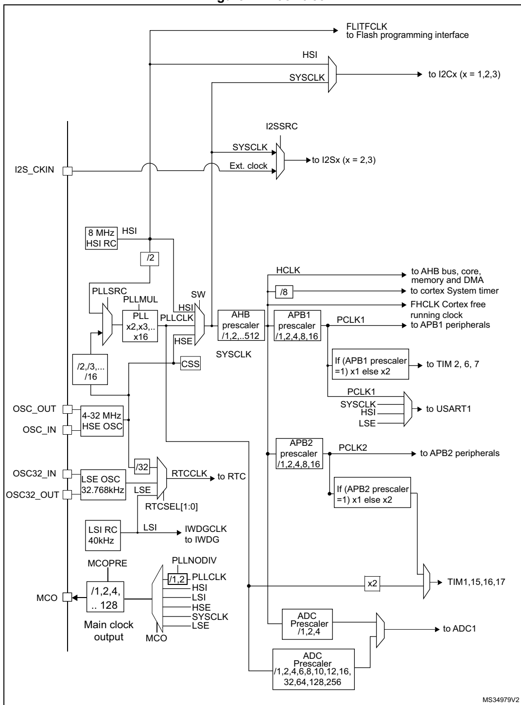
Figure 2. Clock tree
