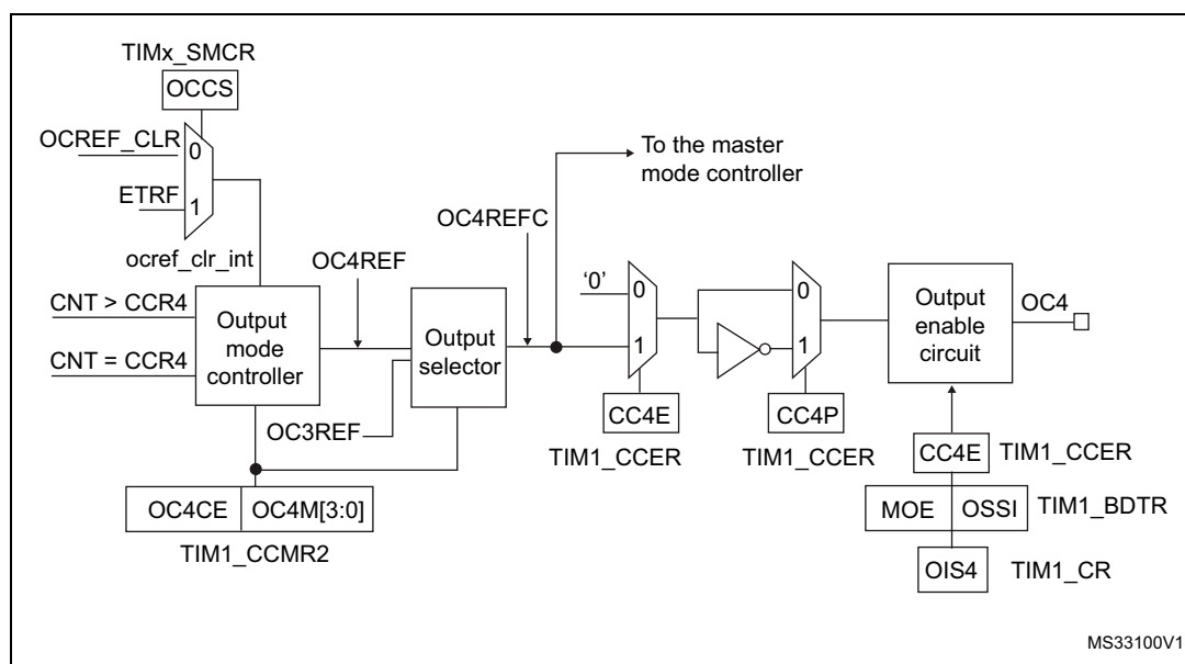
Figure 170. Output stage of capture/compare channel (channel 4)
