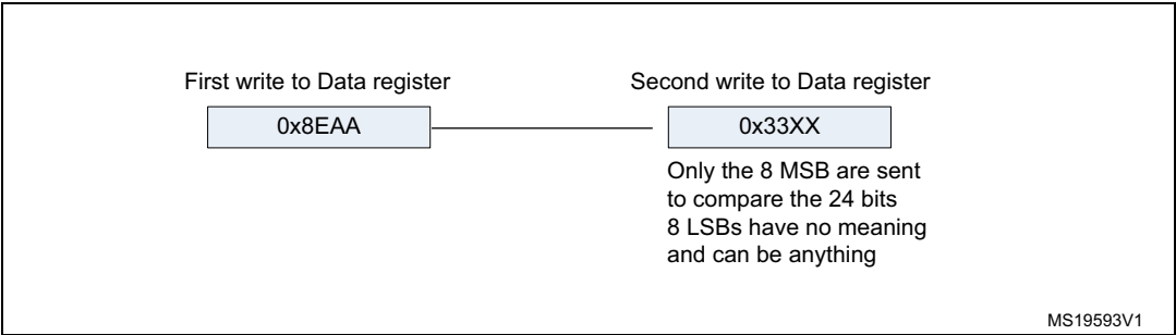
Figure 368. Transmitting 0x8EAA33
