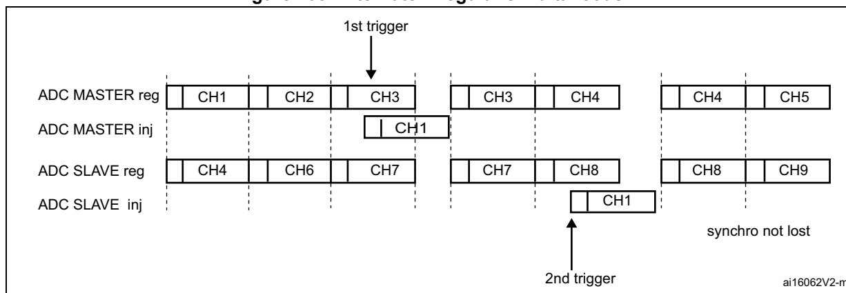
Figure 105. Alternate + regular simultaneous
