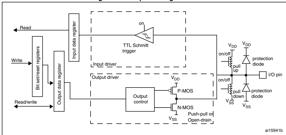
Figure 43. Output configuration
