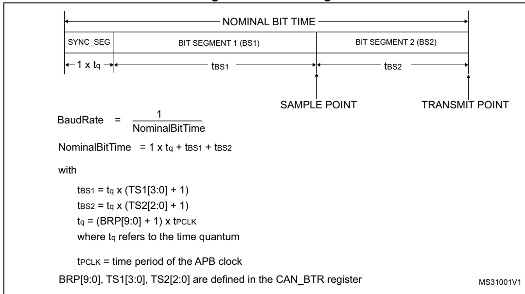
Figure 397. Bit timing
