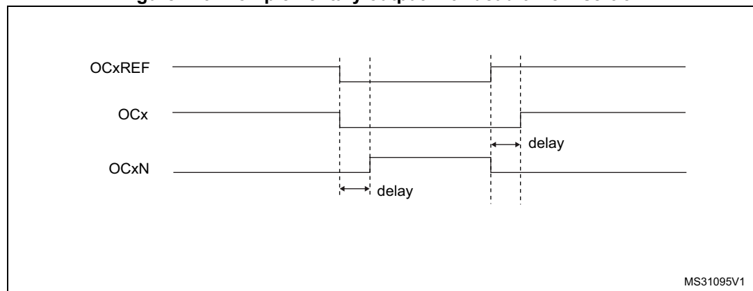
Figure 179. Complementary output with dead-time insertion
