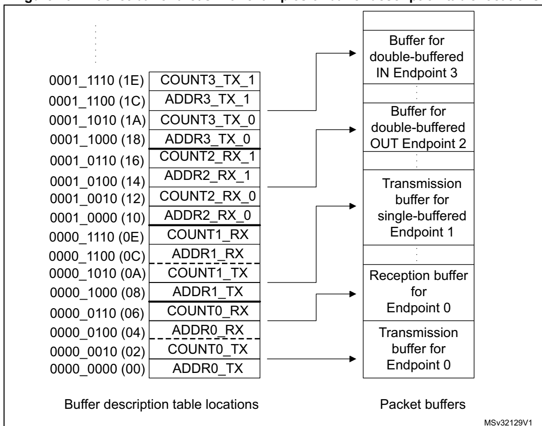
Figure 402. Packet buffer areas with examples of buffer description table locations
