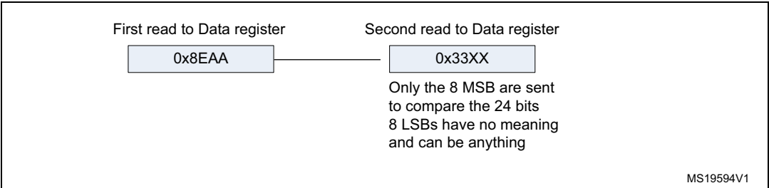
Figure 369. Receiving 0x8EAA33
