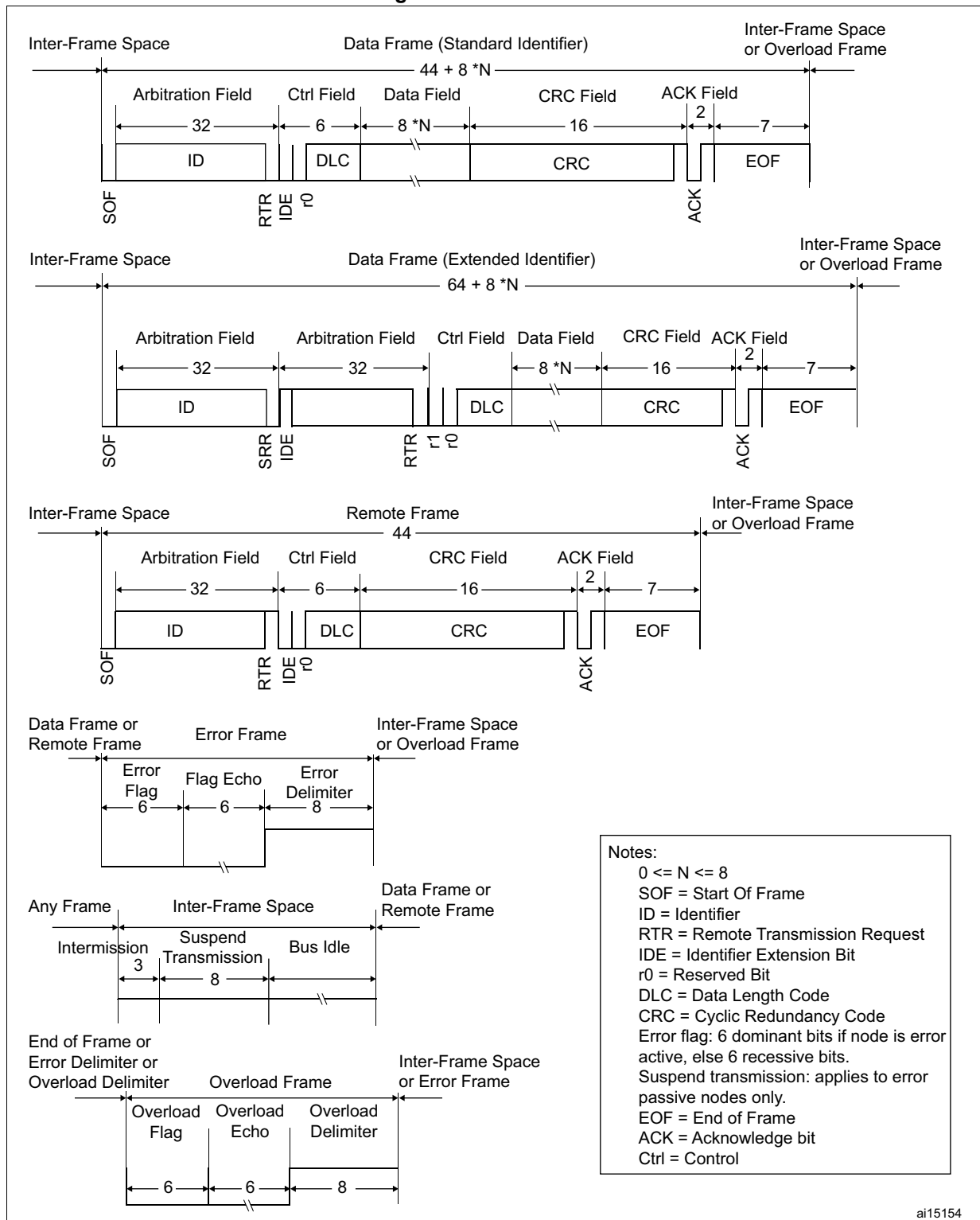
Figure 398. CAN frames
