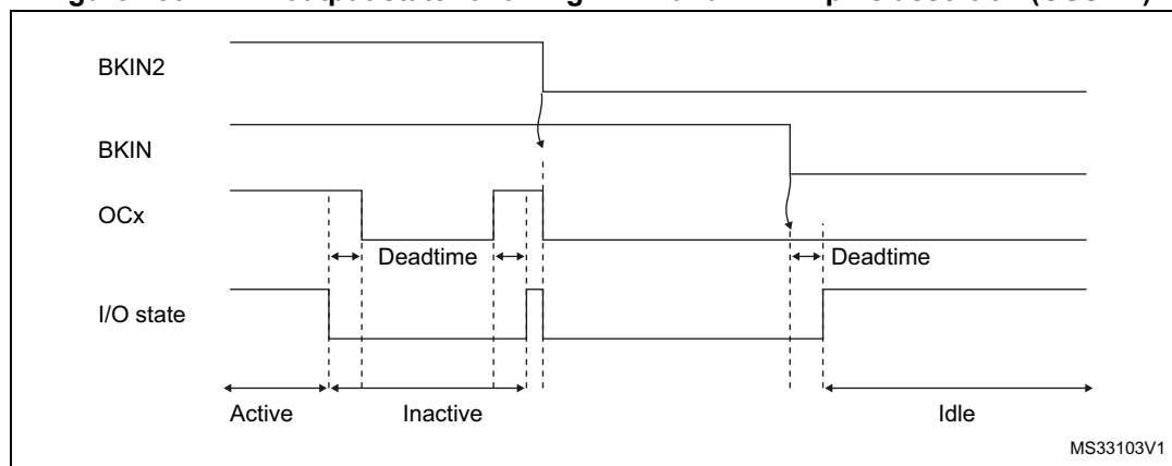
Figure 183. PWM output state following BKIN and BKIN2 pins assertion (OSSR=1)
