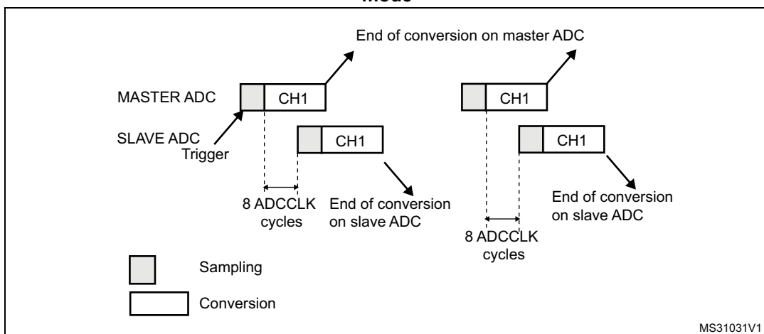
Figure 101. Interleaved mode on 1 channel in single conversion mode: dual ADC mode
