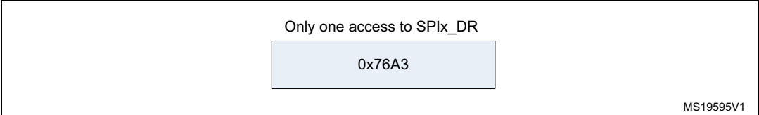
Figure 371. Example of 16-bit data frame extended to 32-bit channel frame
