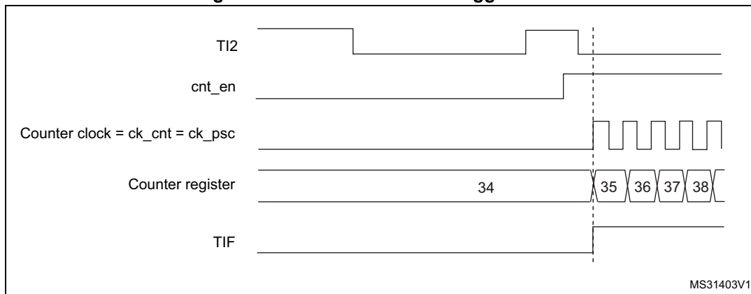
Figure 195. Control circuit in trigger mode
