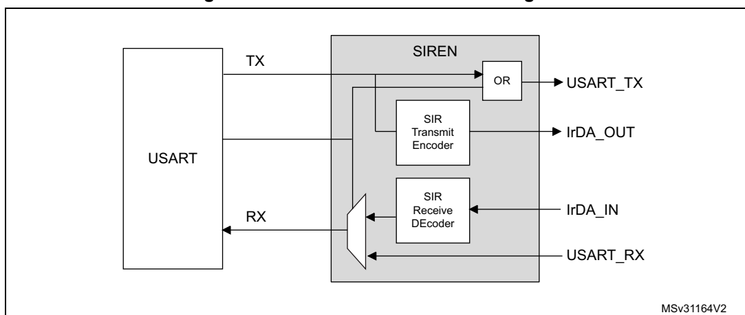
Figure 340. IrDA SIR ENDEC- block diagram
