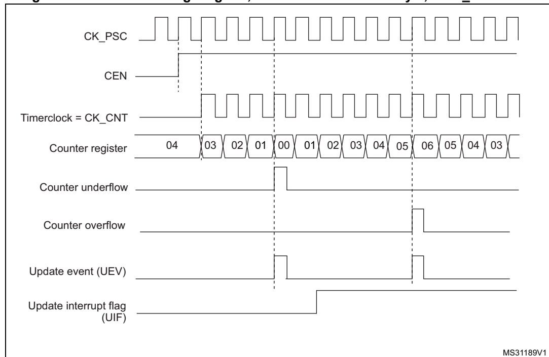
Figure 154. Counter timing diagram, internal clock divided by 1, TIMx_ARR = 0x6
