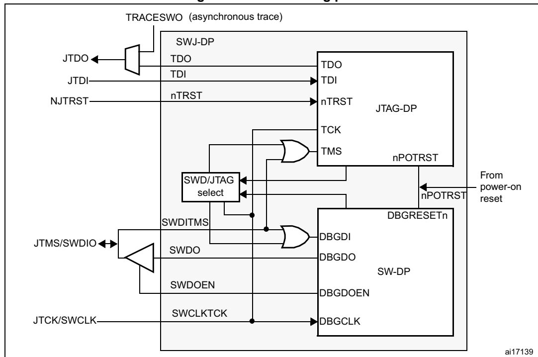
Figure 404. SWJ debug port
