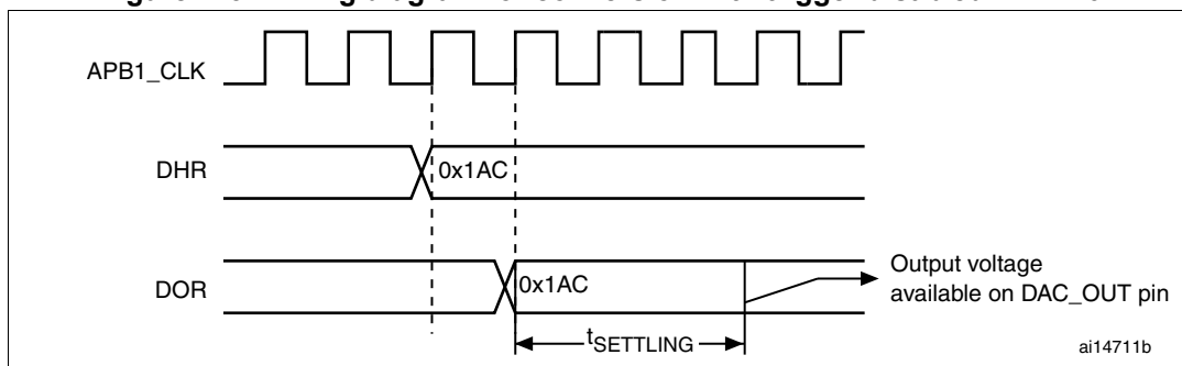
Figure 113. Timing diagram for conversion with trigger disabled TEN = 0
