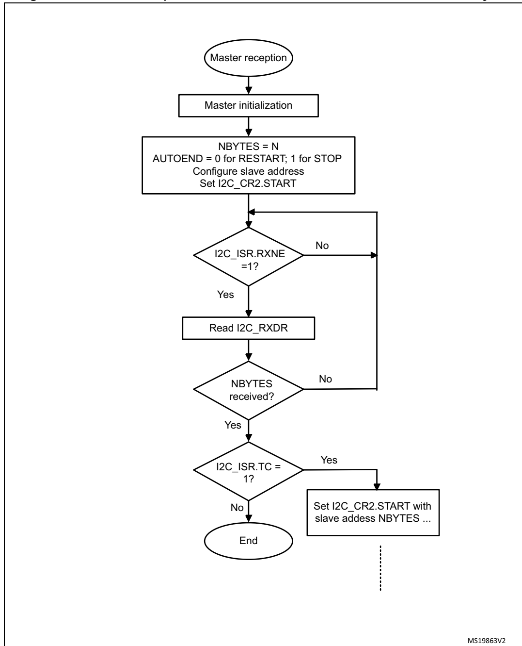
Figure 304. Transfer sequence flowchart for I2C master receiver for N \leq 255 bytes
