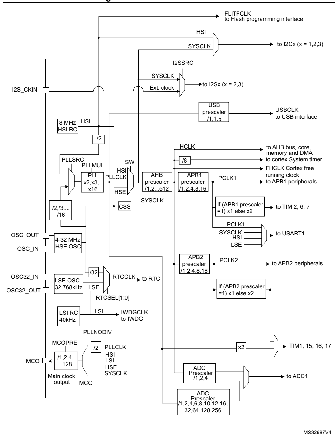
Figure 14. STM32F302x6/8 clock tree
