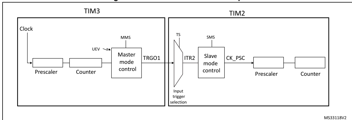
Figure 232. Master/Slave timer example
