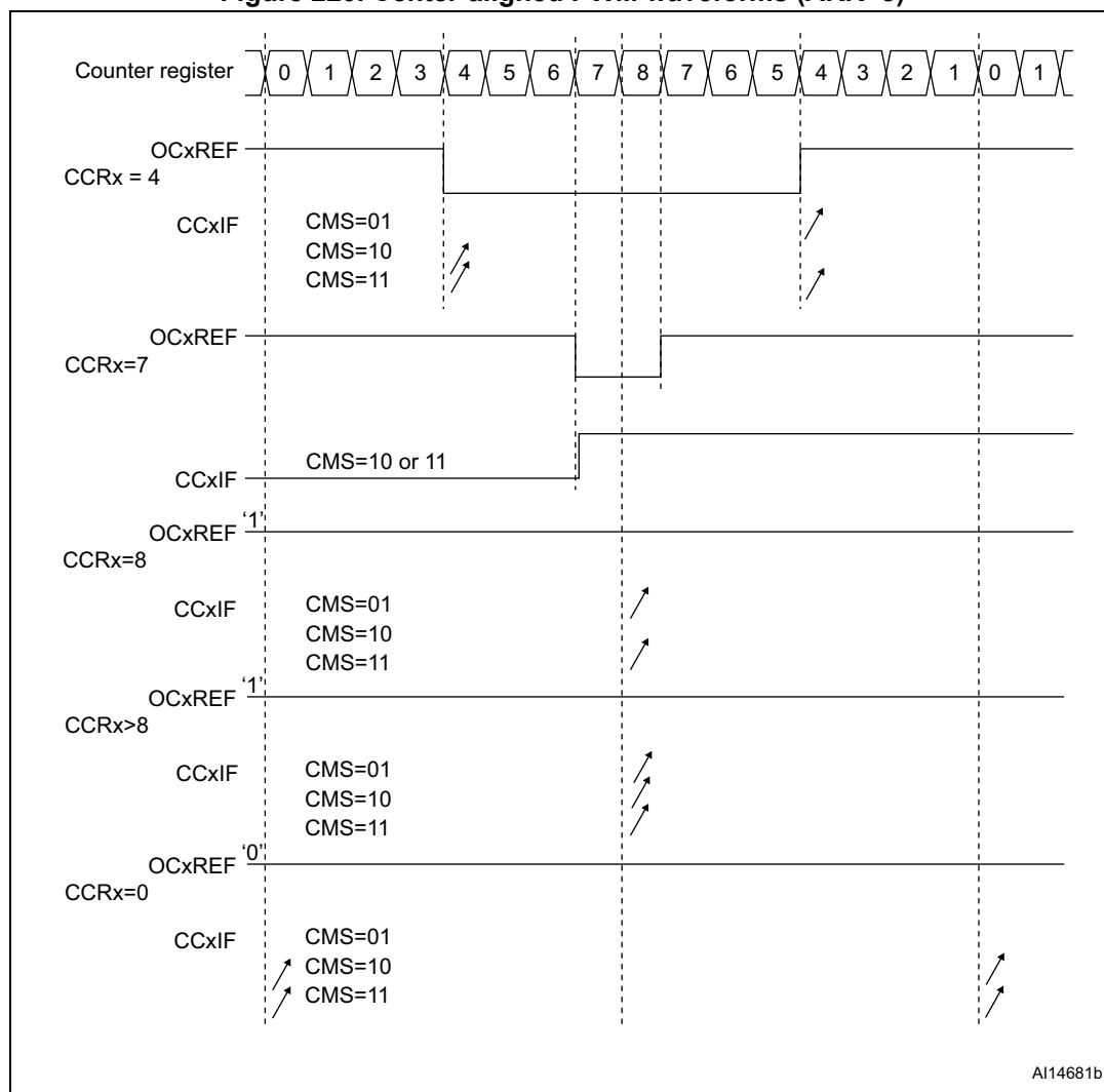
Figure 220. Center-aligned PWM waveforms (ARR=8)
