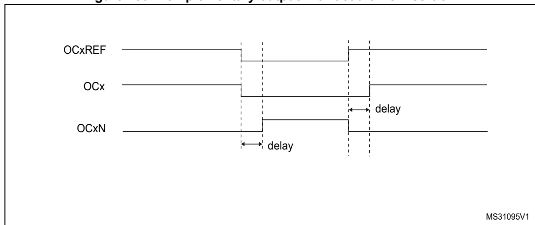
Figure 260. Complementary output with dead-time insertion.
