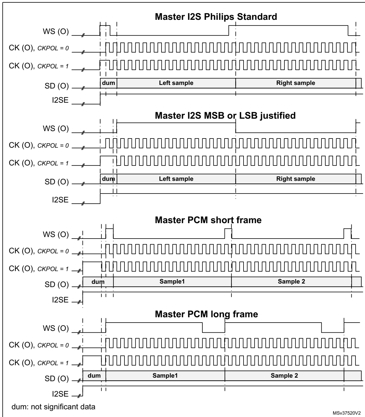
Figure 375. Start sequence in master mode
