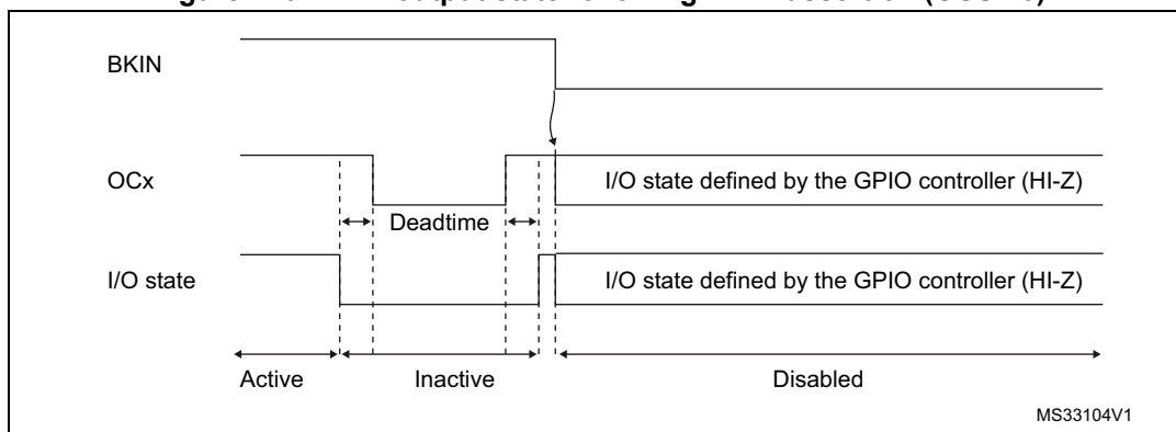
Figure 176. PWM output state following BKIN assertion (OSS1=0)
