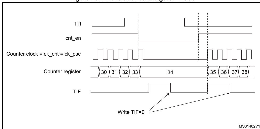
Figure 267. Control circuit in gated mode
