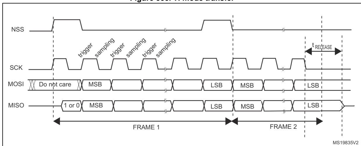
Figure 355. TI mode transfer
