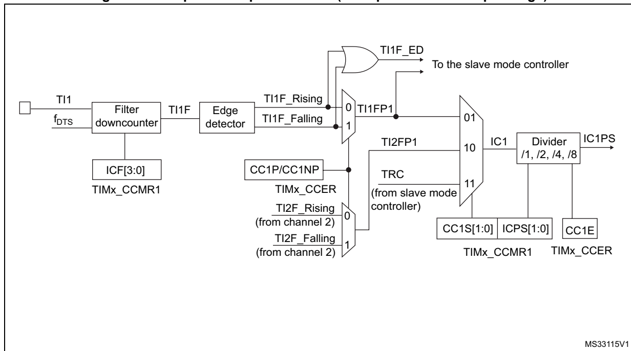
Figure 214. Capture/compare channel (example: channel 1 input stage)
