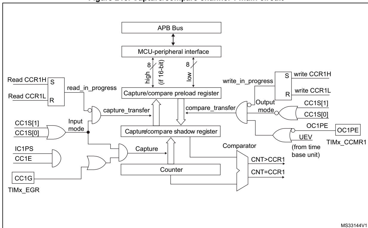
Figure 215. Capture/compare channel 1 main circuit
