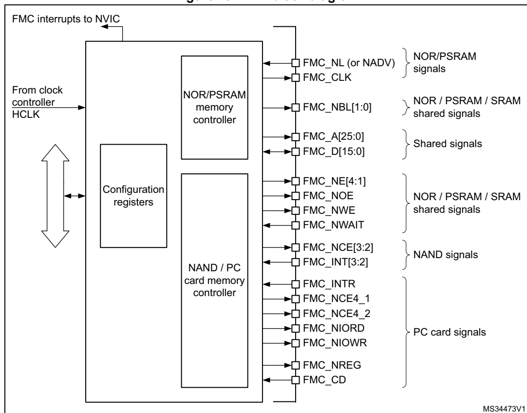
Figure 29. FMC block diagram
