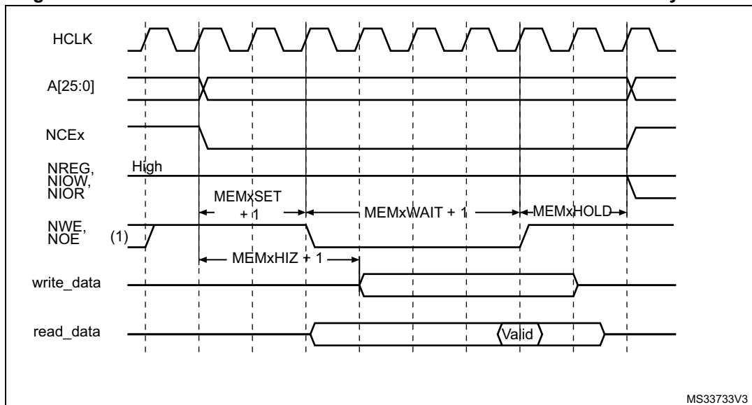
Figure 49. NAND Flash/PC Card controller waveforms for common memory access
