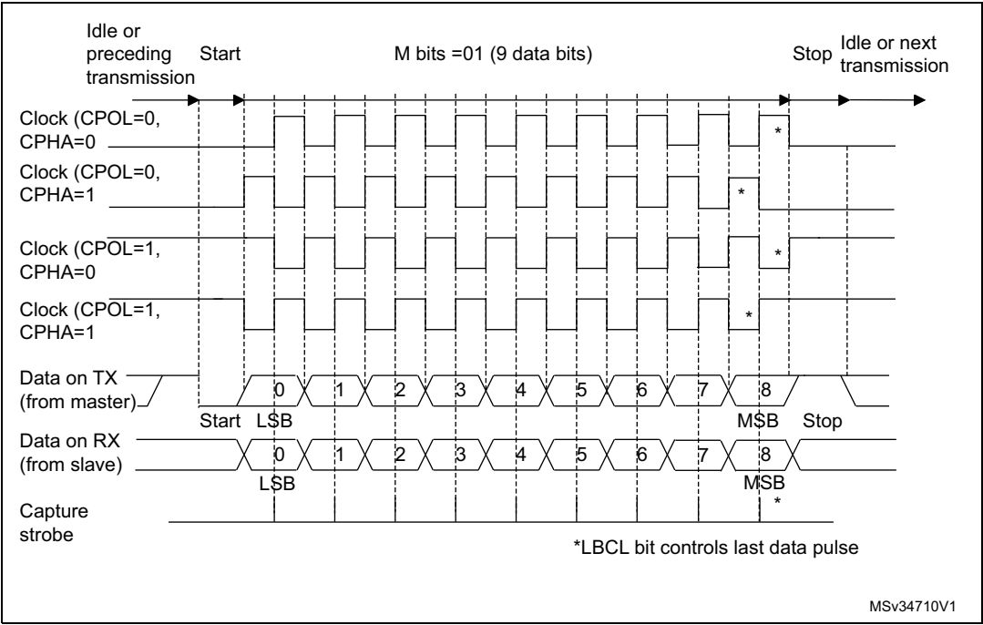
Figure 328. USART data clock timing diagram (M bits = 01)
