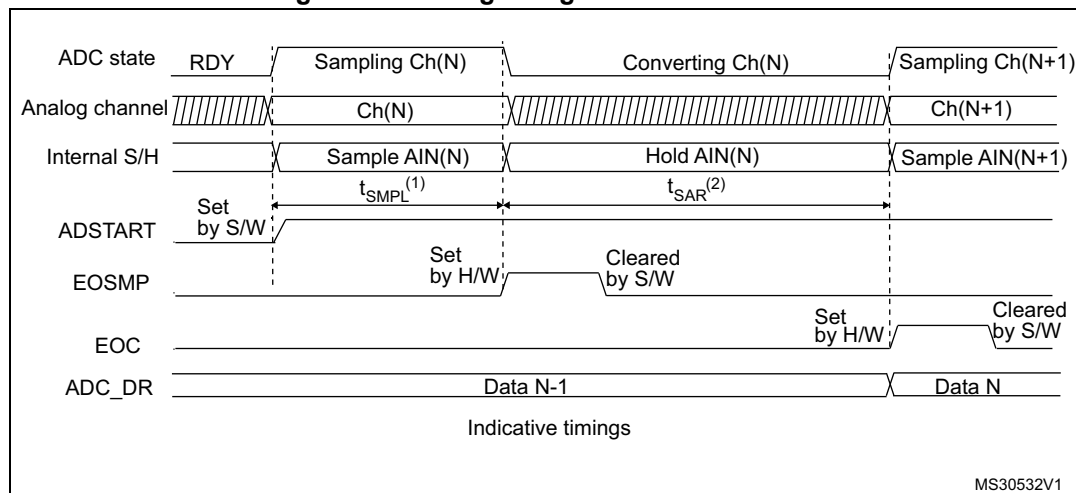
Figure 58. Analog to digital conversion time
