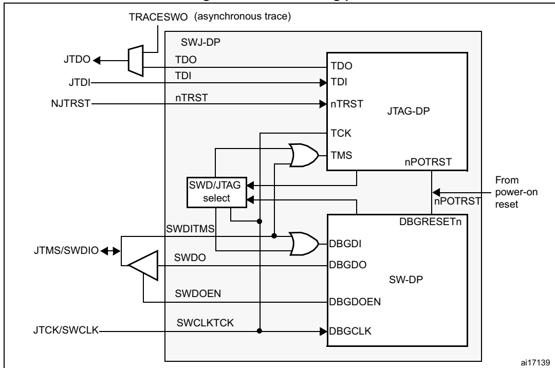
Figure 396. SWJ debug port
