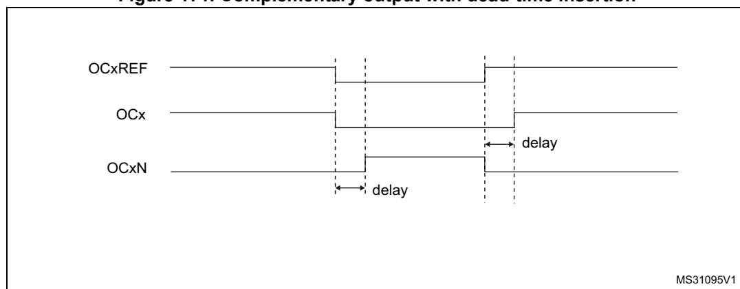
Figure 171. Complementary output with dead-time insertion
