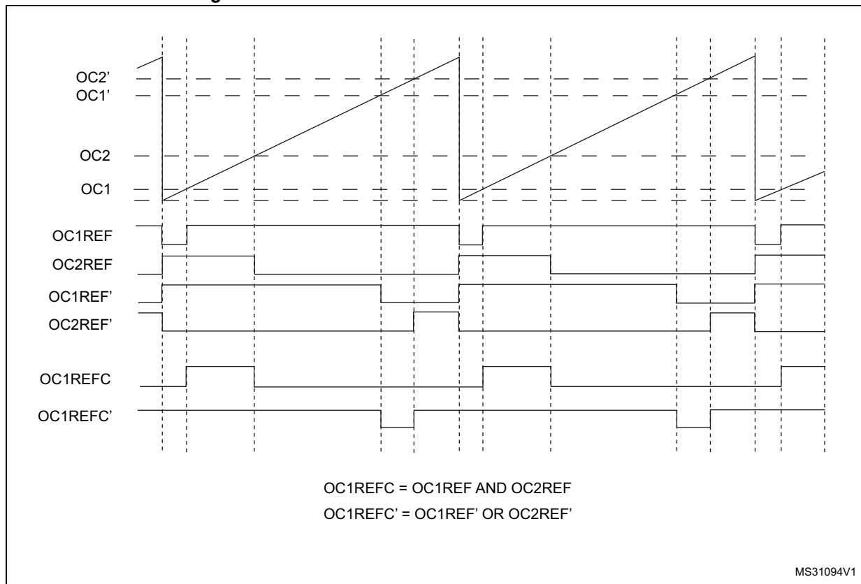
Figure 222. Combined PWM mode on channels 1 and 3
