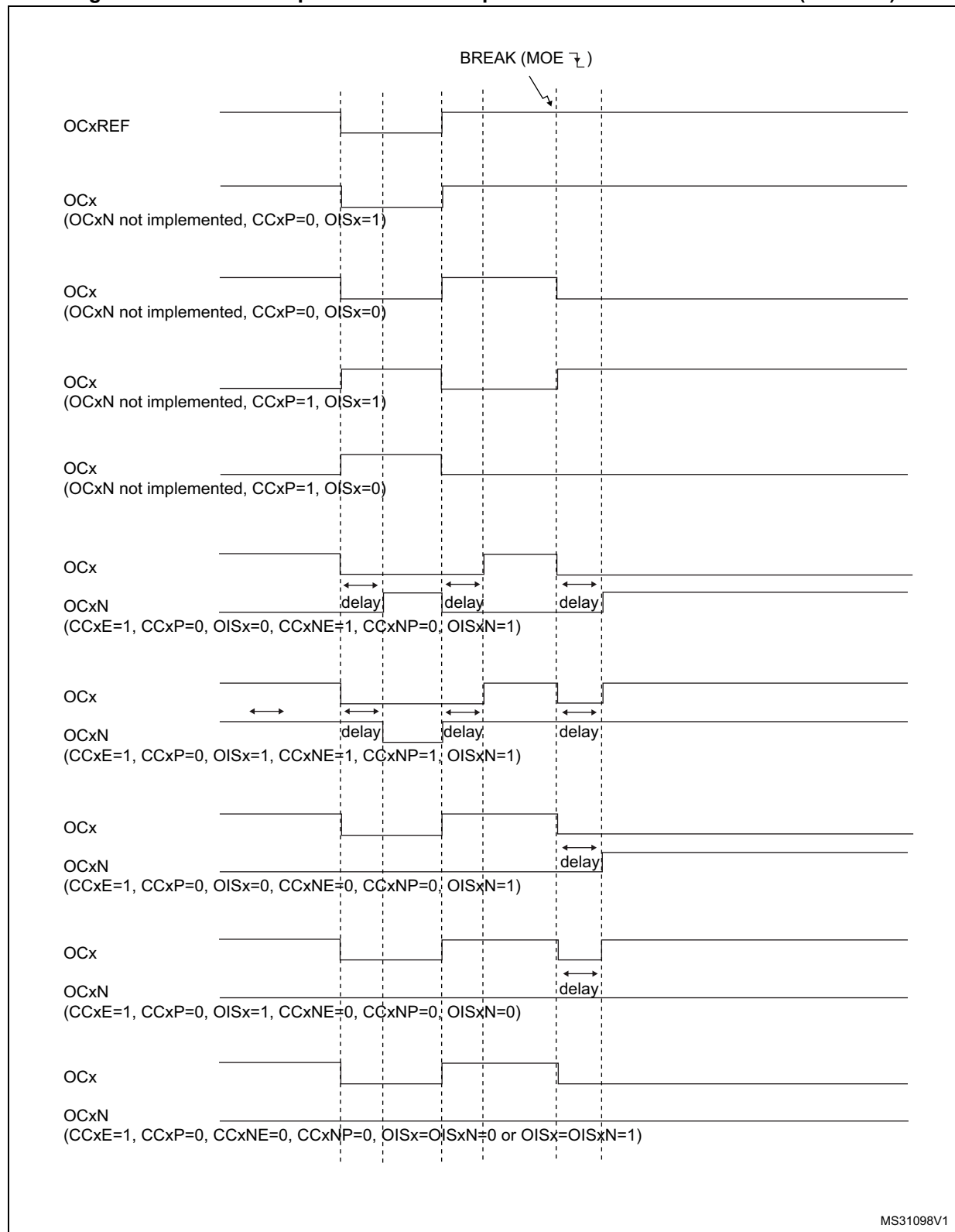
Figure 174. Various output behavior in response to a break event on BKIN (OSSR = 1)
