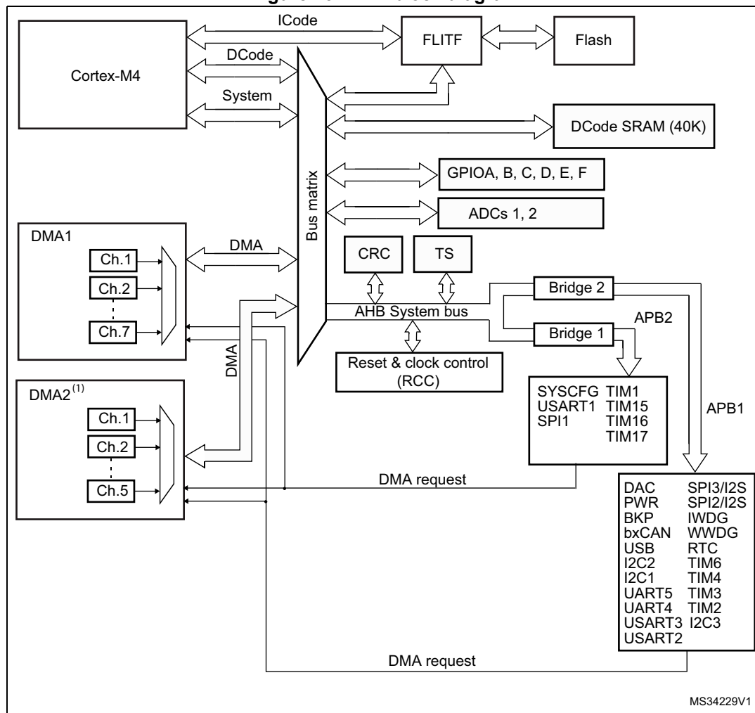
Figure 23. DMA block diagram
