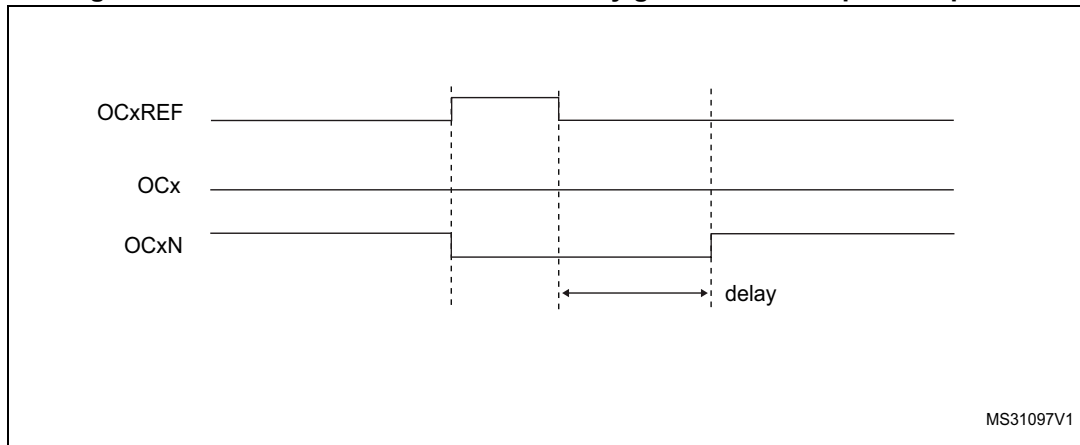
Figure 262. Dead-time waveforms with delay greater than the positive pulse.
