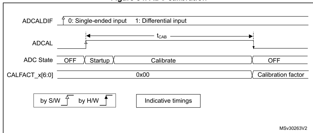
Figure 54. ADC calibration
