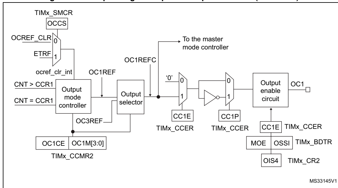
Figure 216. Output stage of capture/compare channel (channel 1)
