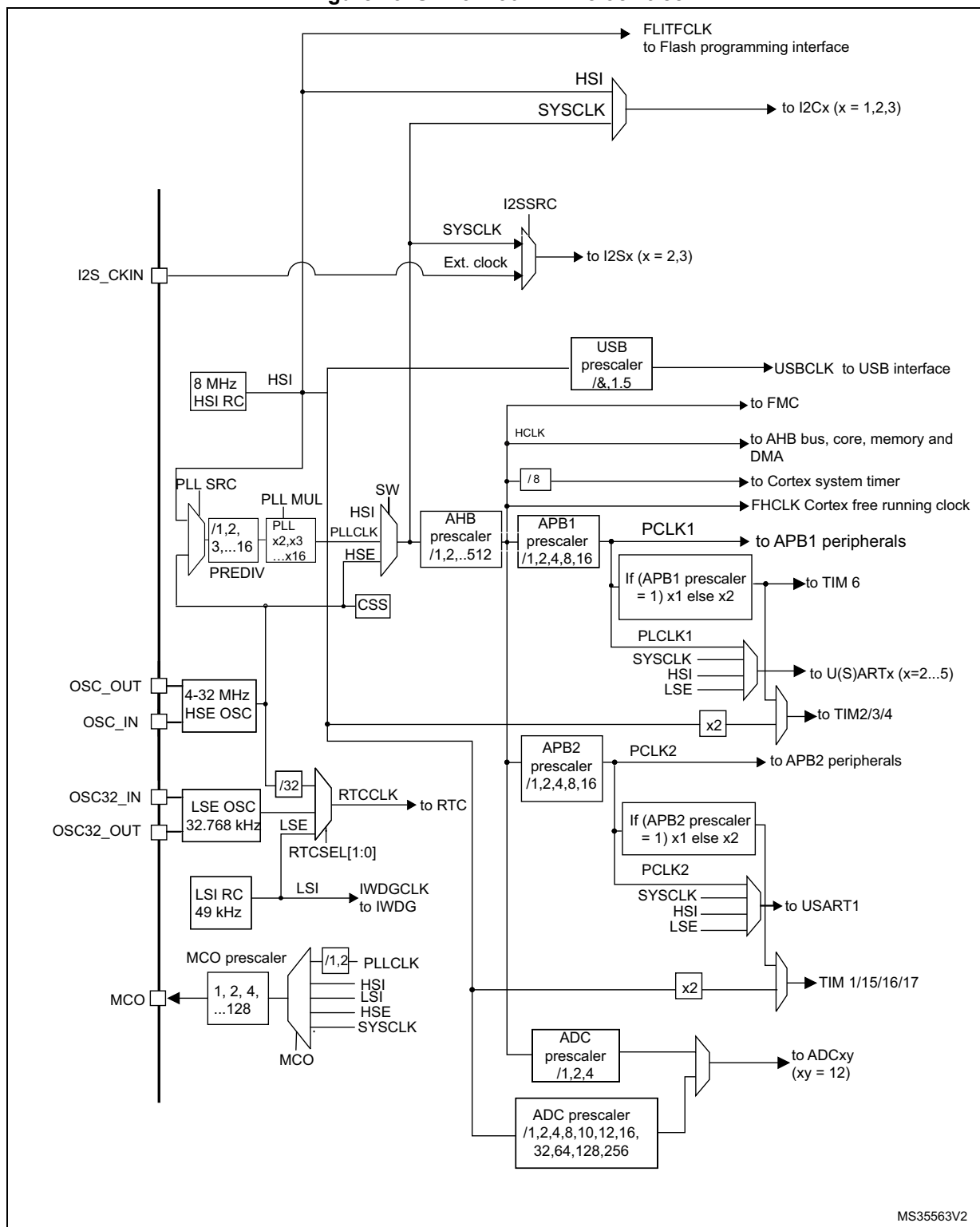
Figure 13. STM32F302xD/E clock tree
