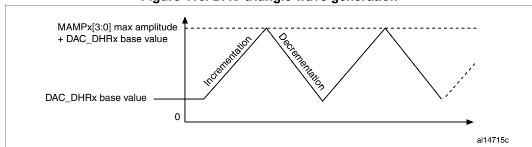
Figure 117. DAC conversion (SW trigger enabled) with triangle wave generation
