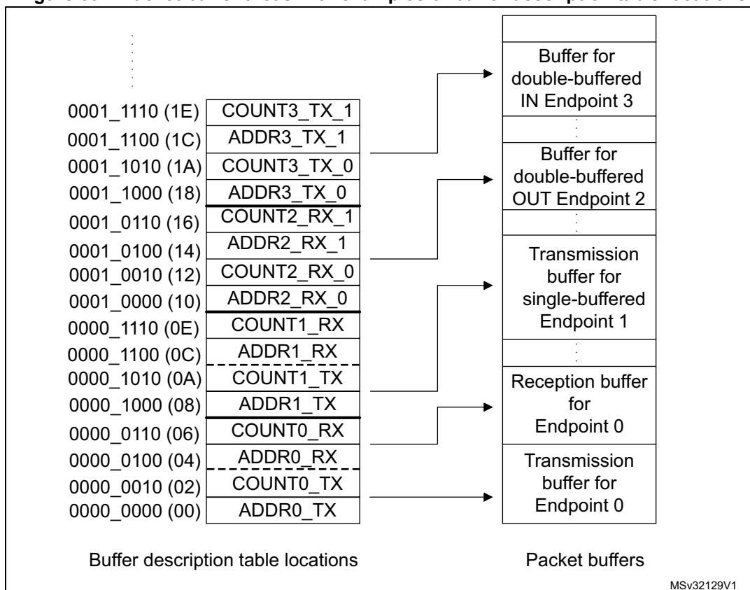
Figure 394. Packet buffer areas with examples of buffer description table locations
