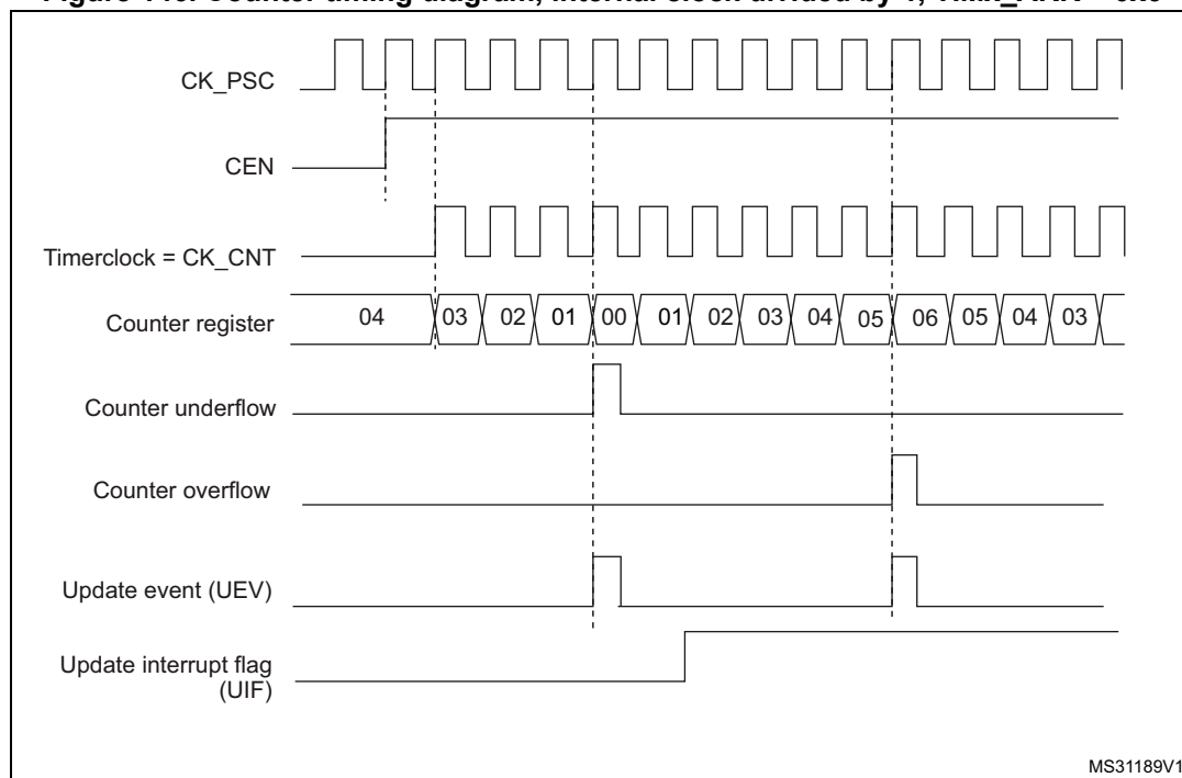
Figure 146. Counter timing diagram, internal clock divided by 1, TIMx_ARR = 0x6
