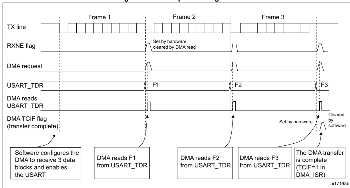
Figure 294. Reception using DMA
