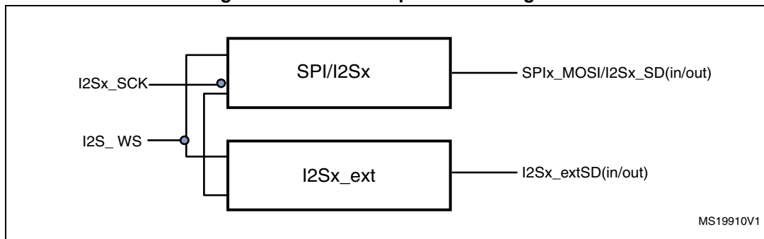
Figure 316. I2S full duplex block diagram
