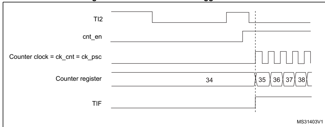
Figure 227. Control circuit in trigger mode
