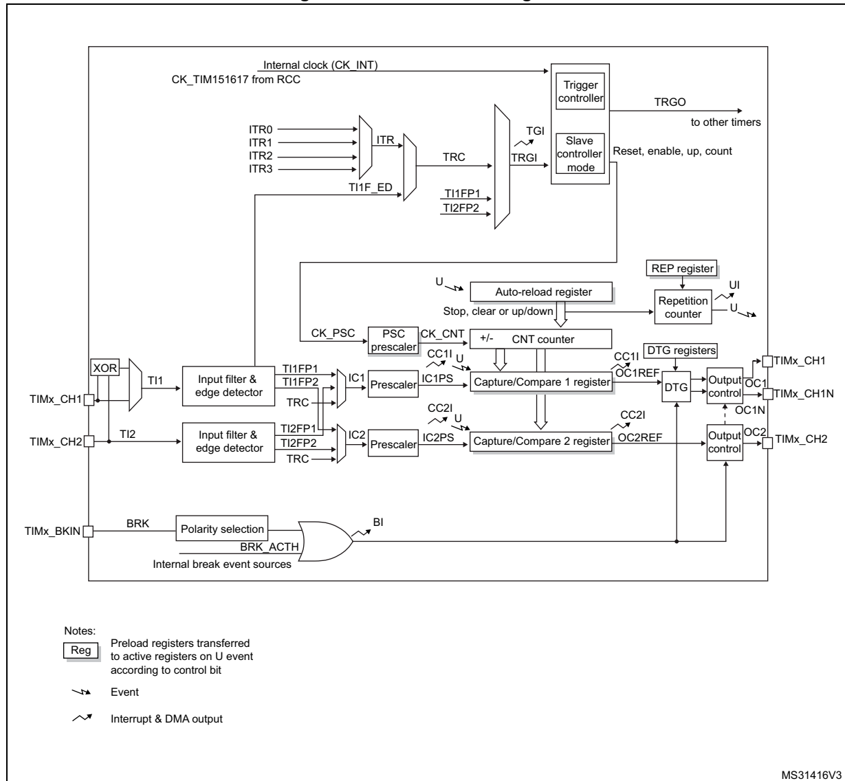
Figure 197. TIM15 block diagram
