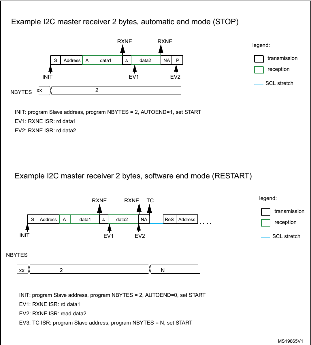
Figure 265. Transfer bus diagrams for I2C master receiver
