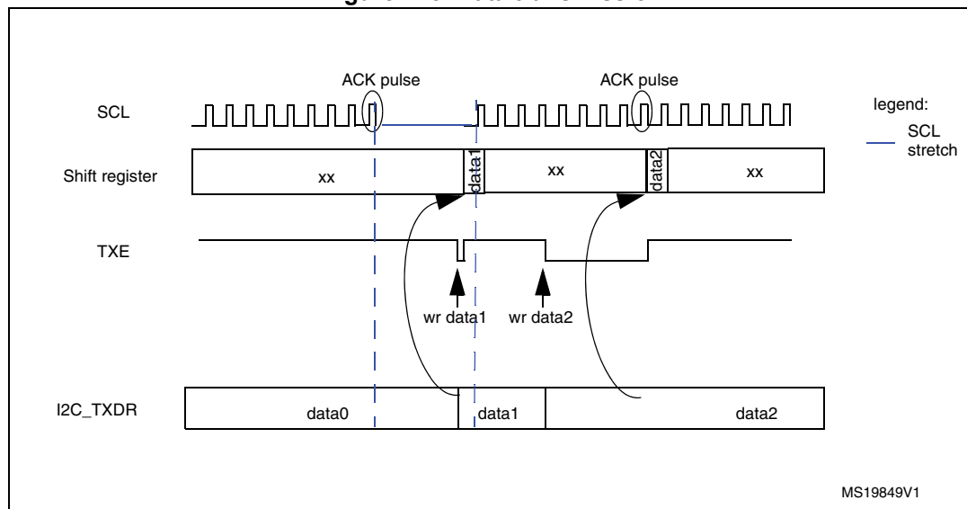
Figure 248. Data transmission
