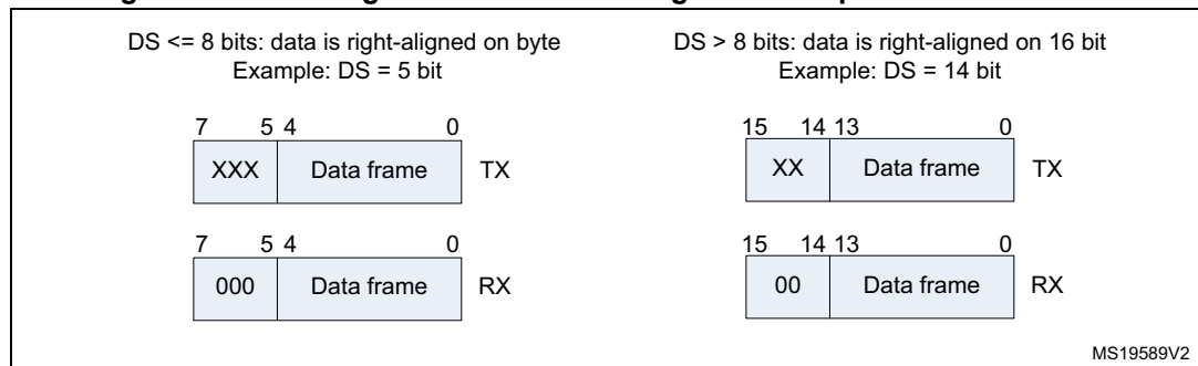
Figure 307. Data alignment when data length is not equal to 8-bit or 16-bit
