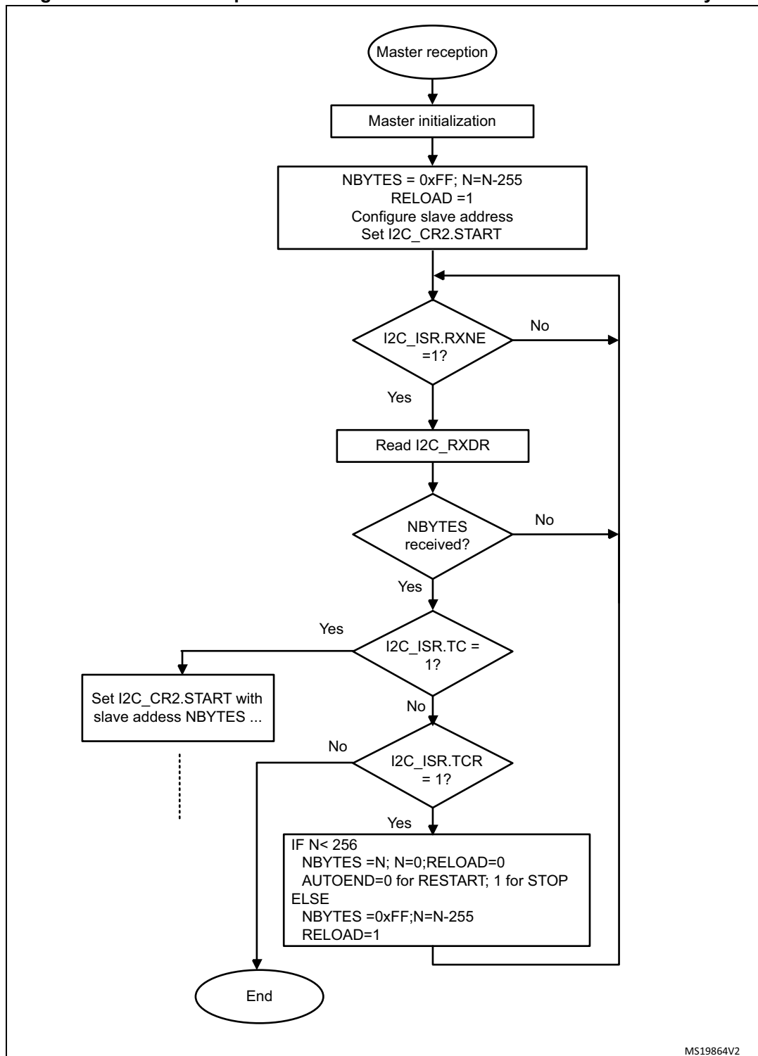
Figure 264. Transfer sequence flowchart for I2C master receiver for N &gt; 255 bytes
