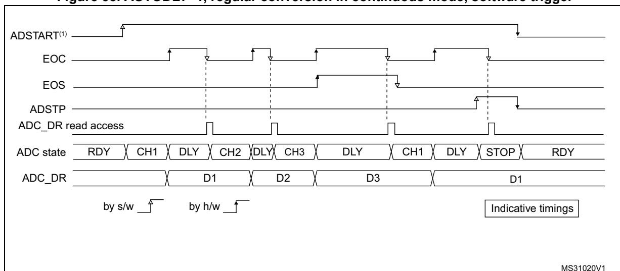
Figure 58. AUTDLY=1, regular conversion in continuous mode, software trigger
