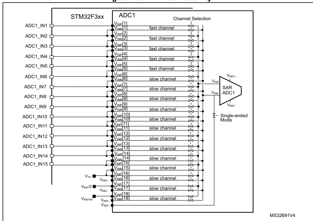
Figure 26. ADC1 connectivity
