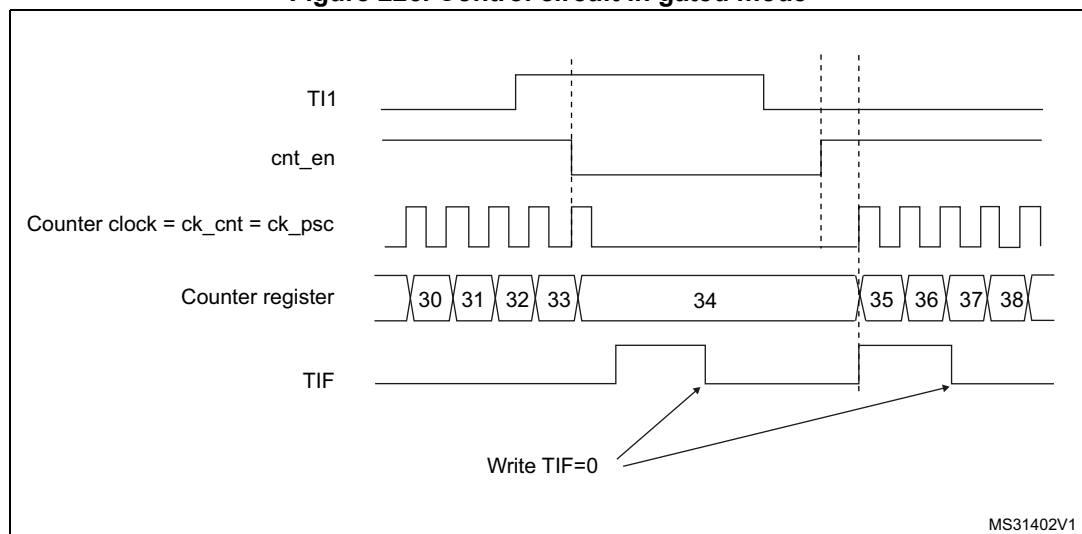
Figure 226. Control circuit in gated mode
