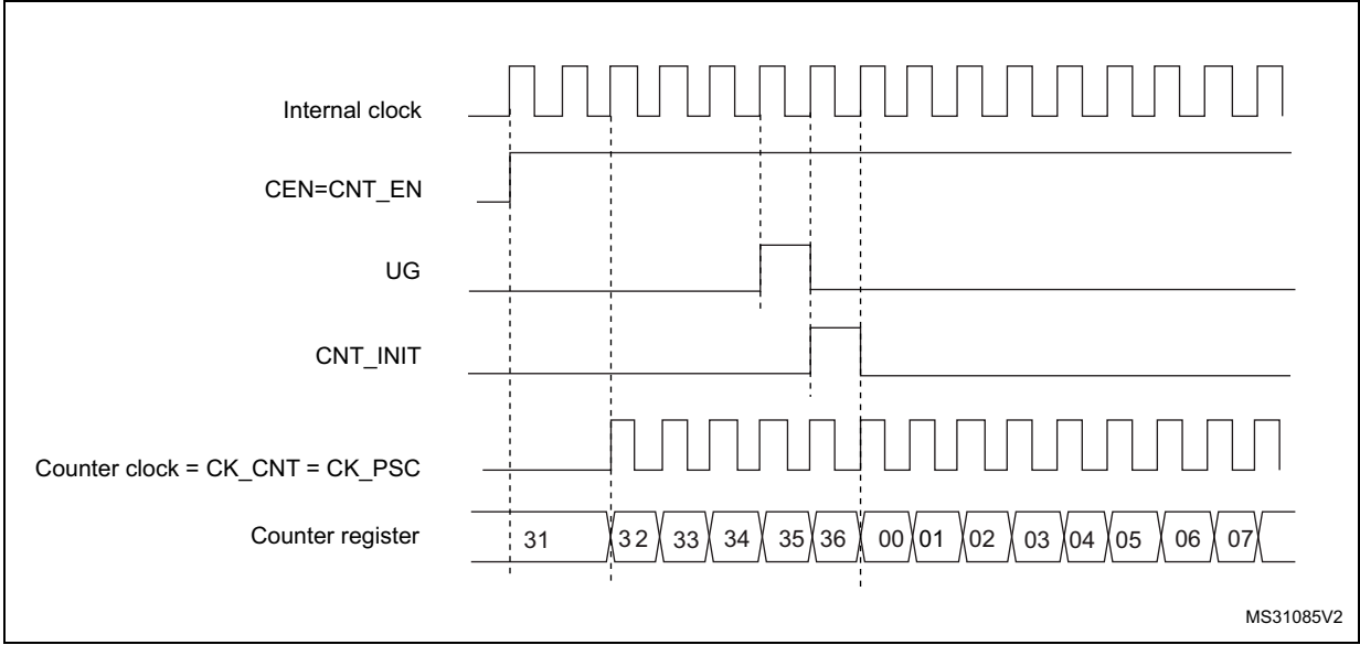
Figure 237. Control circuit in normal mode, internal clock divided by 1
