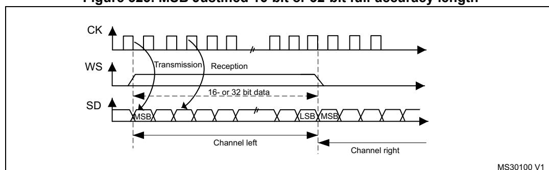
Figure 323. MSB Justified 16-bit or 32-bit full-accuracy length
