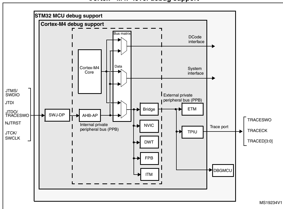
Figure 337. Block diagram of STM32 MCU and Cortex®-M4F-level debug support
