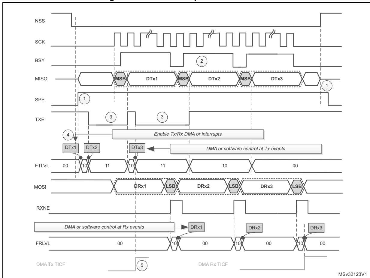
Figure 310. Slave full duplex communication
