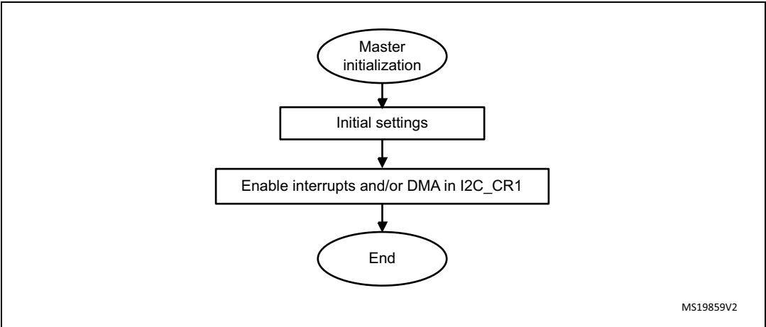
Figure 257. Master initialization flowchart
