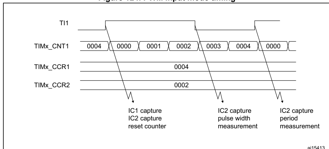
Figure 124. PWM input mode timing
