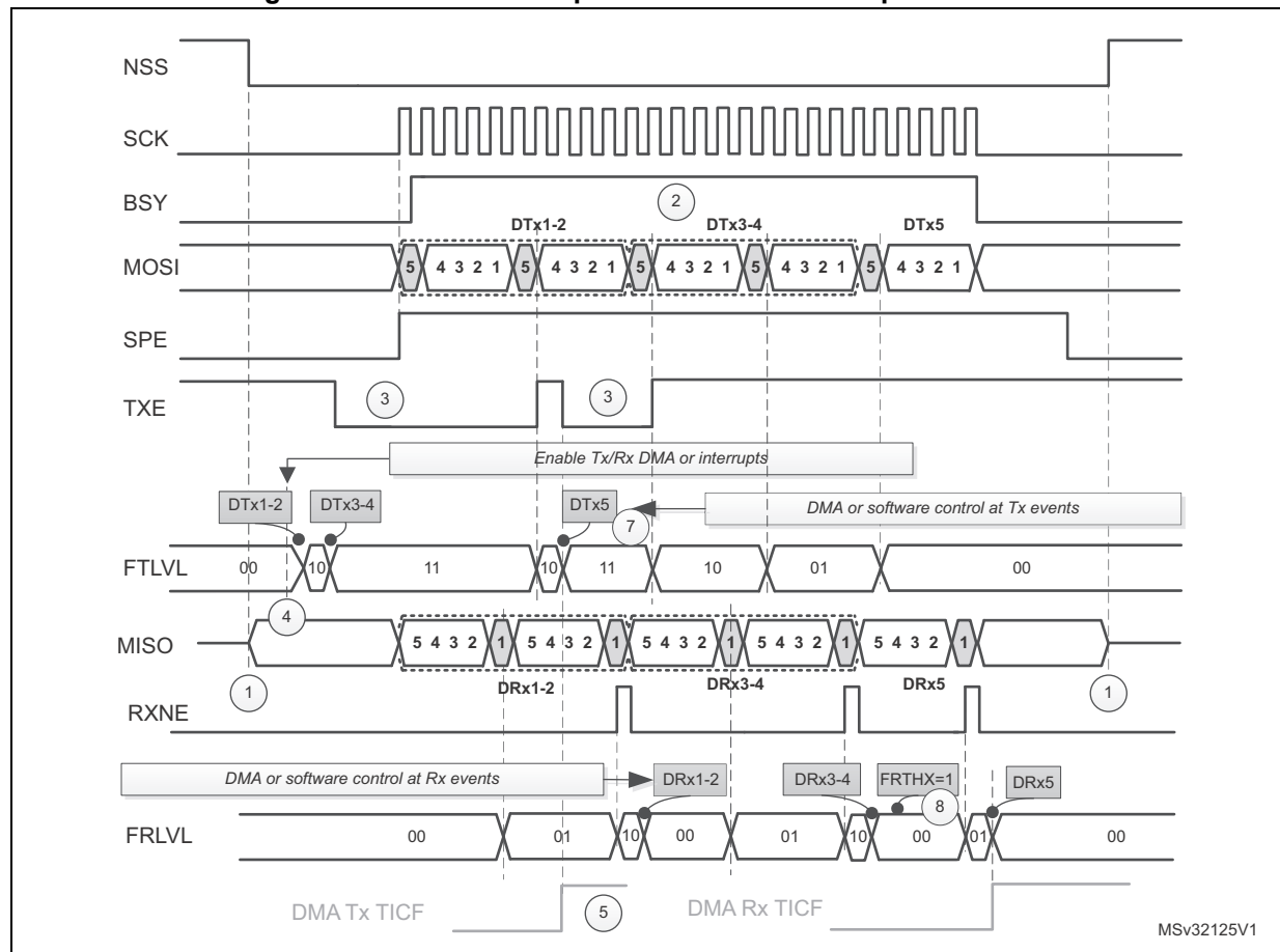
Figure 312. Master full duplex communication in packed mode
