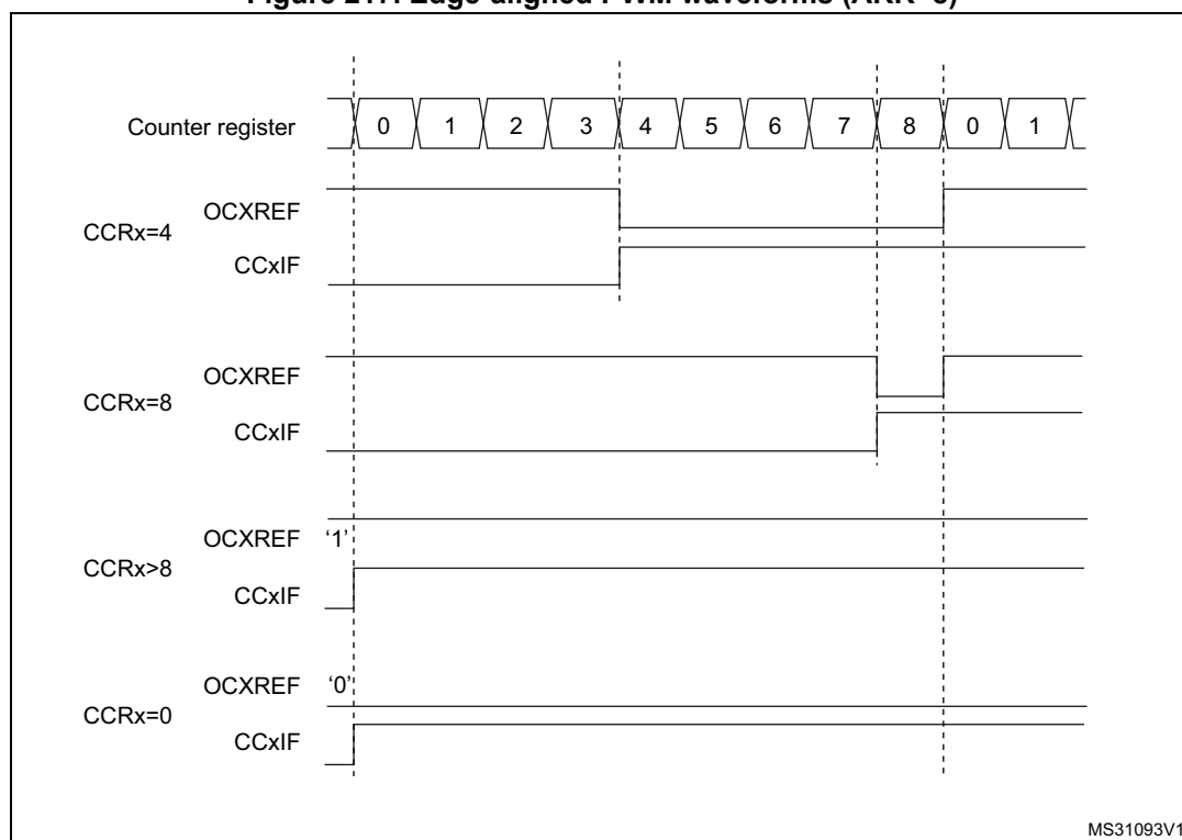
Figure 217. Edge-aligned PWM waveforms (ARR=8)
