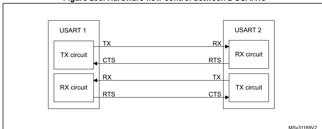
Figure 295. Hardware flow control between 2 USARTs
