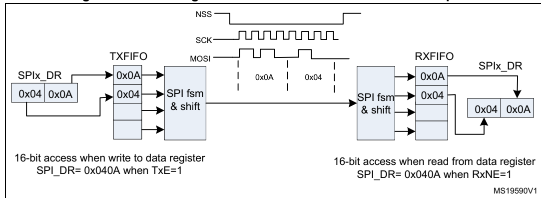
Figure 308. Packing data in FIFO for transmission and reception
