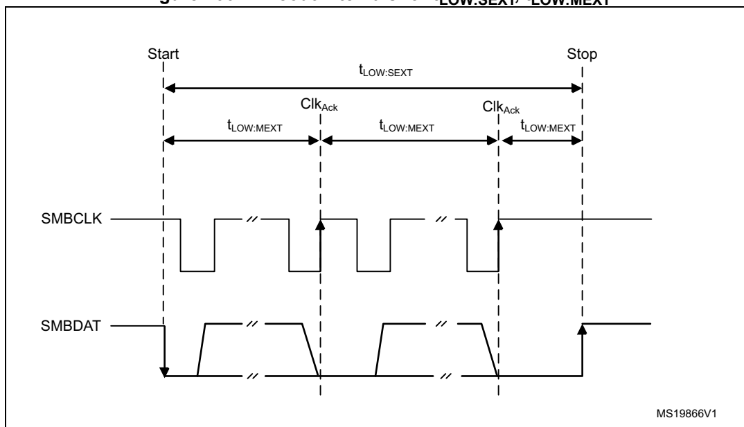
Figure 266. Timeout intervals for t_{\text{LOW:SEXT}} , t_{\text{LOW:MEXT}}
