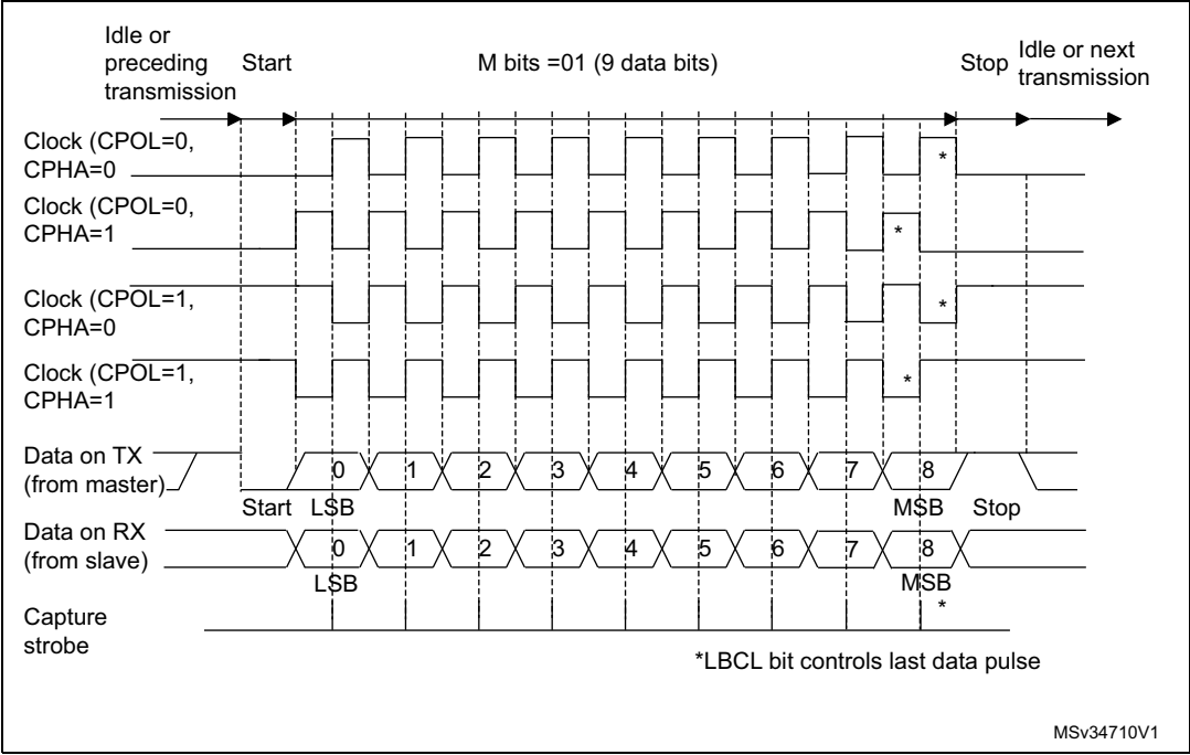
Figure 287. USART data clock timing diagram (M bits = 01)
