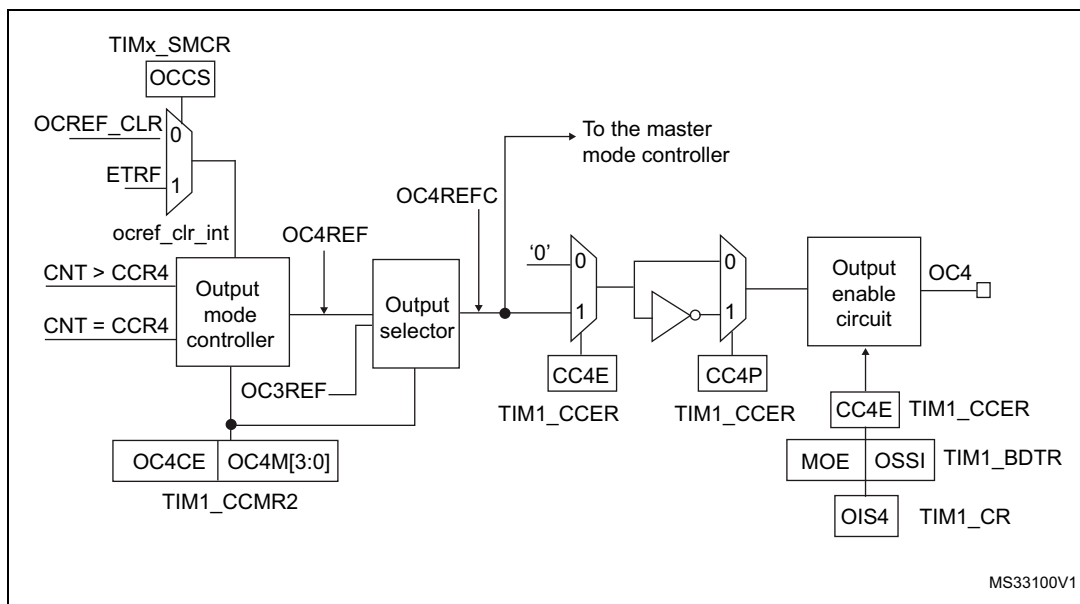
Figure 122. Output stage of capture/compare channel (channel 4)
