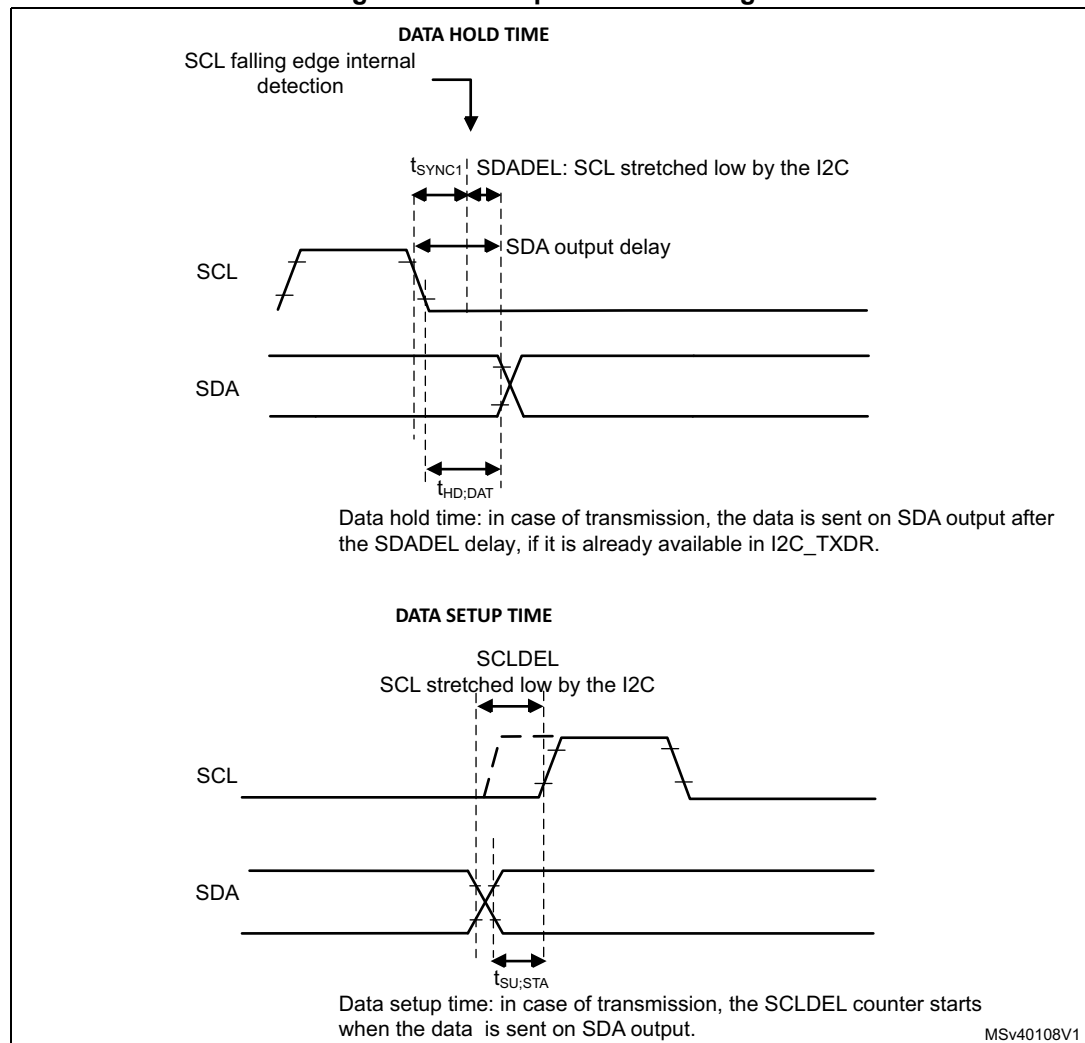
Figure 245. Setup and hold timings
