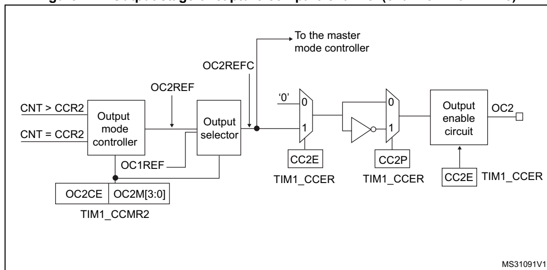
Figure 214. Output stage of capture/compare channel (channel 2 for TIM15)
