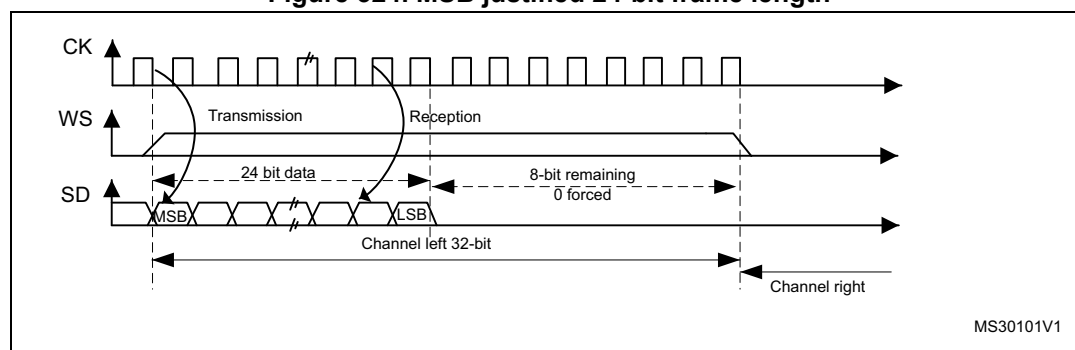
Figure 324. MSB justified 24-bit frame length
