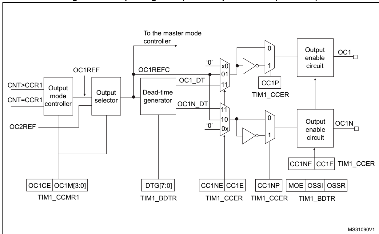
Figure 213. Output stage of capture/compare channel (channel 1)
