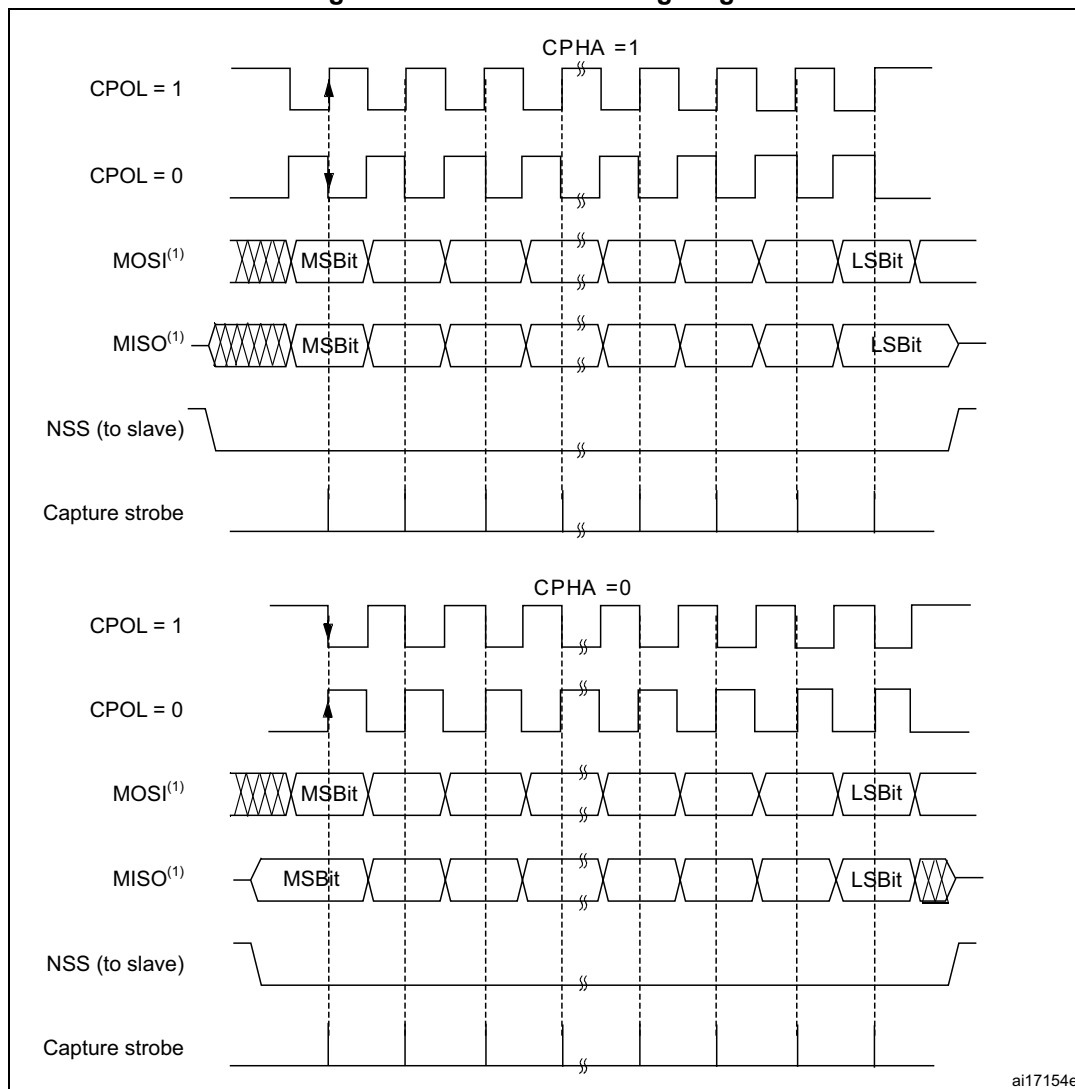
Figure 306. Data clock timing diagram
