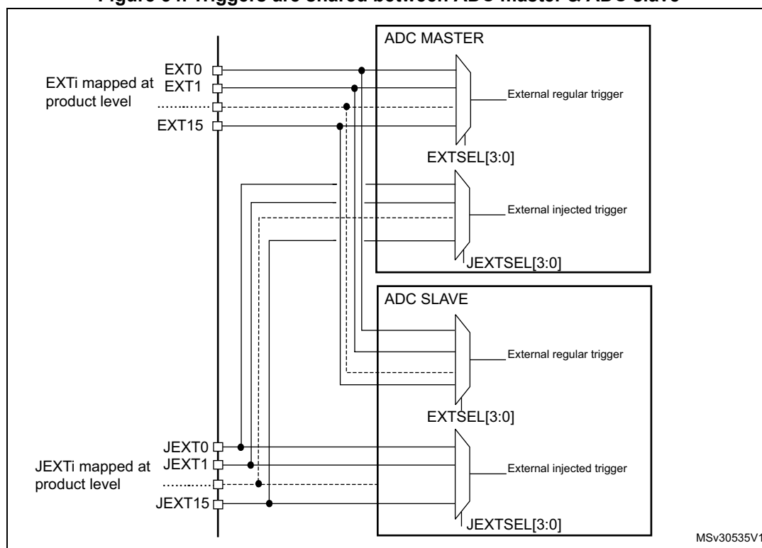
Figure 34. Triggers are shared between ADC master &amp; ADC slave
