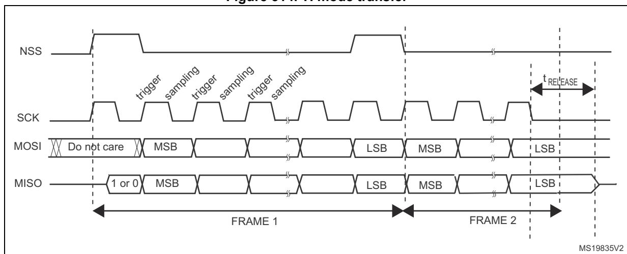
Figure 314. TI mode transfer
