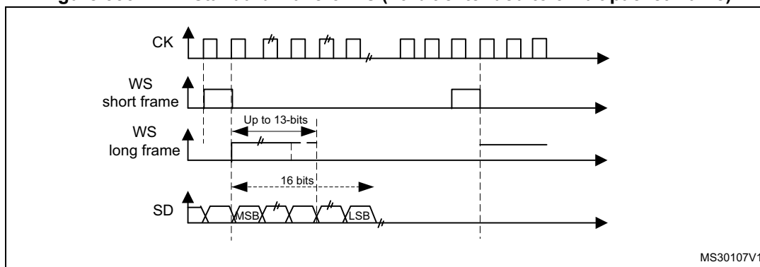
Figure 333. PCM standard waveforms (16-bit extended to 32-bit packet frame)
