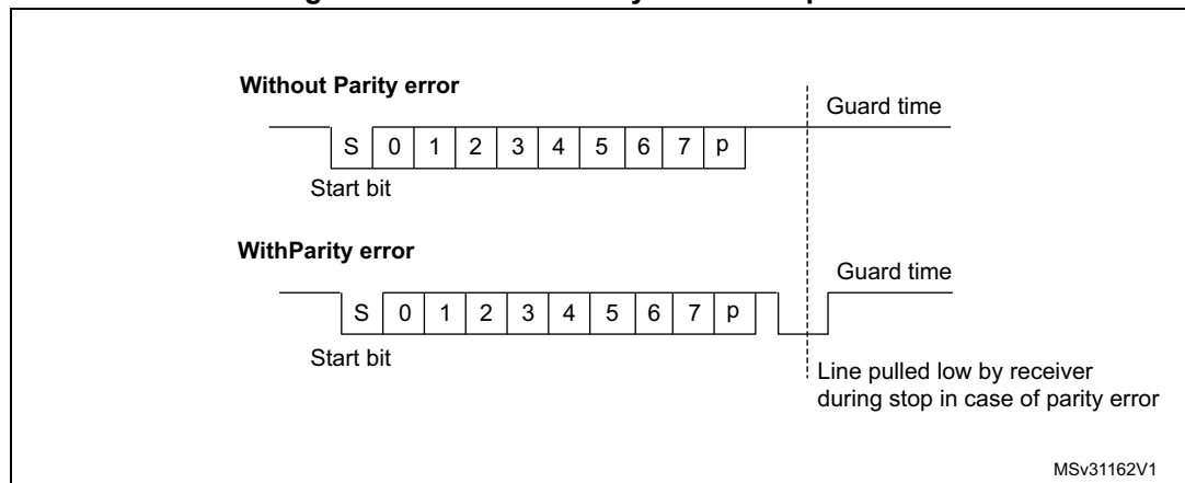
Figure 289. ISO 7816-3 asynchronous protocol
