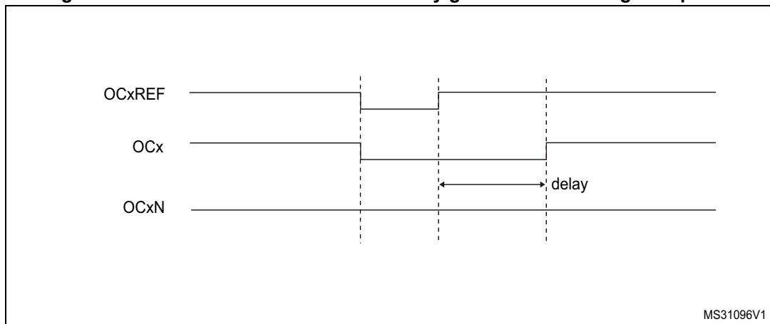
Figure 221. Dead-time waveforms with delay greater than the positive pulse.
