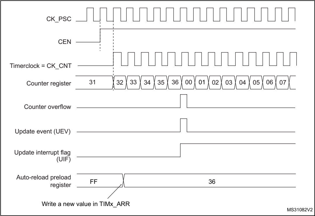
Figure 205. Counter timing diagram, update event when ARPE=0 (TIMx_ARR not preloaded)
