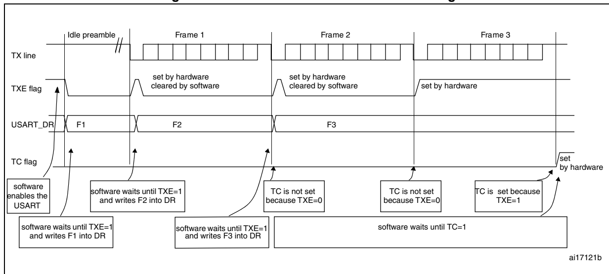
Figure 277. TC/TXE behavior when transmitting
