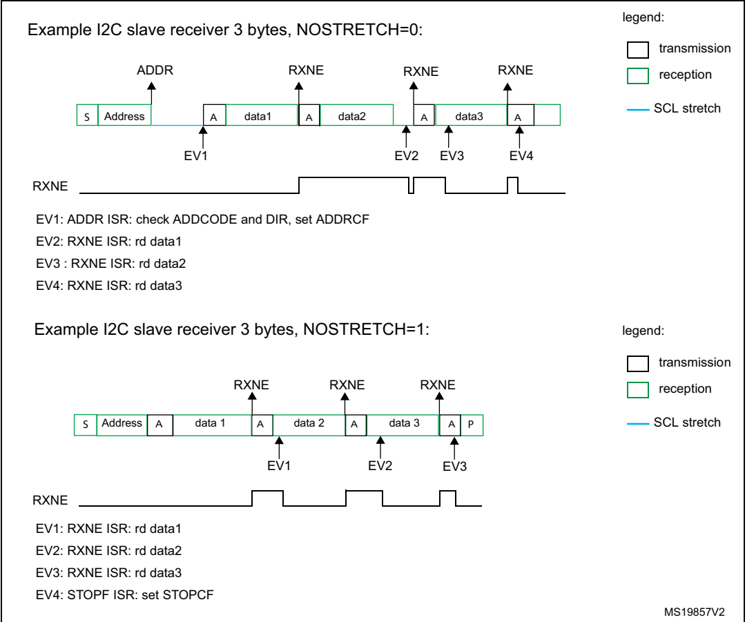
Figure 255. Transfer bus diagrams for I2C slave receiver
