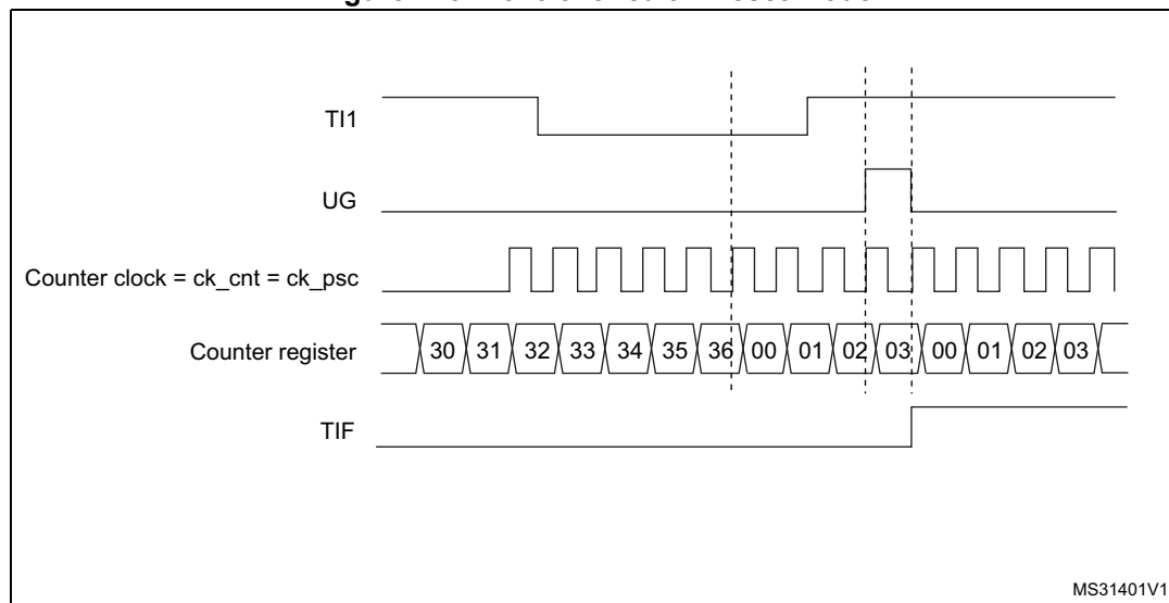
Figure 225. Control circuit in reset mode
