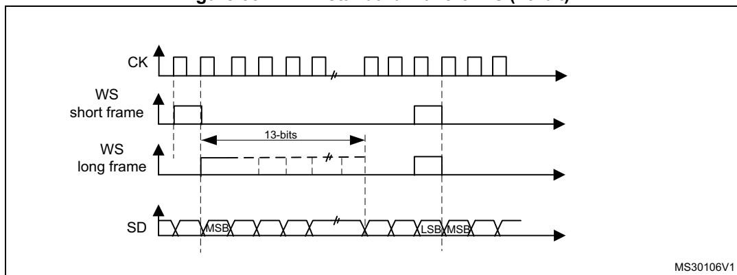
Figure 332. PCM standard waveforms (16-bit)
