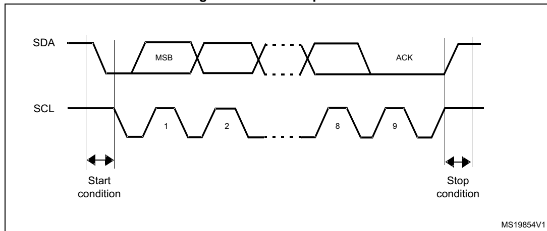
Figure 244. I 2 C bus protocol
