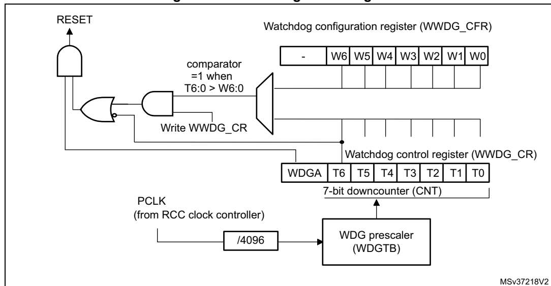
Figure 239. Watchdog block diagram
