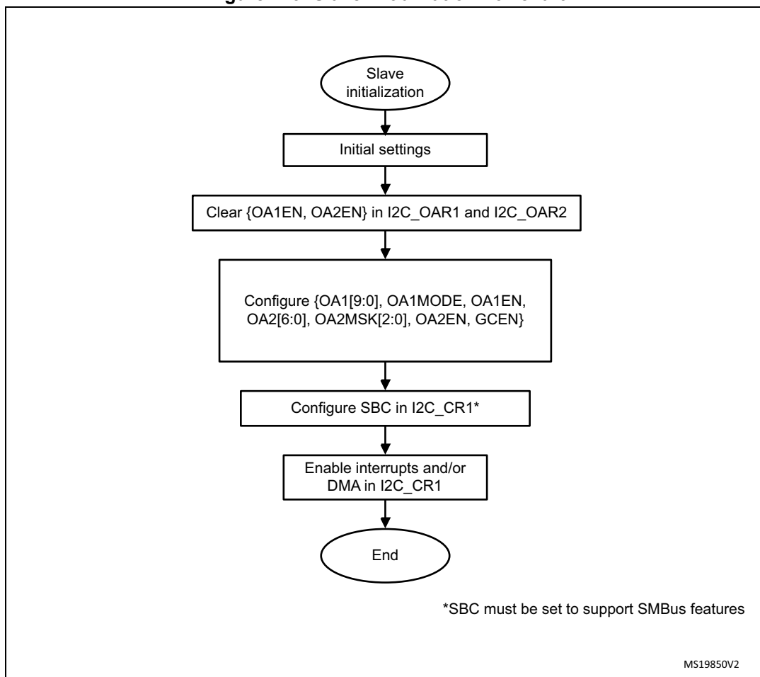
Figure 249. Slave initialization flowchart
