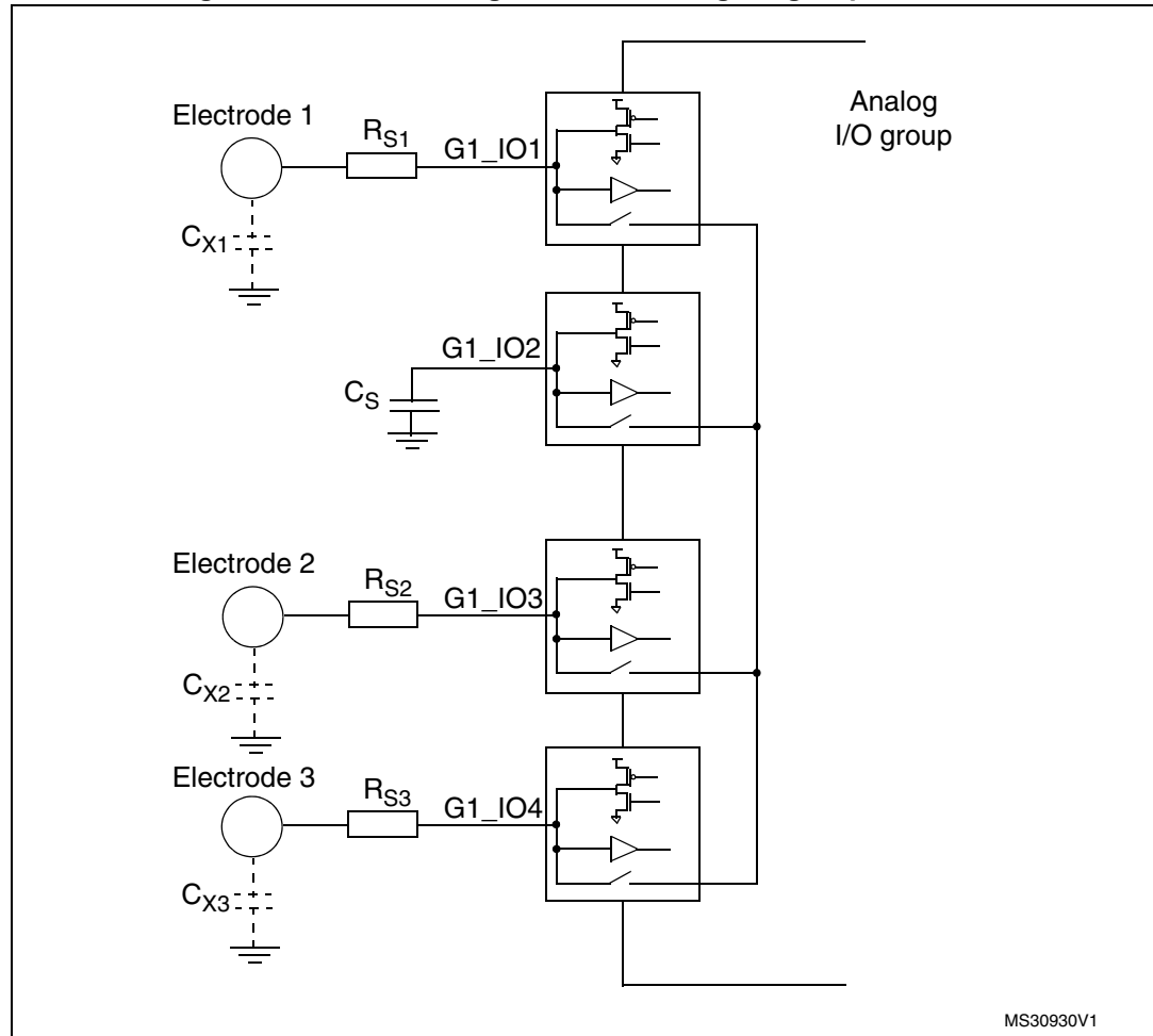
Figure 88. Surface charge transfer analog I/O group structure
