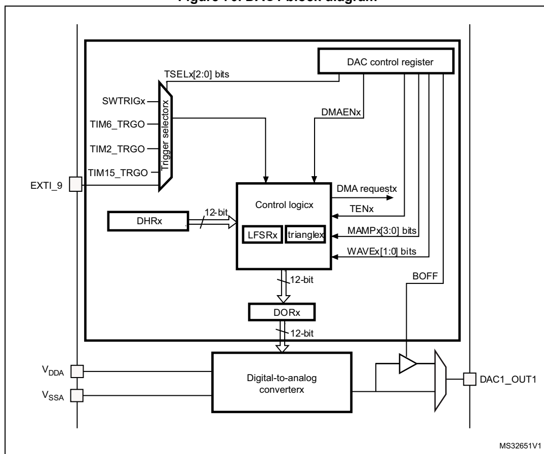
Figure 70. DAC1 block diagram
