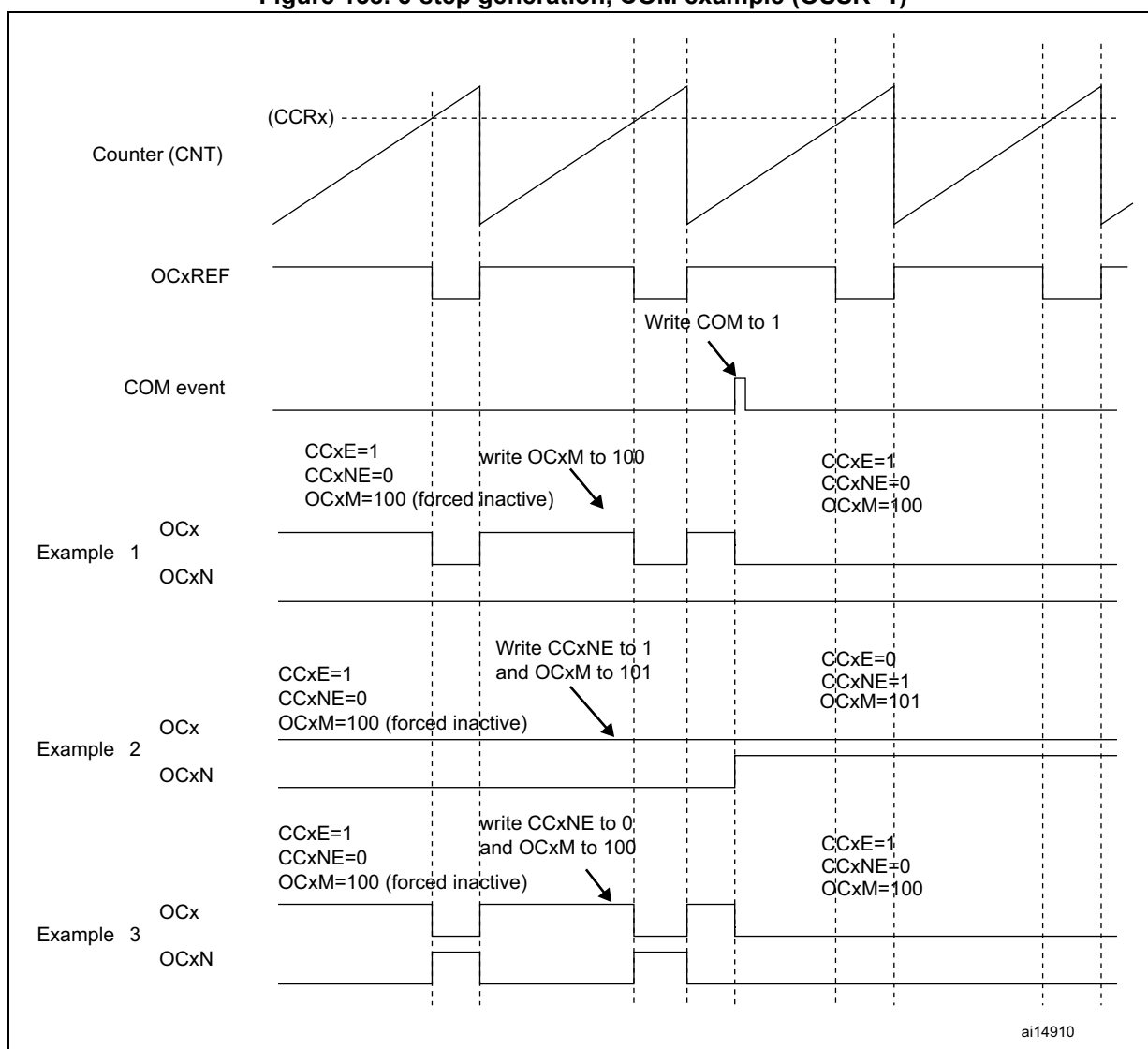
Figure 138. 6-step generation, COM example (OSSR=1)
