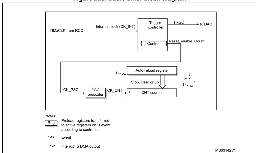
Figure 228. Basic timer block diagram
