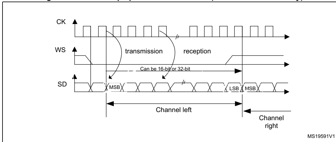
Figure 317. I 2 S Philips protocol waveforms (16/32-bit full accuracy)
