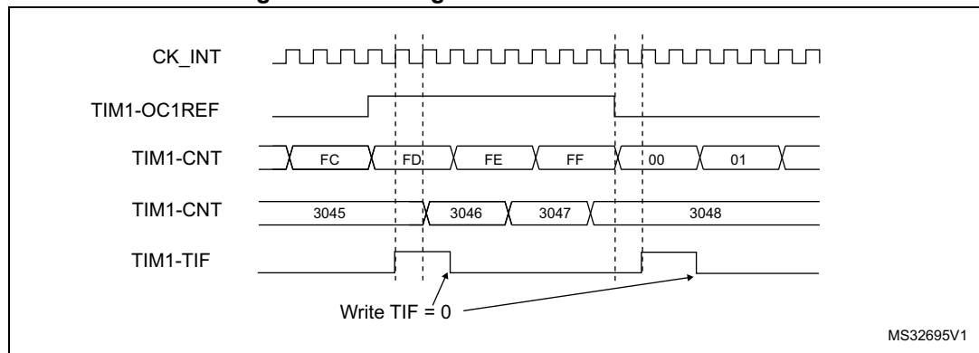
Figure 193. Gating TIM2 with OC1REF of TIM1
