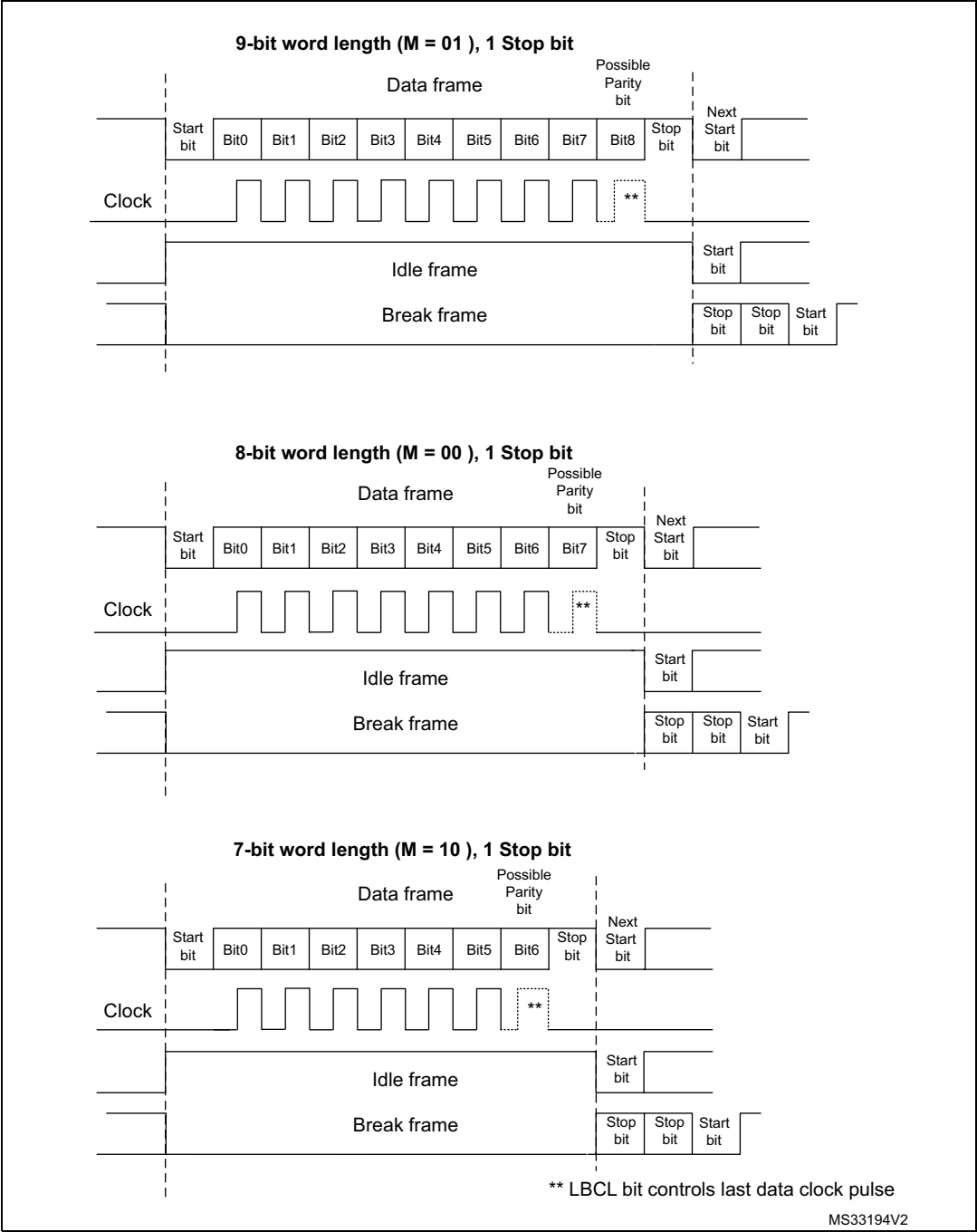
Figure 275. Word length programming
