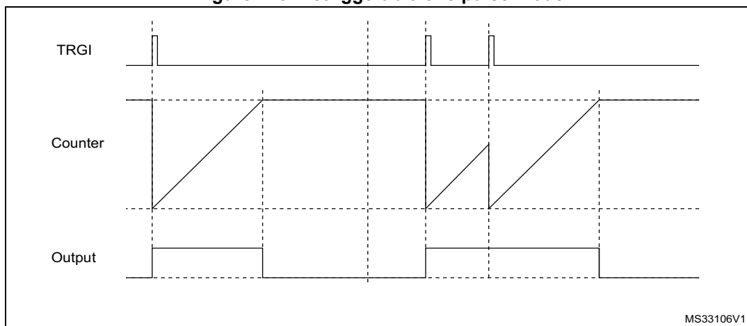
Figure 140. Retriggerable one pulse mode
