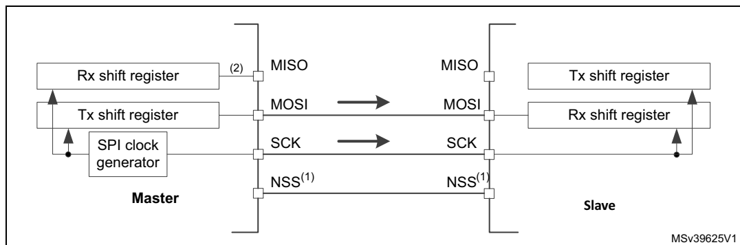
Figure 302. Simplex single master/single slave application (master in transmit-only/ slave in receive-only mode)
