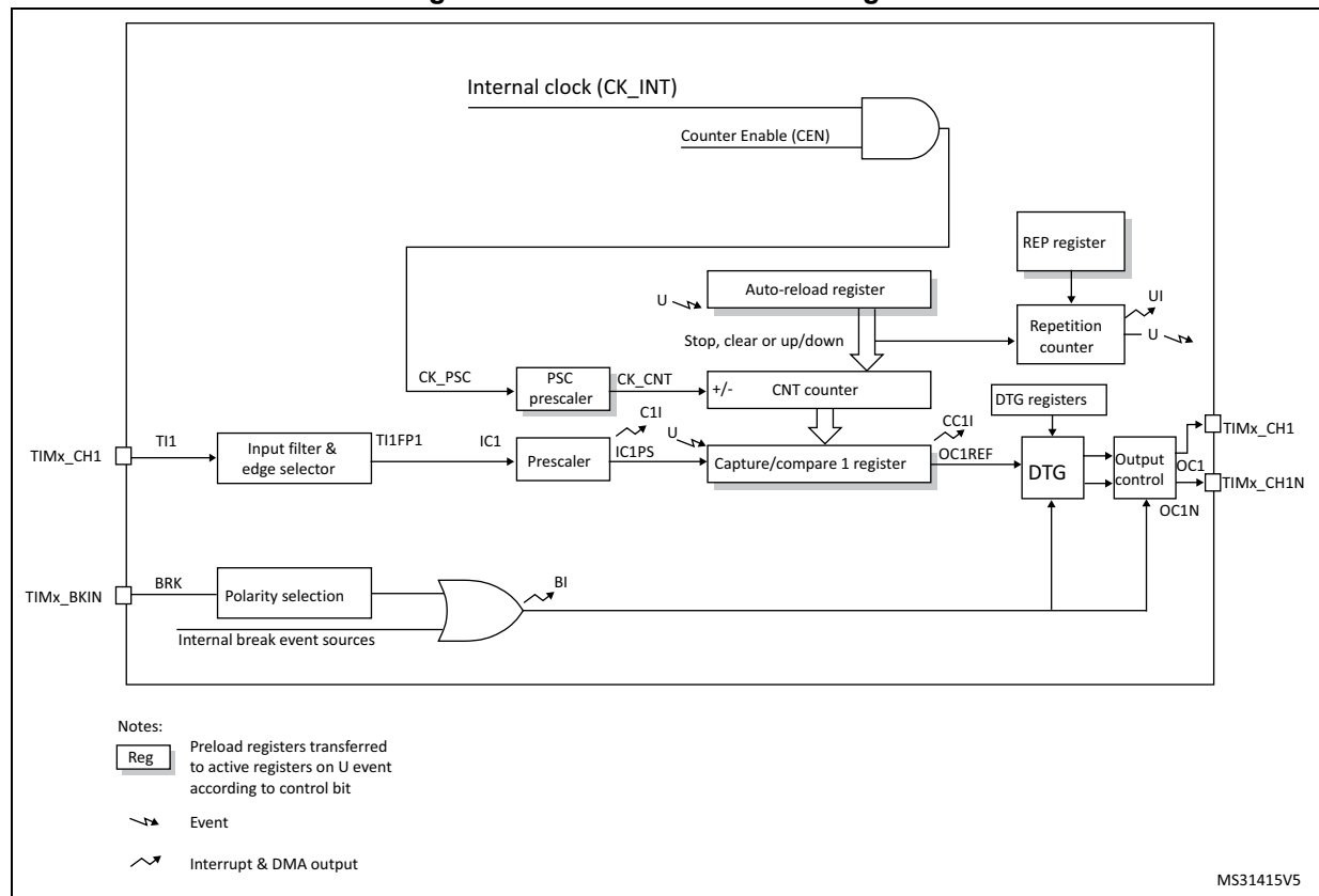
Figure 198. TIM16/TIM17 block diagram
