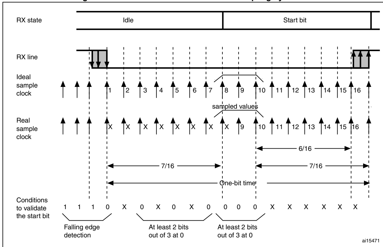
Figure 278. Start bit detection when oversampling by 16 or 8
