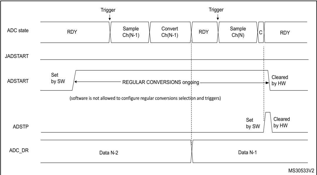
Figure 32. Stopping ongoing regular conversions
