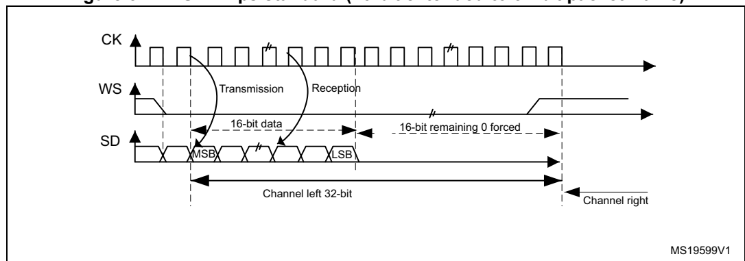
Figure 321. I 2 S Philips standard (16-bit extended to 32-bit packet frame)
