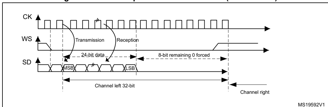
Figure 318. I 2 S Philips standard waveforms (24-bit frame)
