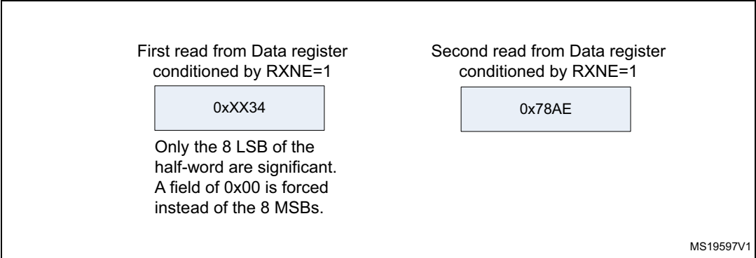
Figure 329. Operations required to receive 0x3478AE
