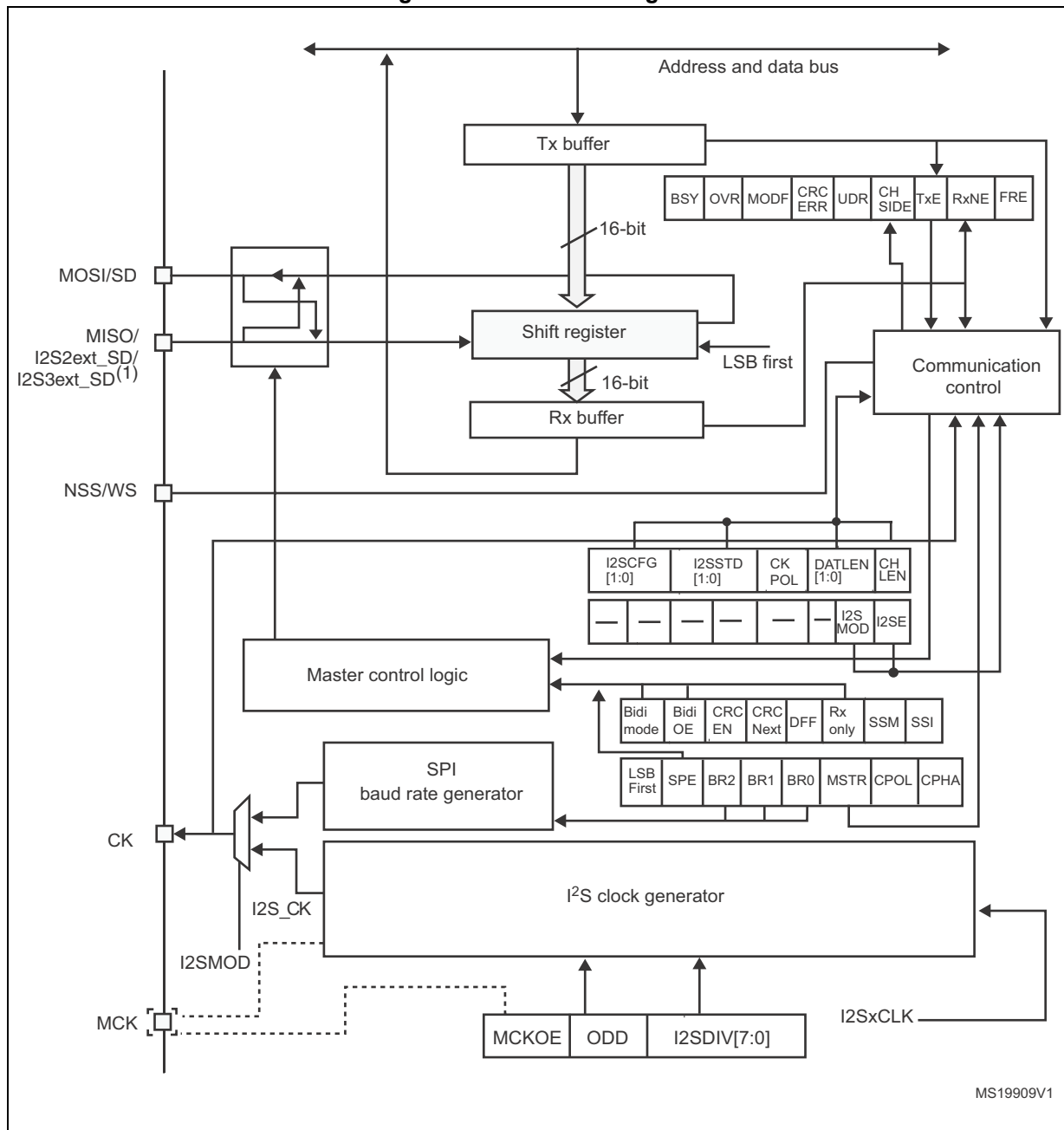
Figure 315. I 2 S block diagram
