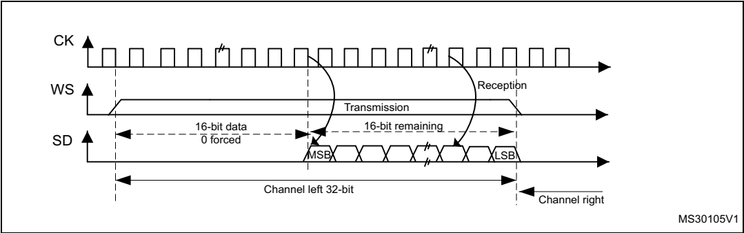
Figure 330. LSB justified 16-bit extended to 32-bit packet frame
