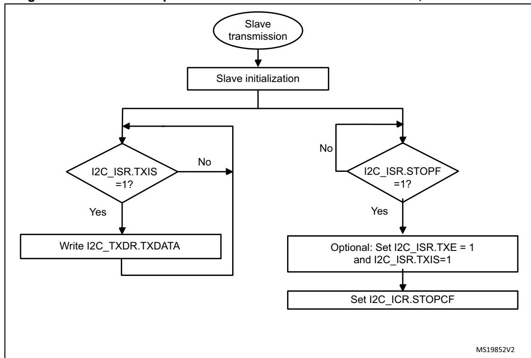
Figure 251. Transfer sequence flowchart for I2C slave transmitter, NOSTRETCH=1
