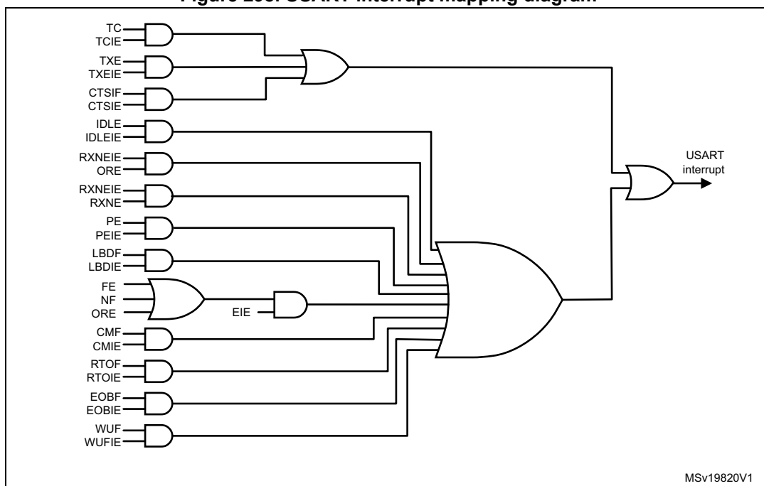
Figure 298. USART interrupt mapping diagram
