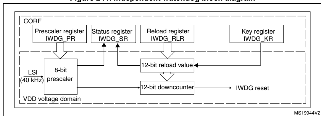
Figure 241. Independent watchdog block diagram
