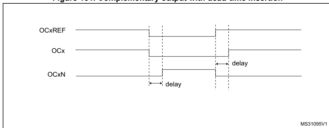
Figure 131. Complementary output with dead-time insertion
