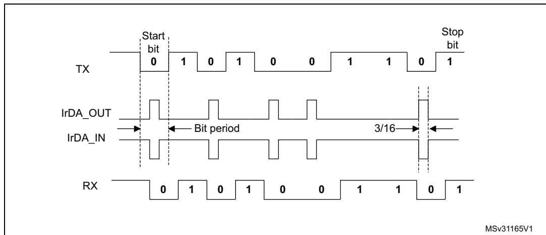
Figure 292. IrDA data modulation (3/16) -Normal Mode
