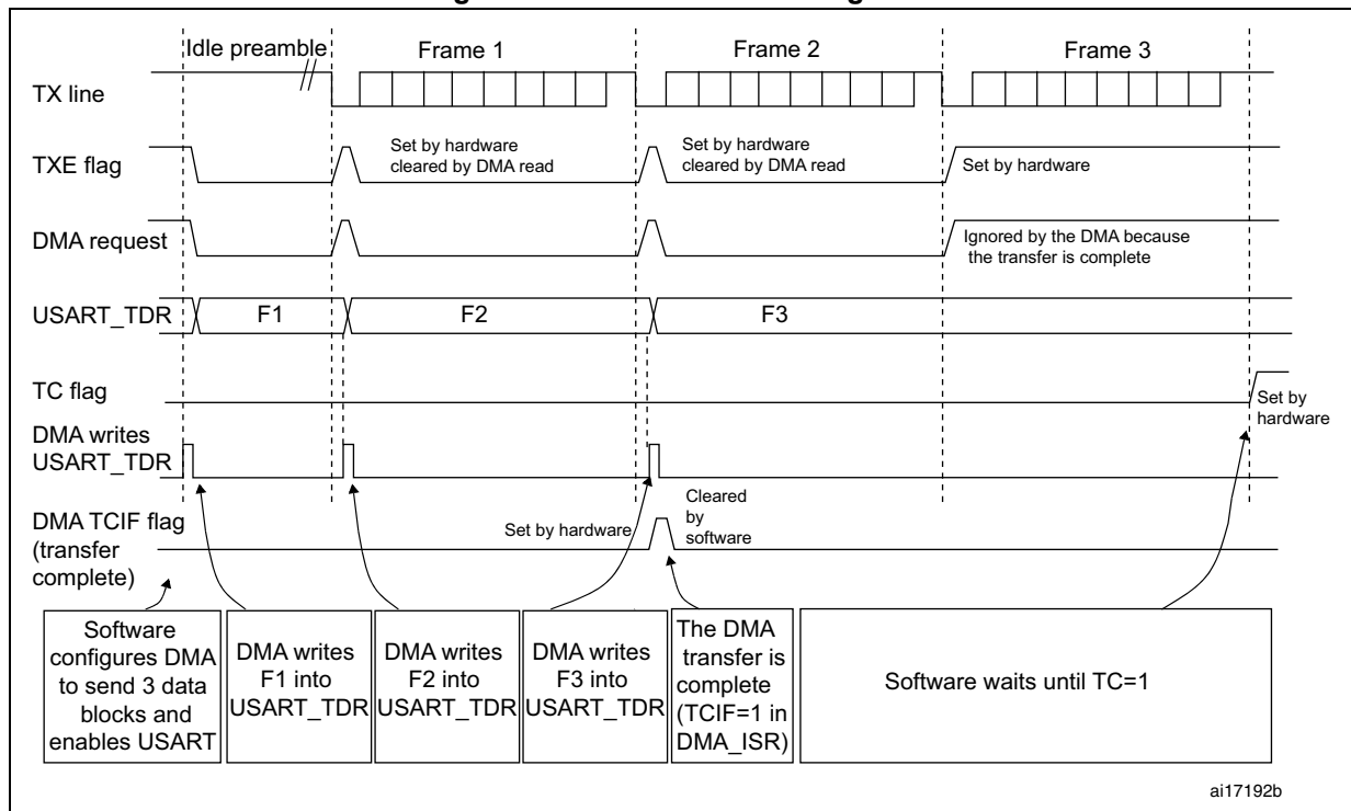
Figure 293. Transmission using DMA
