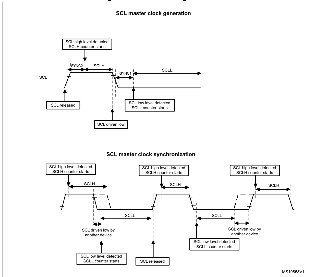
Figure 256. Master clock generation
