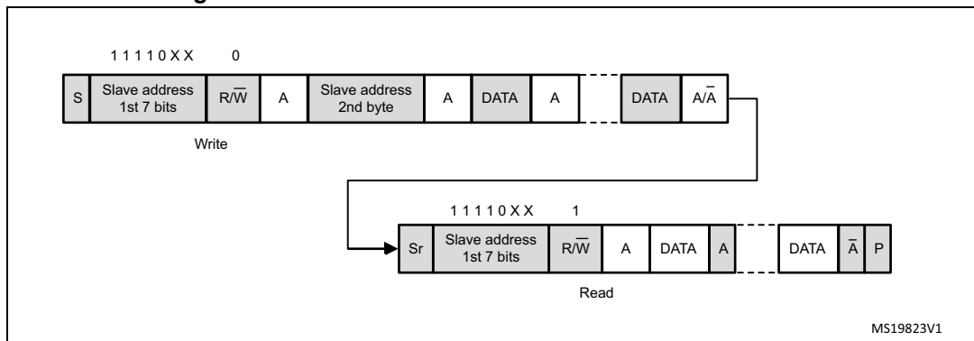
Figure 259. 10-bit address read access with HEAD10R=1
