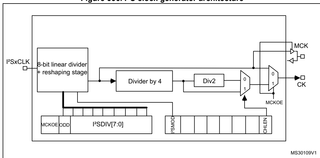
Figure 336. I 2 S clock generator architecture
