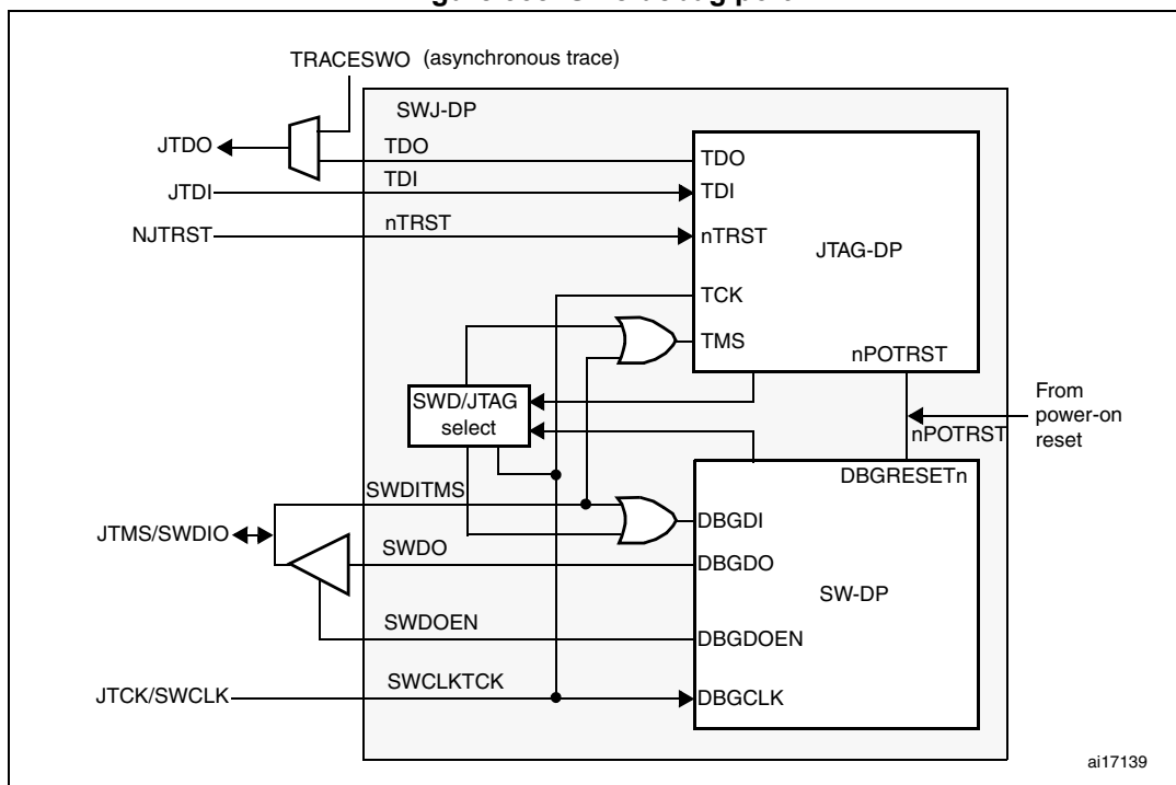
Figure 338. SWJ debug port
