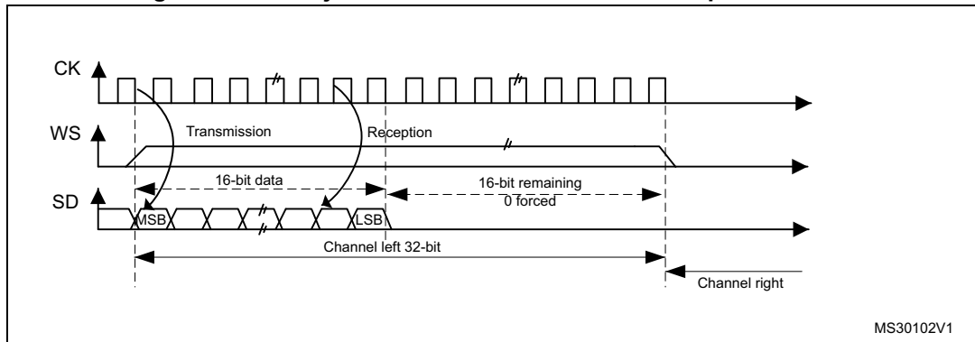
Figure 325. MSB justified 16-bit extended to 32-bit packet frame
