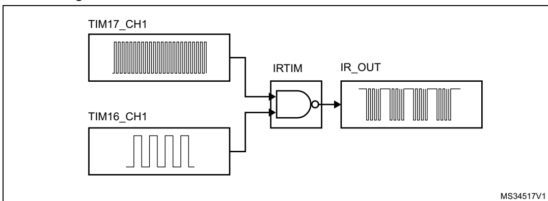
Figure 238. IR internal hardware connections with TIM16 and TIM17
