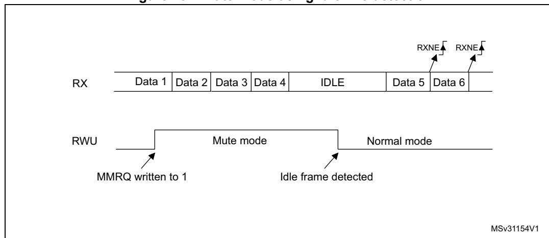
Figure 281. Mute mode using Idle line detection
