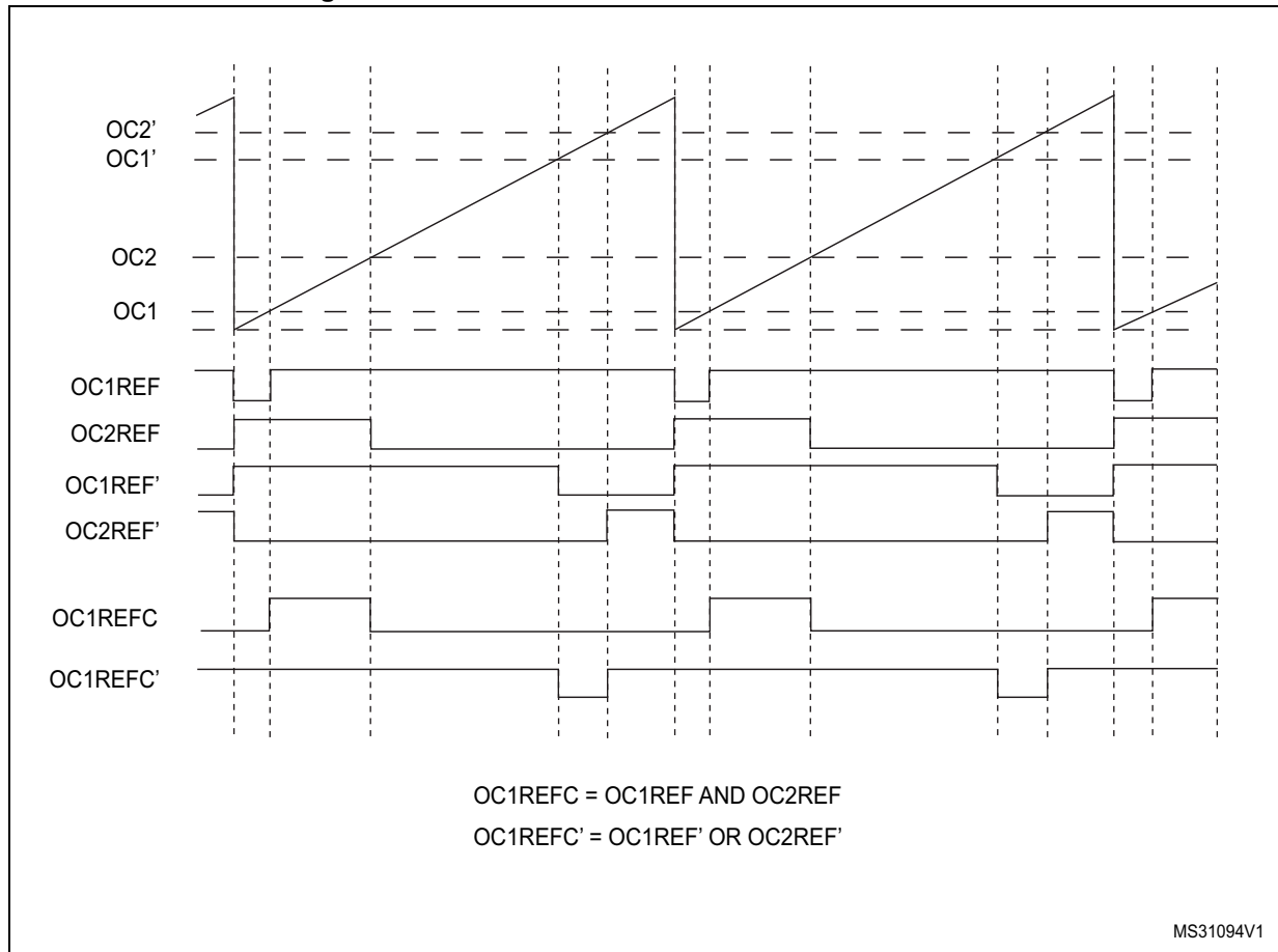
Figure 129. Combined PWM mode on channel 1 and 3
