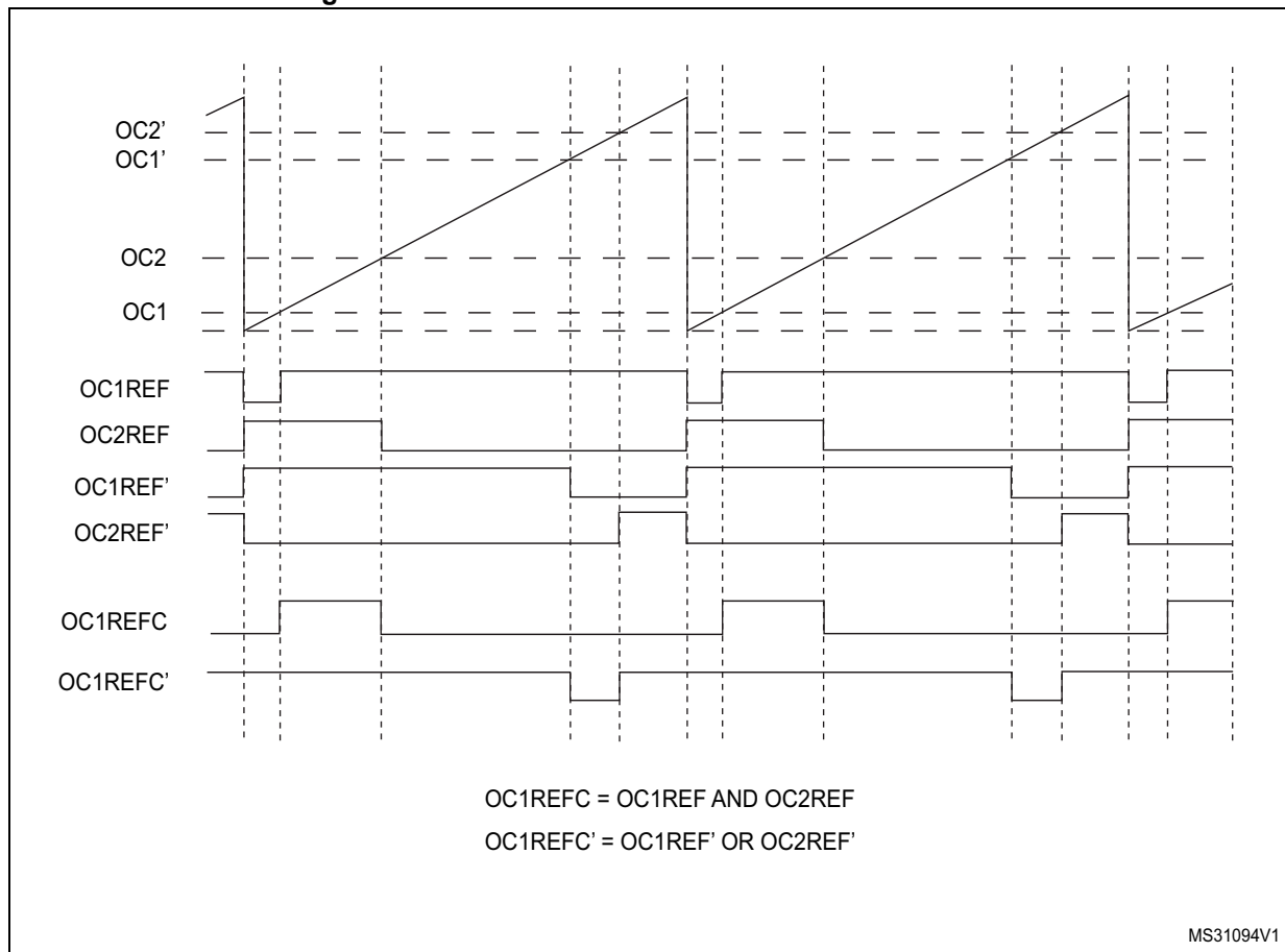
Figure 218. Combined PWM mode on channel 1 and 2
