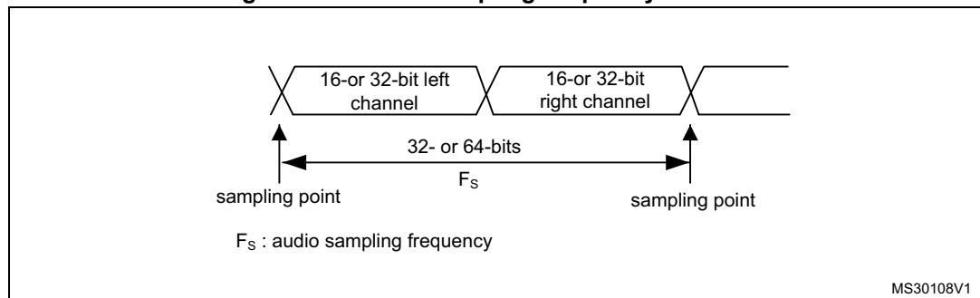
Figure 335. Audio sampling frequency definition
