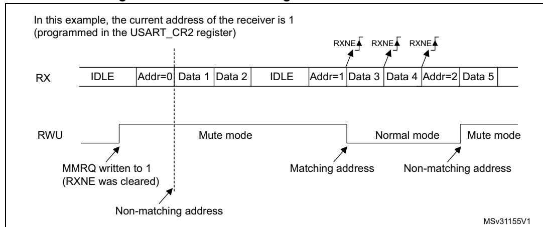
Figure 282. Mute mode using address mark detection
