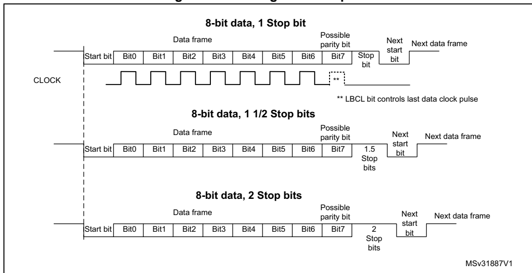
Figure 276. Configurable stop bits
