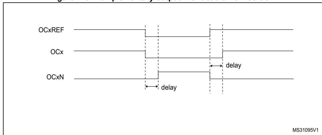
Figure 219. Complementary output with dead-time insertion.
