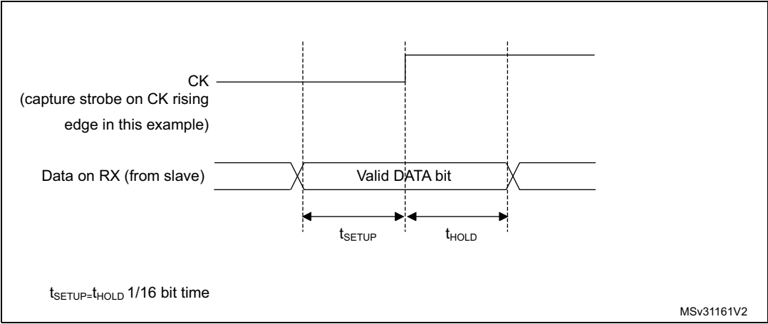
Figure 288. RX data setup/hold time
