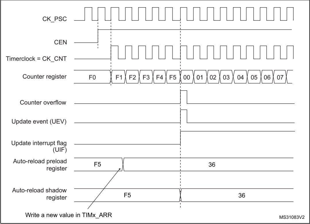
Figure 206. Counter timing diagram, update event when ARPE=1 (TIMx_ARR preloaded)
