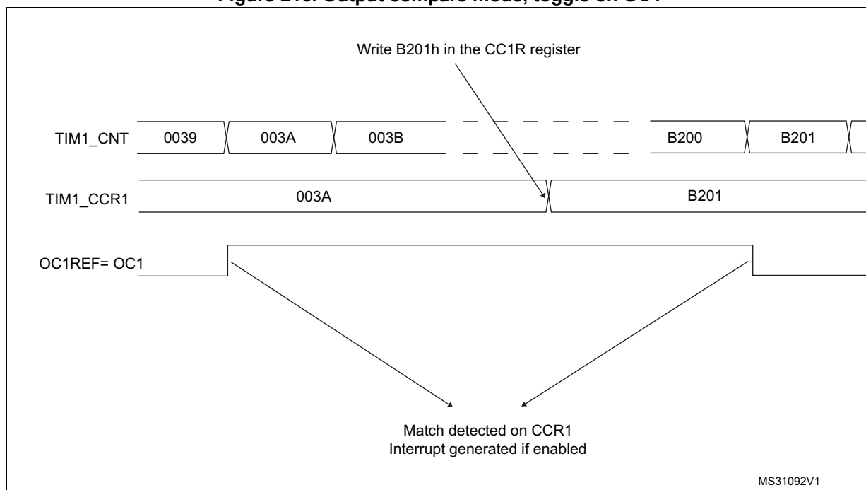
Figure 216. Output compare mode, toggle on OC1
