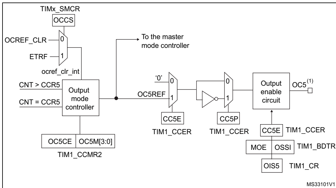
Figure 123. Output stage of capture/compare channel (channel 5, idem ch. 6)
