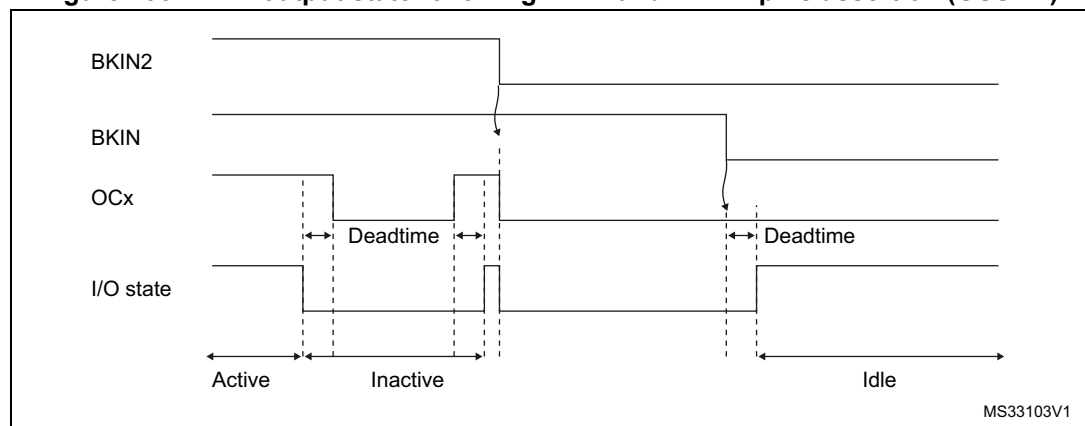
Figure 135. PWM output state following BKIN and BKIN2 pins assertion (OSSl=1)
