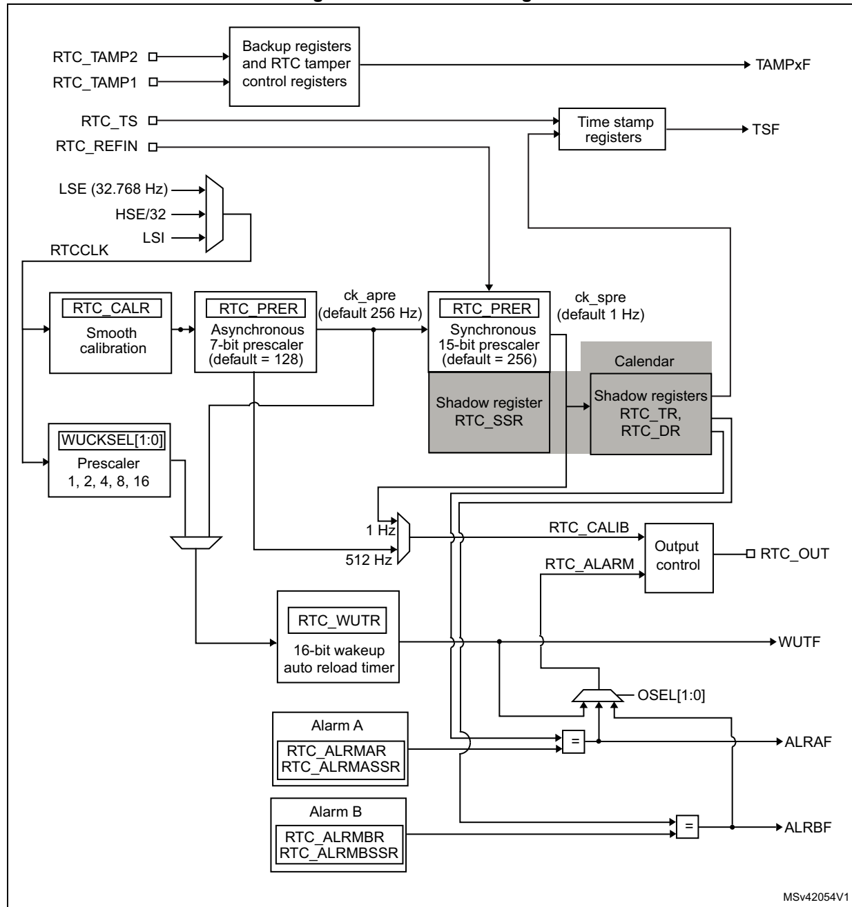
Figure 242. RTC block diagram
