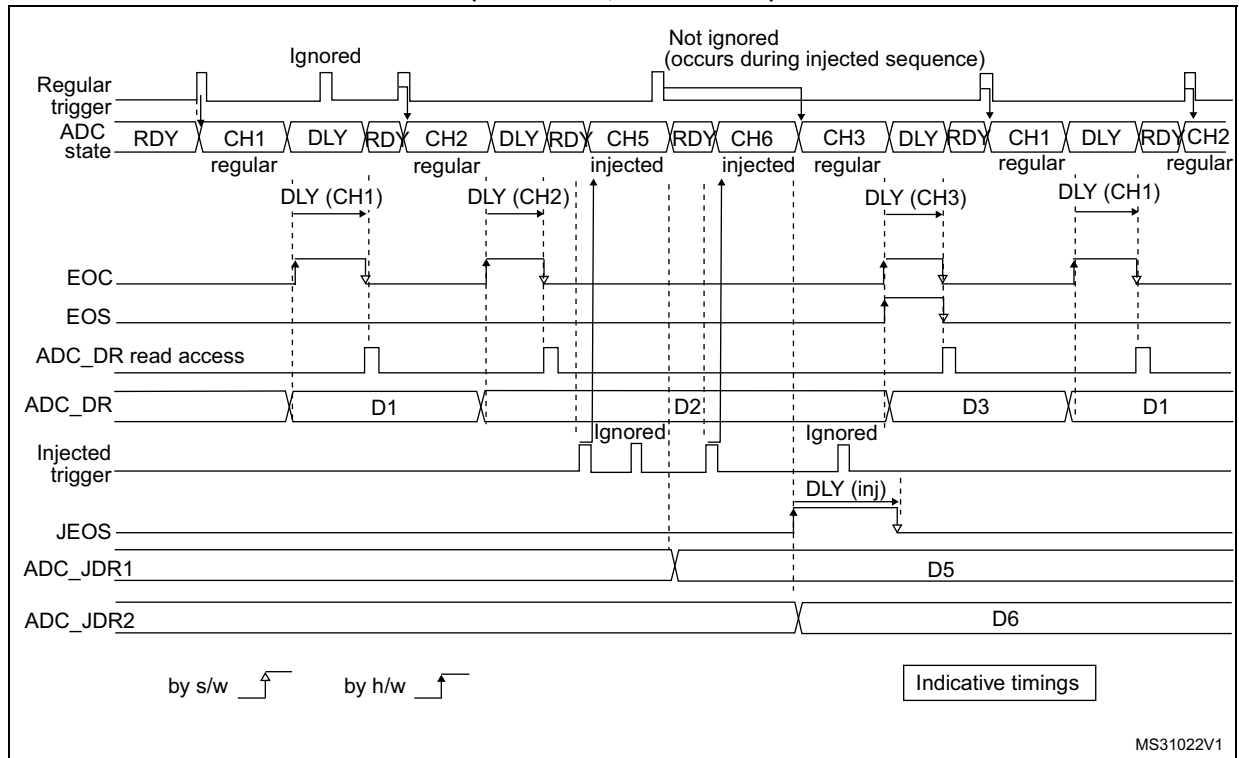
Figure 60. AUTODLY=1, regular HW conversions interrupted by injected conversions (DISCEN=1, JDISCEN=1)
