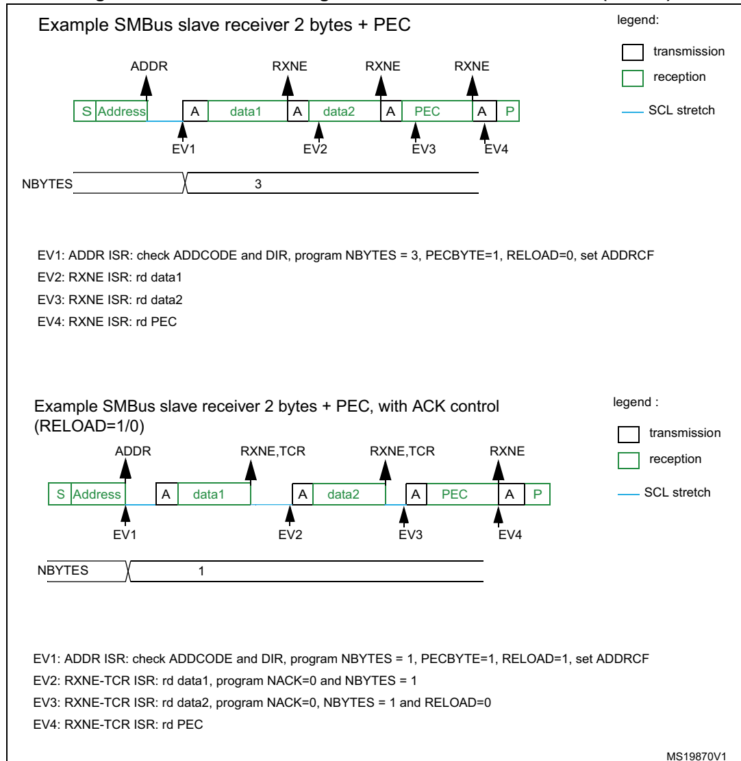
Figure 270. Bus transfer diagrams for SMBus slave receiver (SBC=1)
