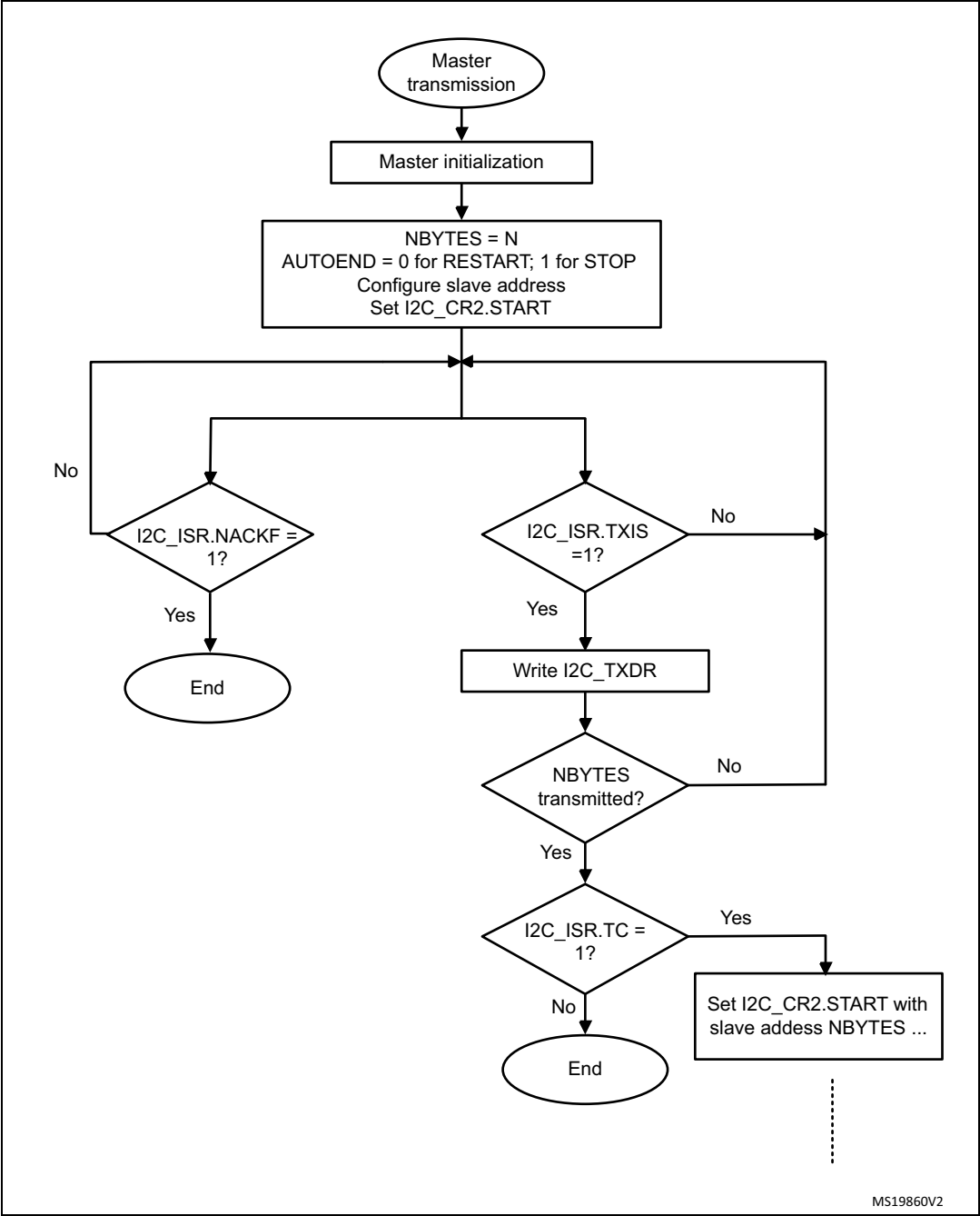
Figure 260. Transfer sequence flowchart for I2C master transmitter for N≤255 bytes
