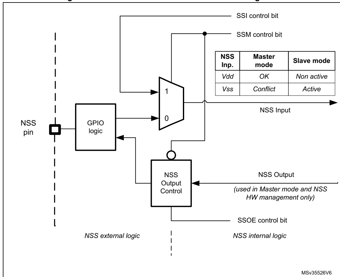
Figure 305. Hardware/software slave select management
