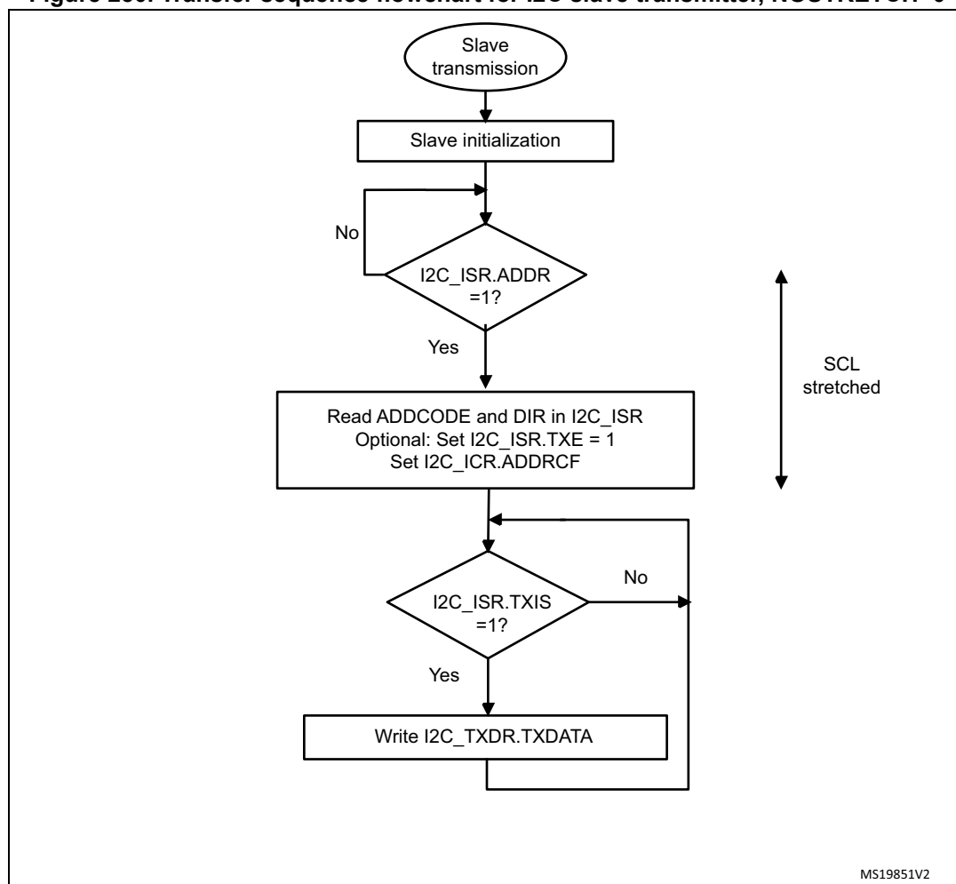
Figure 250. Transfer sequence flowchart for I2C slave transmitter, NOSTRETCH=0
