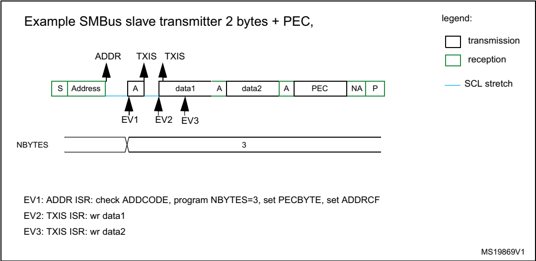
Figure 268. Transfer bus diagrams for SMBus slave transmitter (SBC=1)
