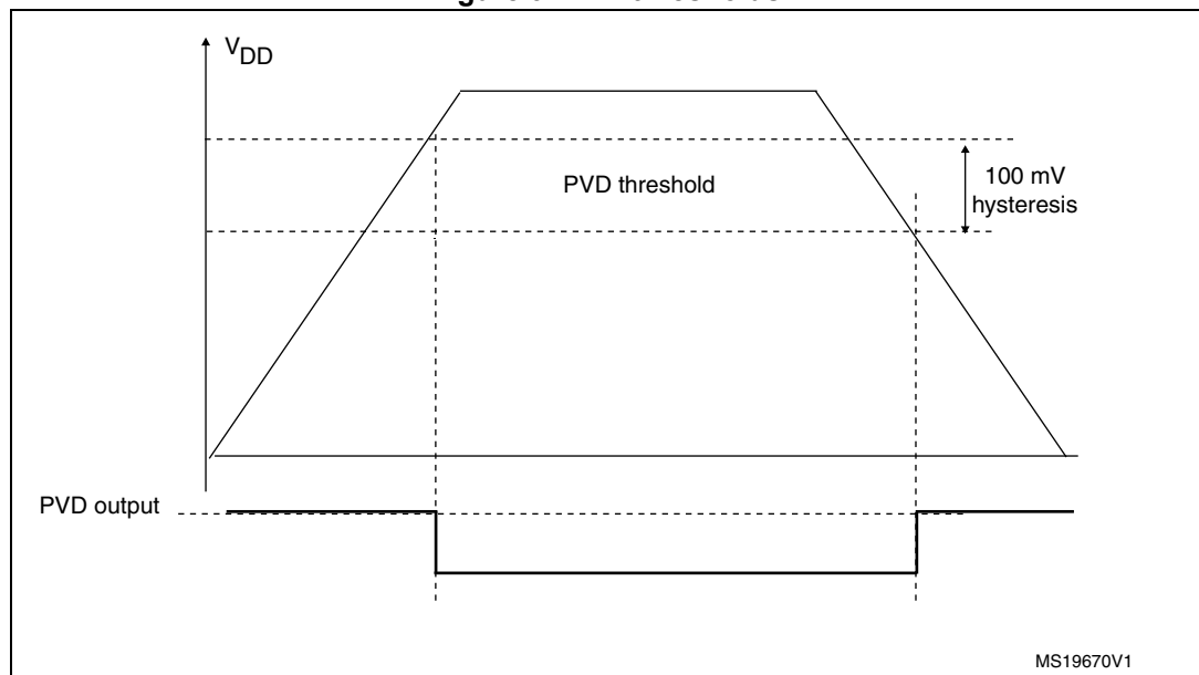
Figure 9. PVD thresholds
