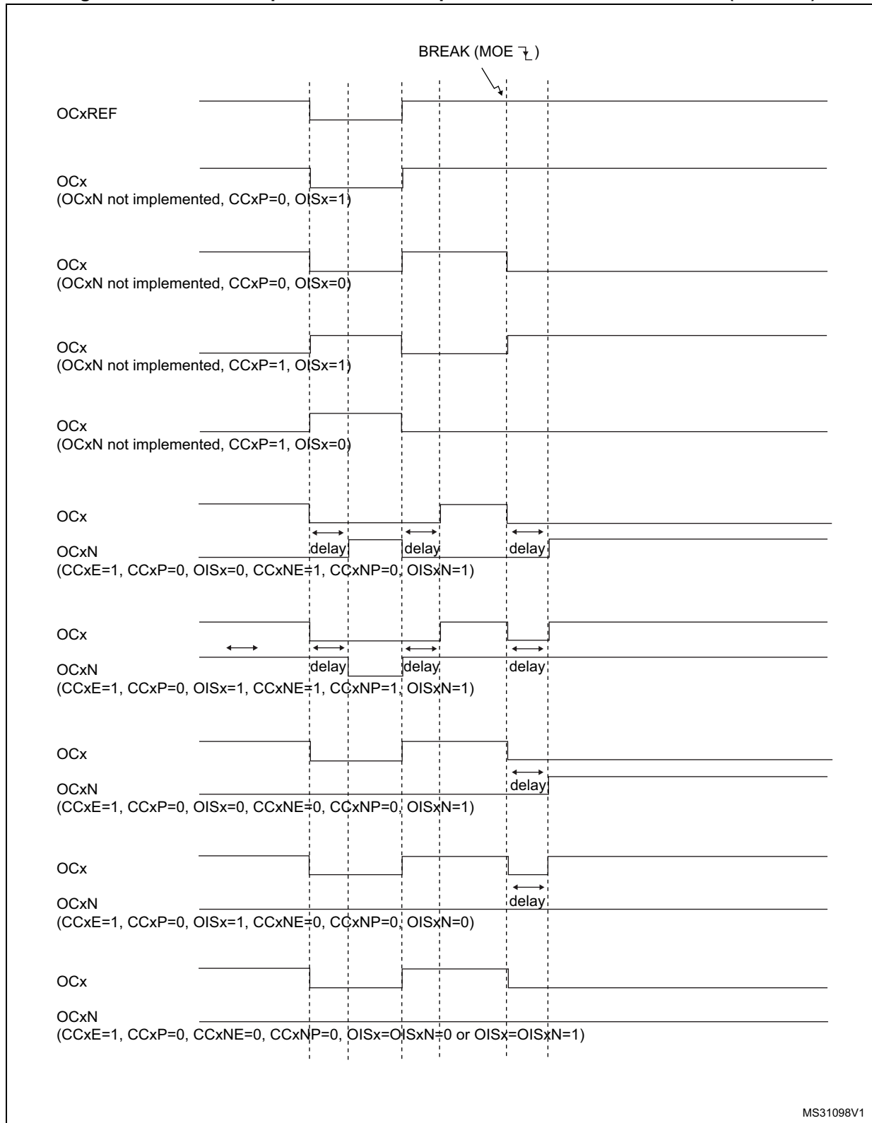
Figure 134. Various output behavior in response to a break event on BKIN (OSS1 = 1)
