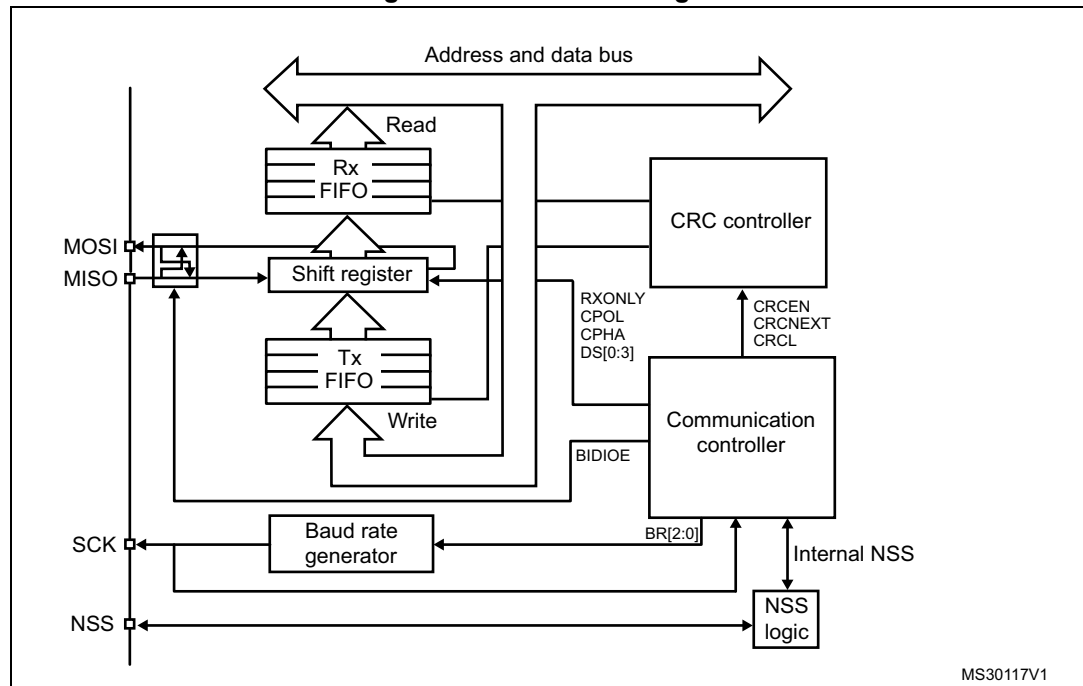
Figure 299. SPI block diagram
