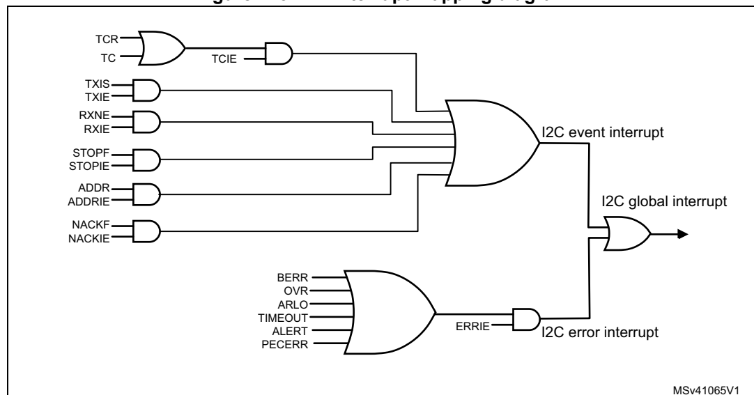
Figure 273. I2C interrupt mapping diagram
