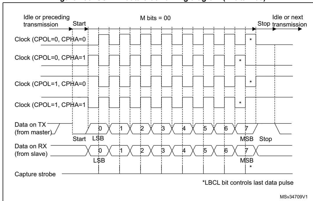
Figure 286. USART data clock timing diagram (M bits = 00)
