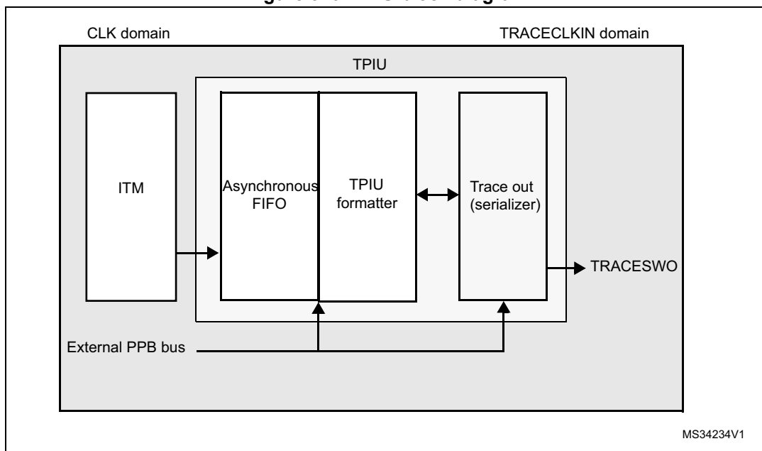
Figure 340. TPIU block diagram
