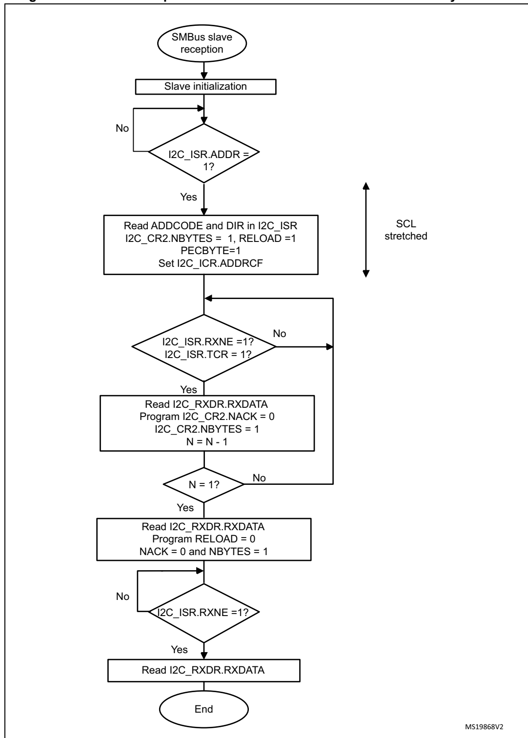
Figure 269. Transfer sequence flowchart for SMBus slave receiver N Bytes + PEC
