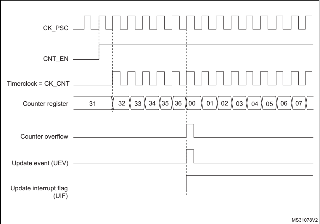
Figure 201. Counter timing diagram, internal clock divided by 1
