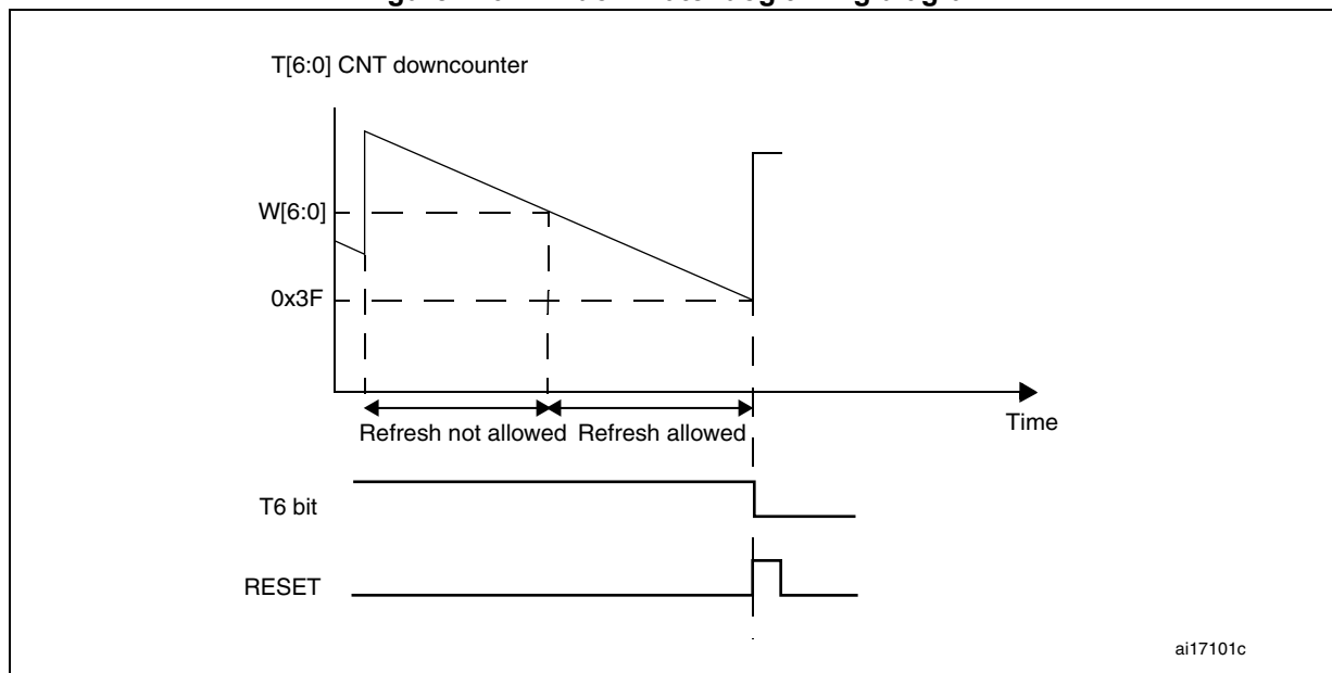
Figure 240. Window watchdog timing diagram
