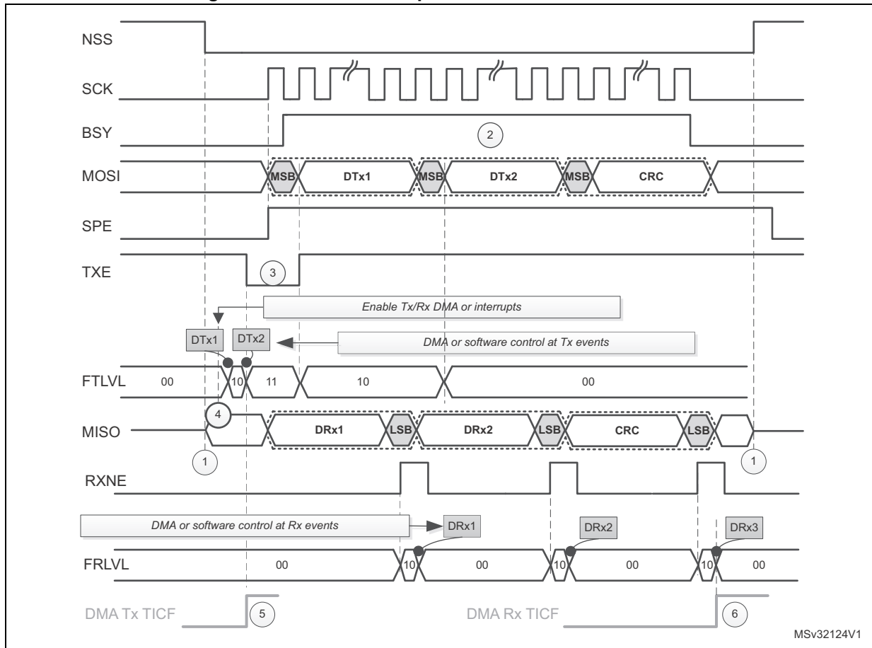
Figure 311. Master full duplex communication with CRC
