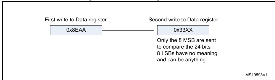
Figure 319. Transmitting 0x8EAA33
