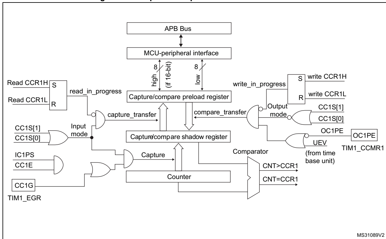
Figure 120. Capture/compare channel 1 main circuit
