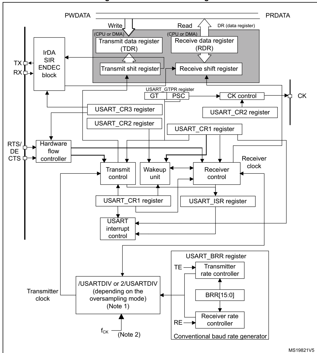
Figure 274. USART block diagram
