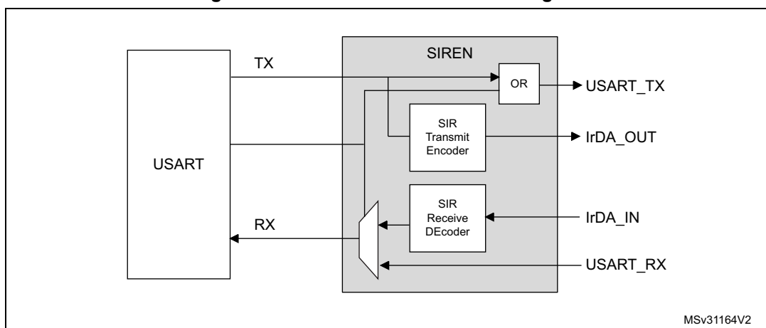
Figure 291. IrDA SIR ENDEC- block diagram
