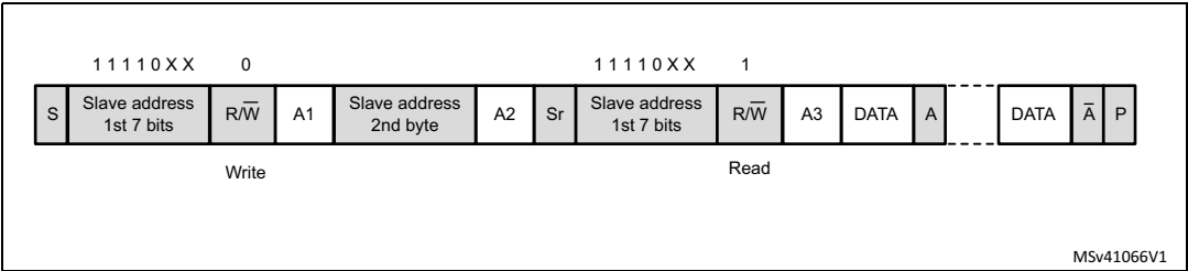
Figure 258. 10-bit address read access with HEAD10R=0
