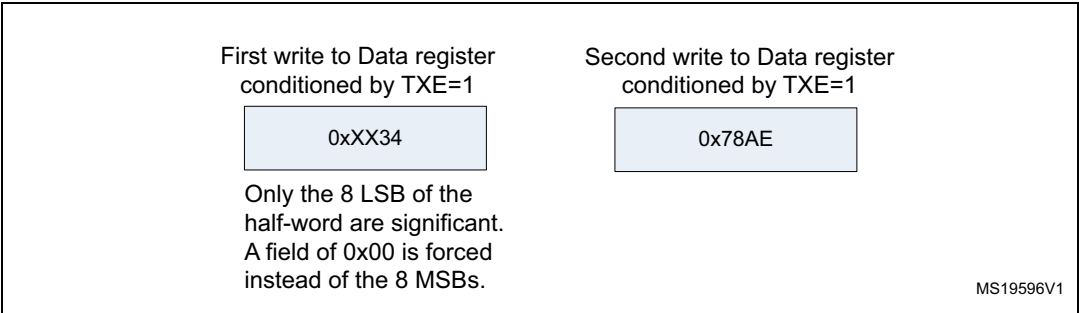
Figure 328. Operations required to transmit 0x3478AE
