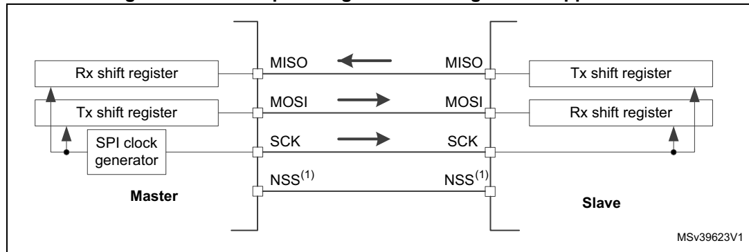
Figure 300. Full-duplex single master/ single slave application
