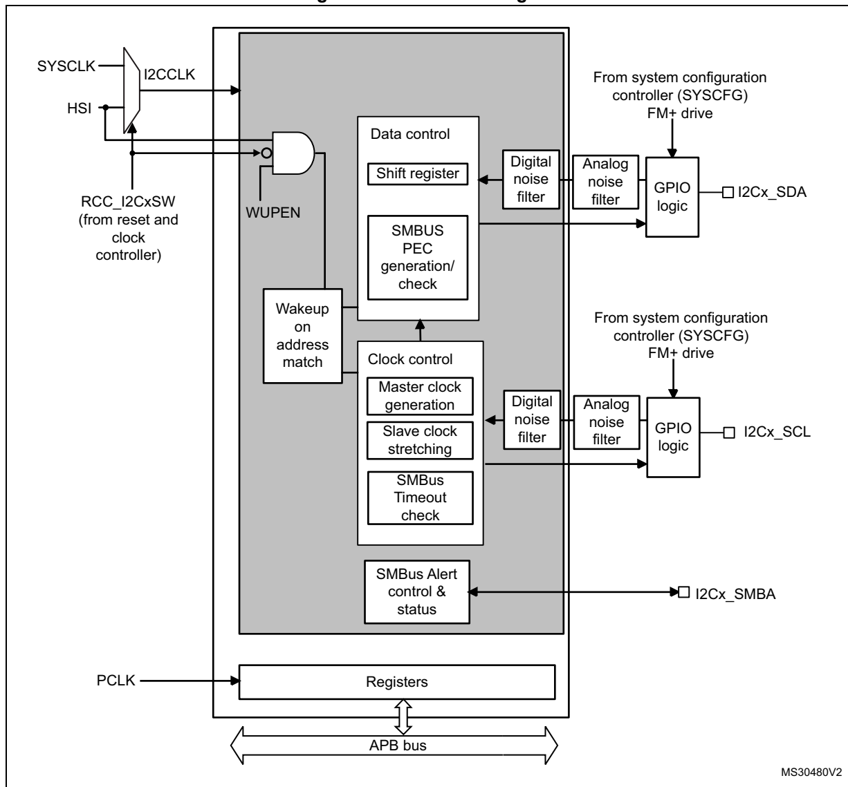
Figure 243. I2C block diagram
