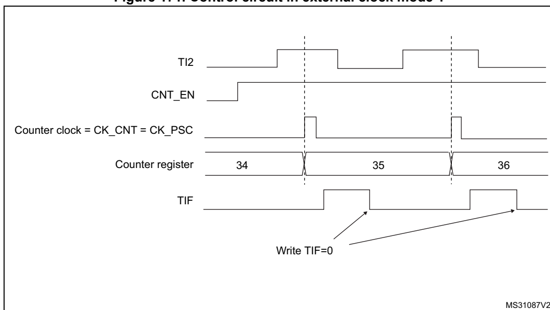
Figure 171. Control circuit in external clock mode 1
