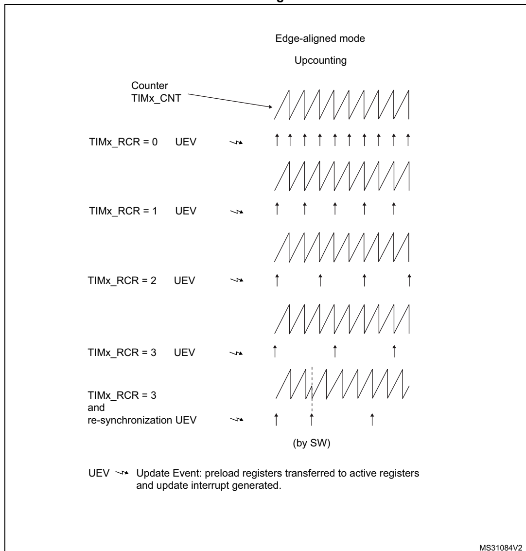
Figure 207. Update rate examples depending on mode and TIMx_RCR register settings
