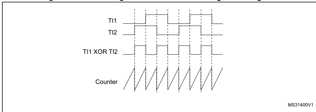
Figure 224. Measuring time interval between edges on 2 signals
