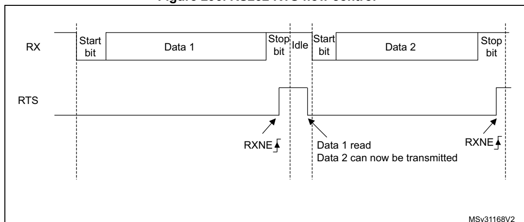
Figure 296. RS232 RTS flow control
