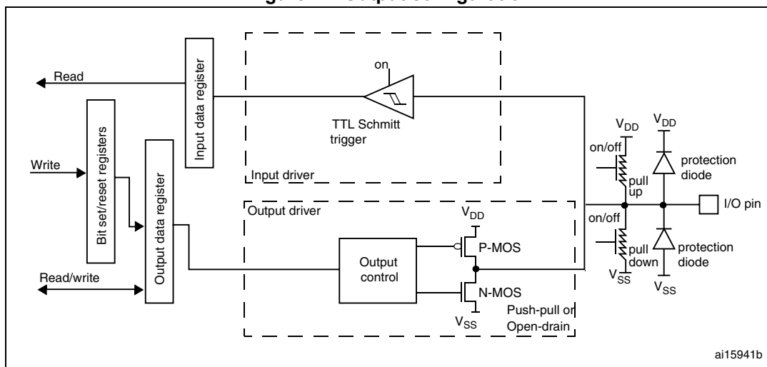
Figure 17. Output configuration
