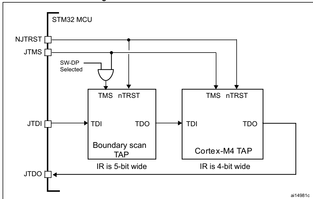
Figure 339. JTAG TAP connections
