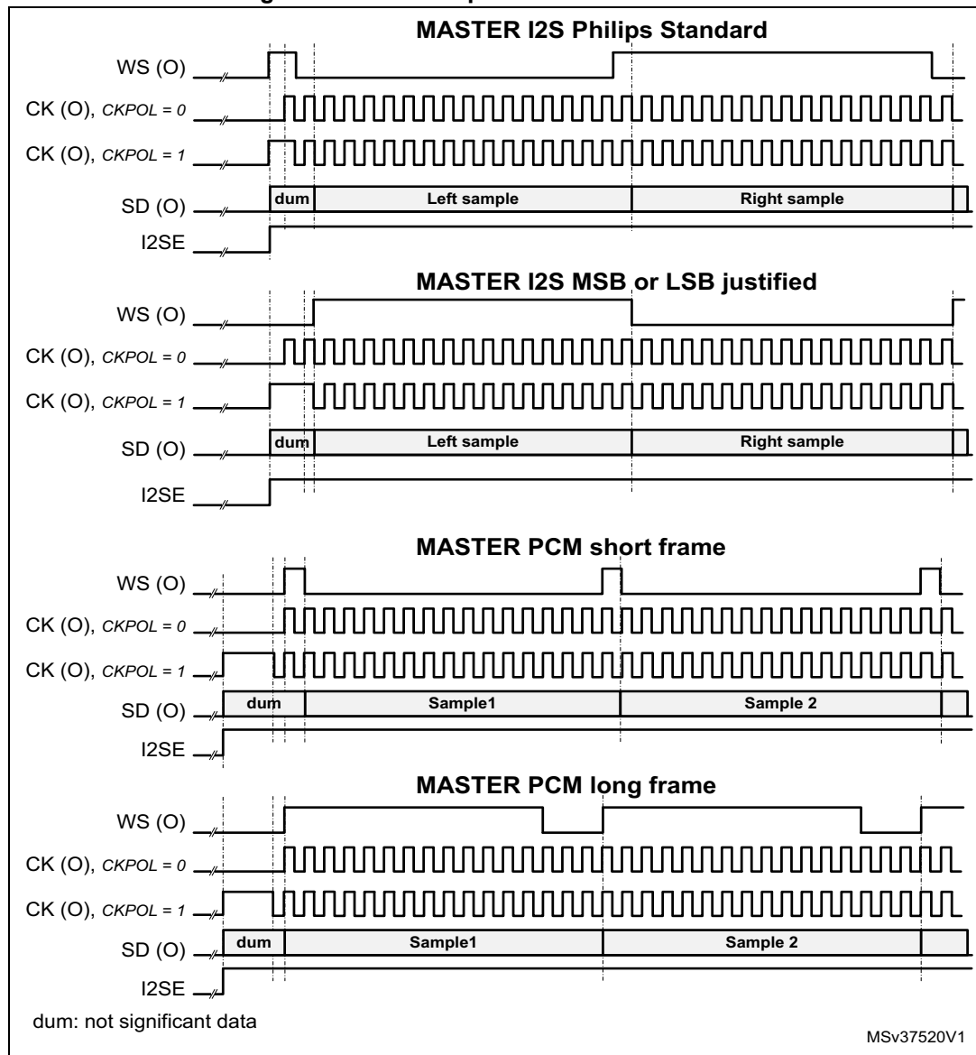
Figure 334. Start sequence in MASTER mode
