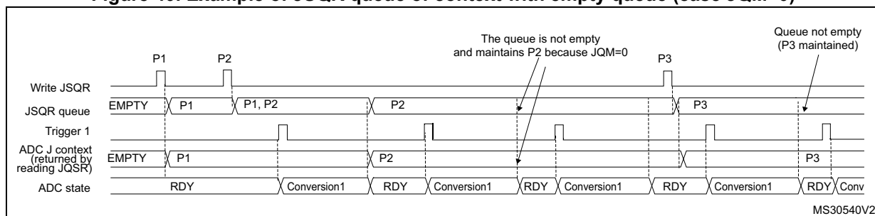
Figure 40. Example of JSQR queue of context with empty queue (case JQM=0)
