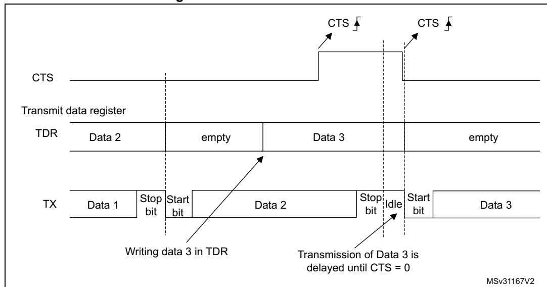
Figure 297. RS232 CTS flow control
