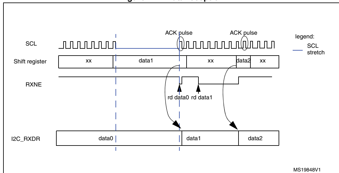
Figure 247. Data reception
