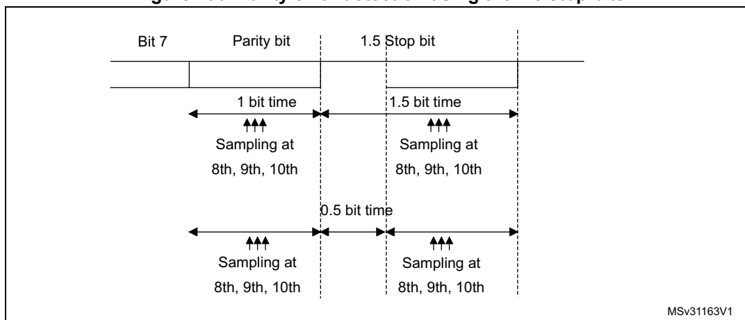
Figure 290. Parity error detection using the 1.5 stop bits
