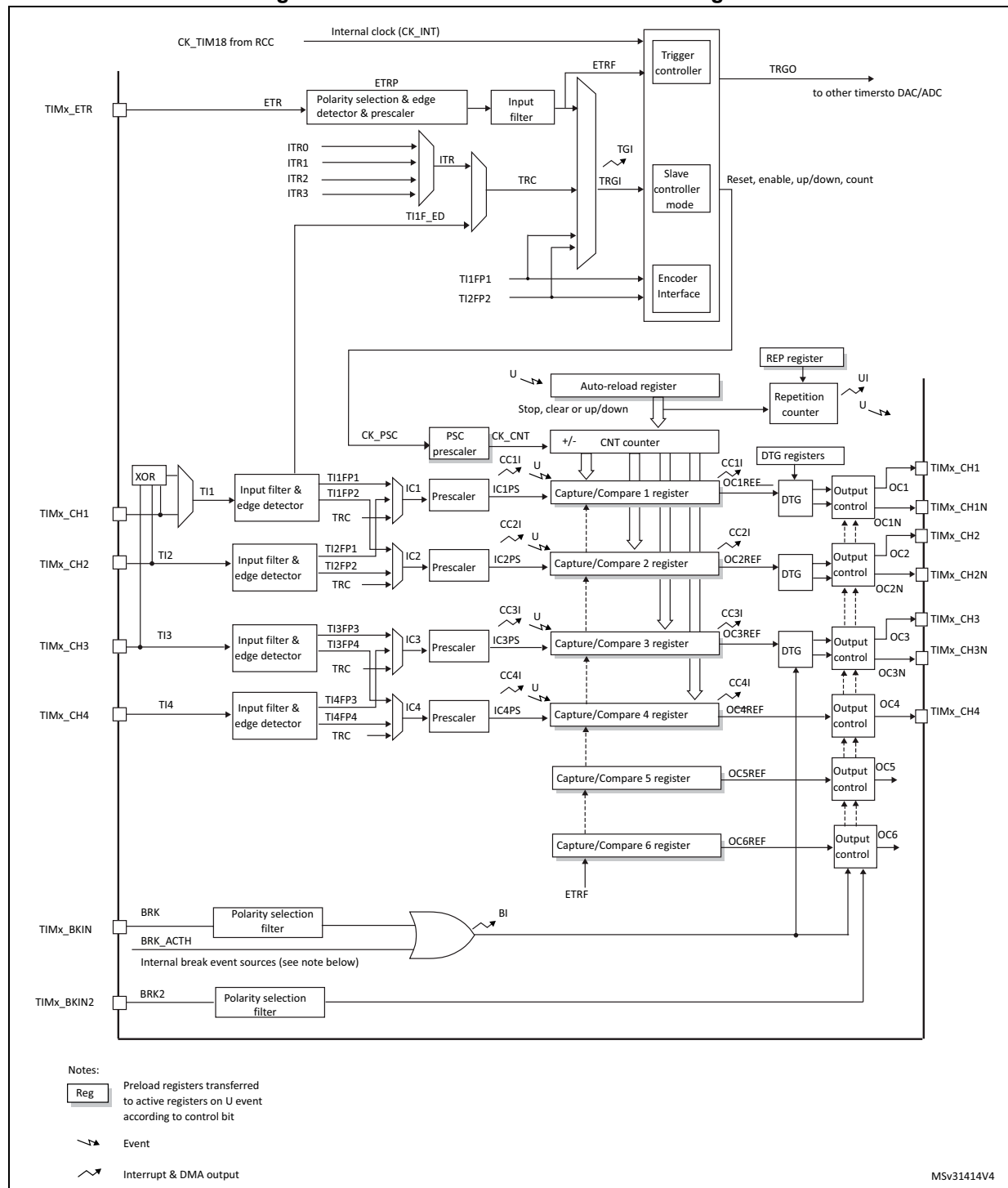
Figure 92. Advanced-control timer block diagram
