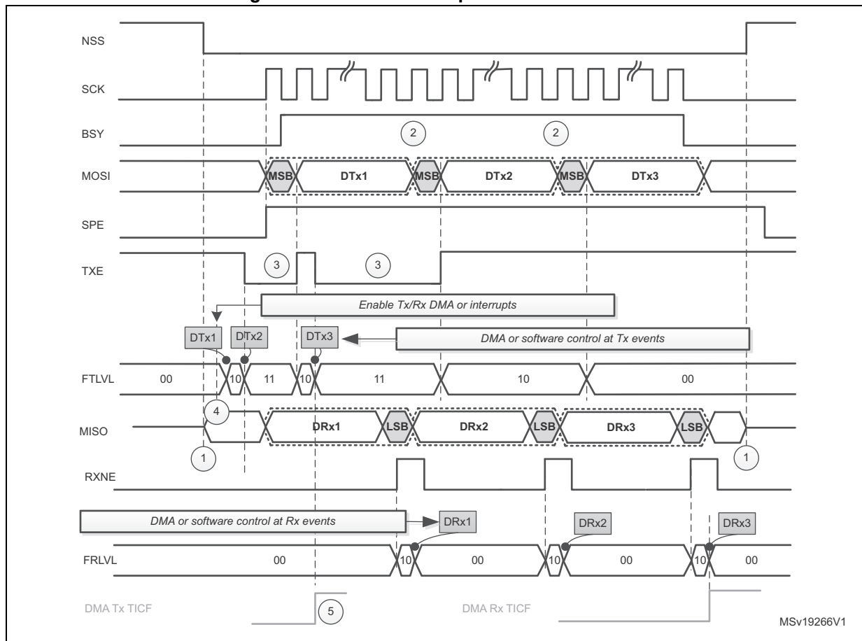
Figure 309. Master full duplex communication
