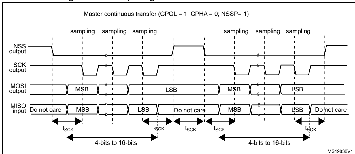
Figure 313. NSSP pulse generation in Motorola SPI master mode
