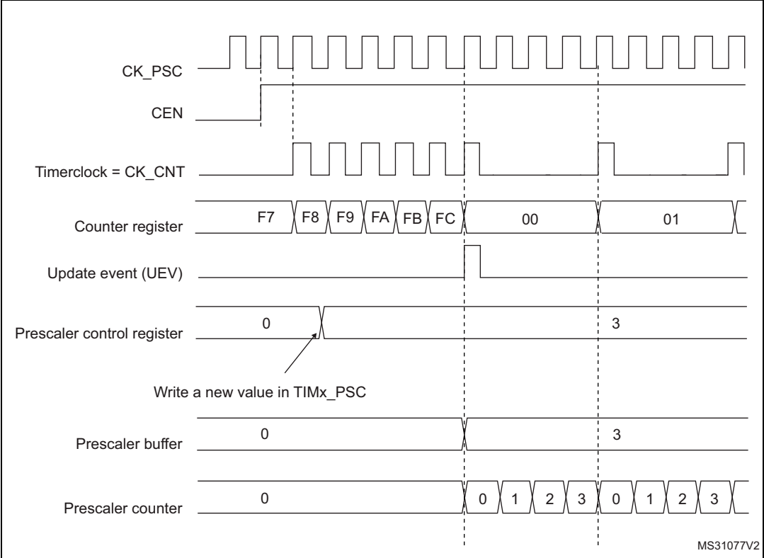
Figure 200. Counter timing diagram with prescaler division change from 1 to 4
