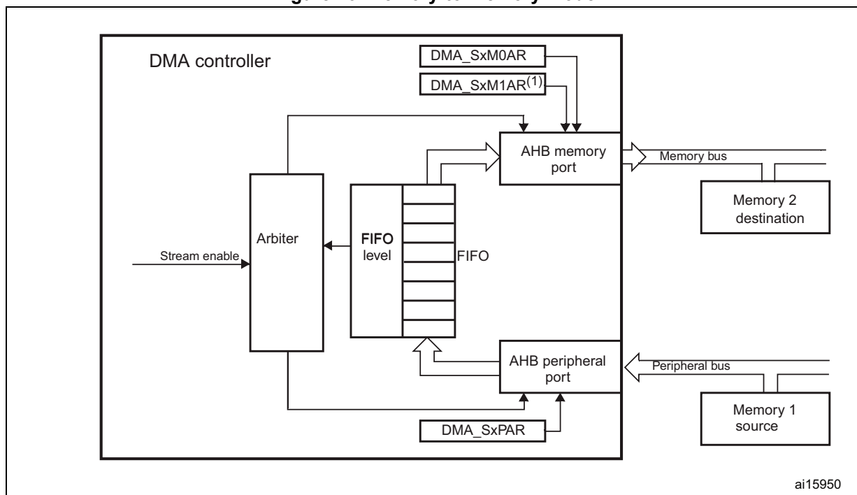
Figure 26. Memory-to-memory mode
