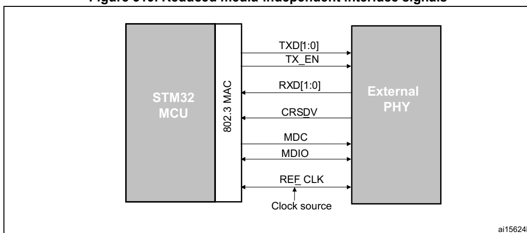
Figure 319. Reduced media-independent interface signals
