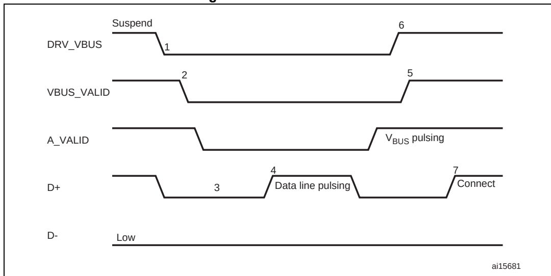
Figure 369. A-device SRP
