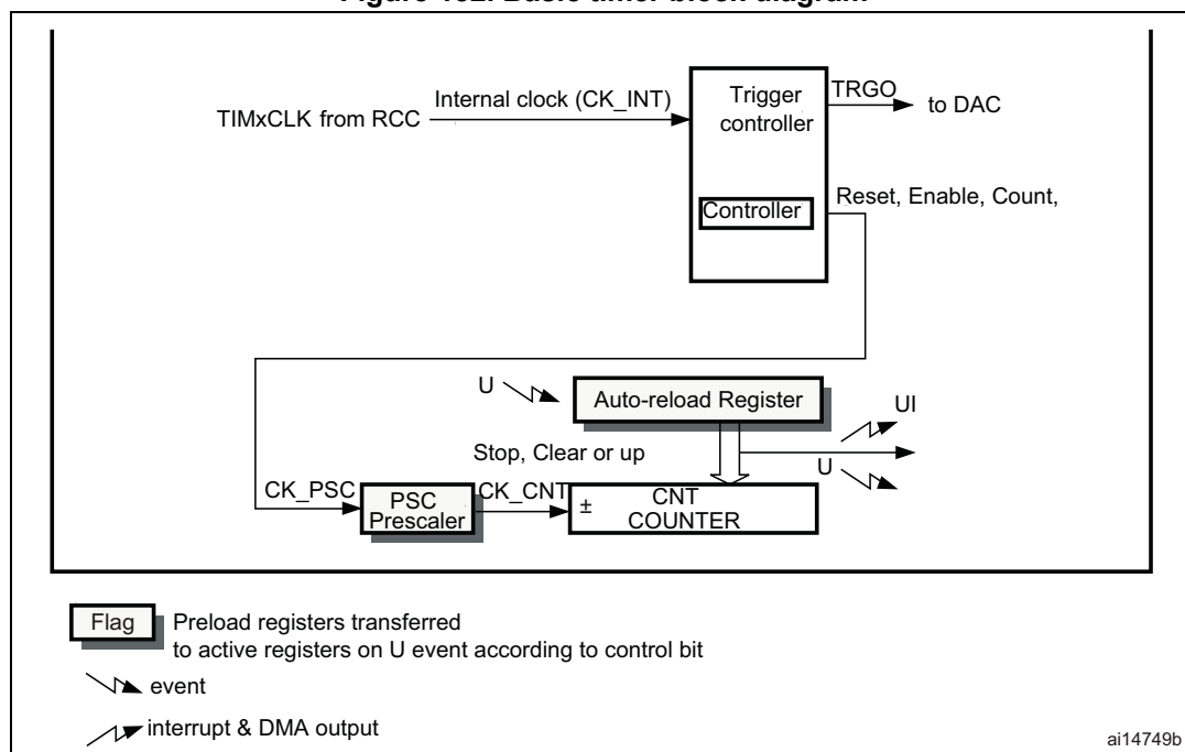
Figure 182. Basic timer block diagram
