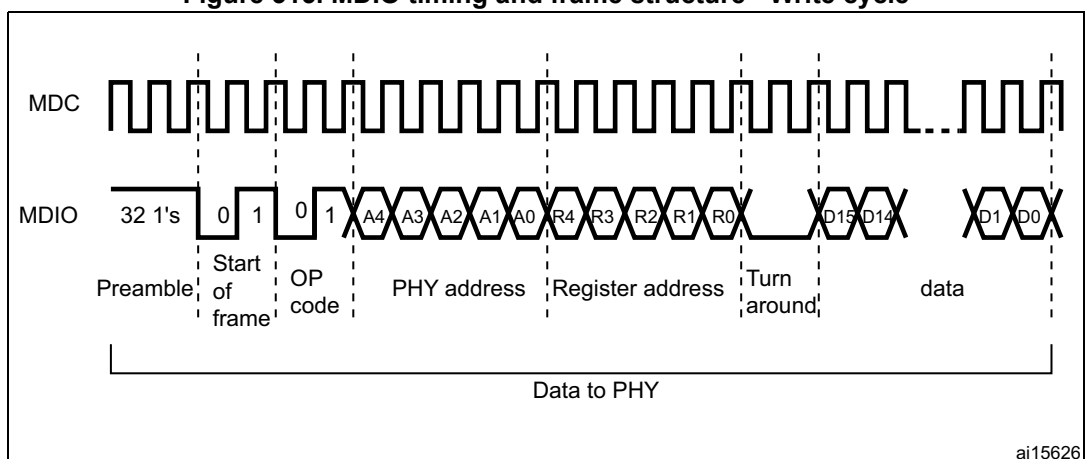
Figure 315. MDIO timing and frame structure - Write cycle
