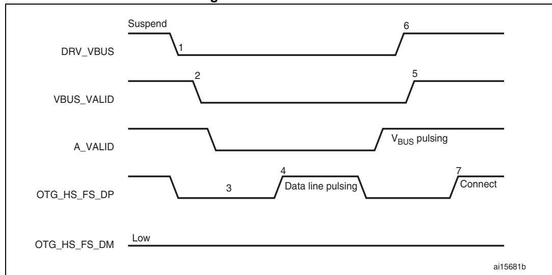
Figure 393. A-device SRP
