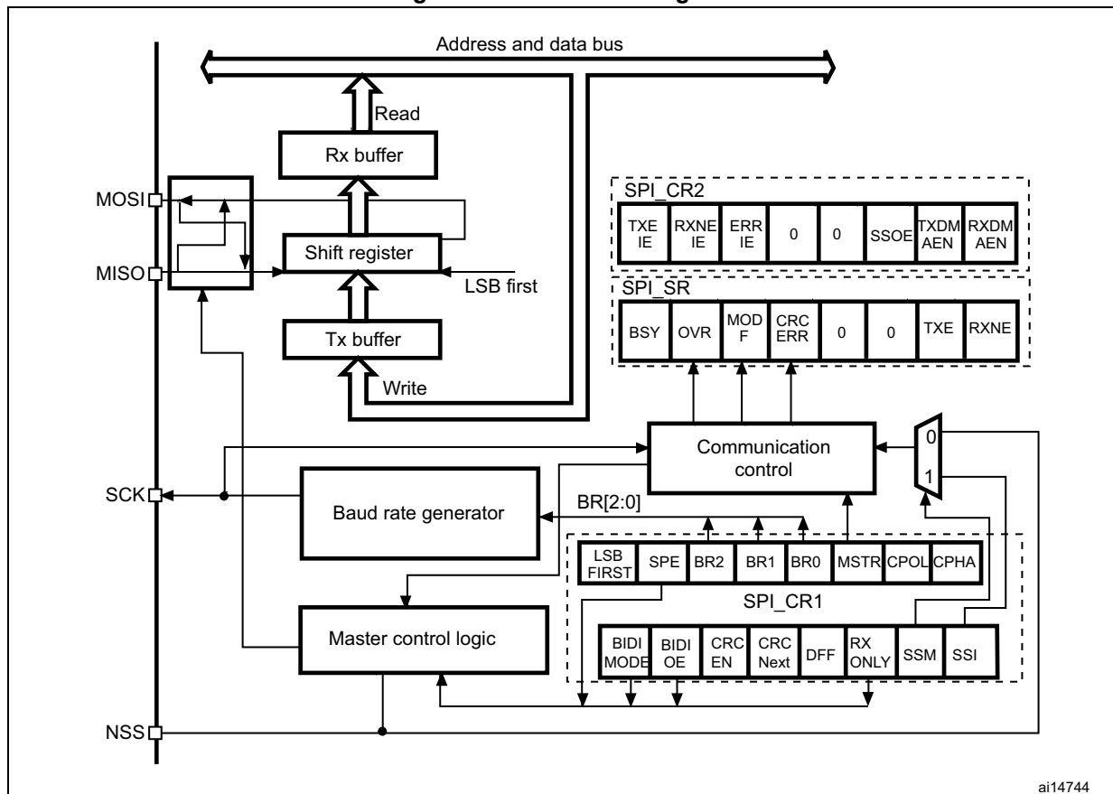
Figure 248. SPI block diagram
