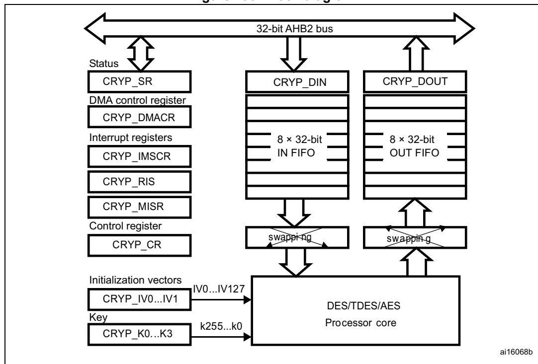
Figure 195. Block diagram
