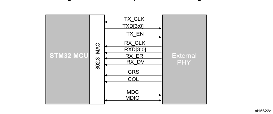
Figure 317. Media independent interface signals
