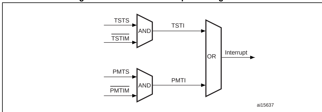
Figure 333. MAC core interrupt masking scheme
