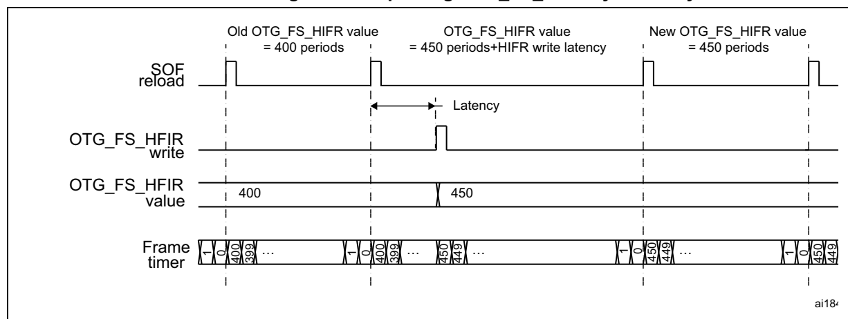
Figure 354. Updating OTG_FS_HFIR dynamically
