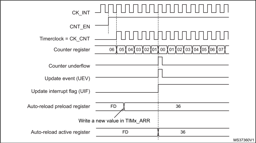
Figure 131. Counter timing diagram, Update event with ARPE=1 (counter underflow)
