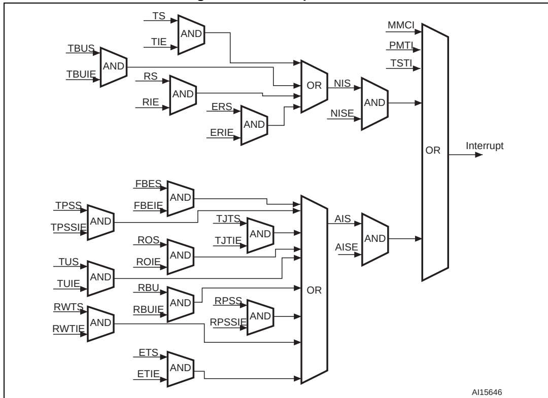
Figure 347. Interrupt scheme
