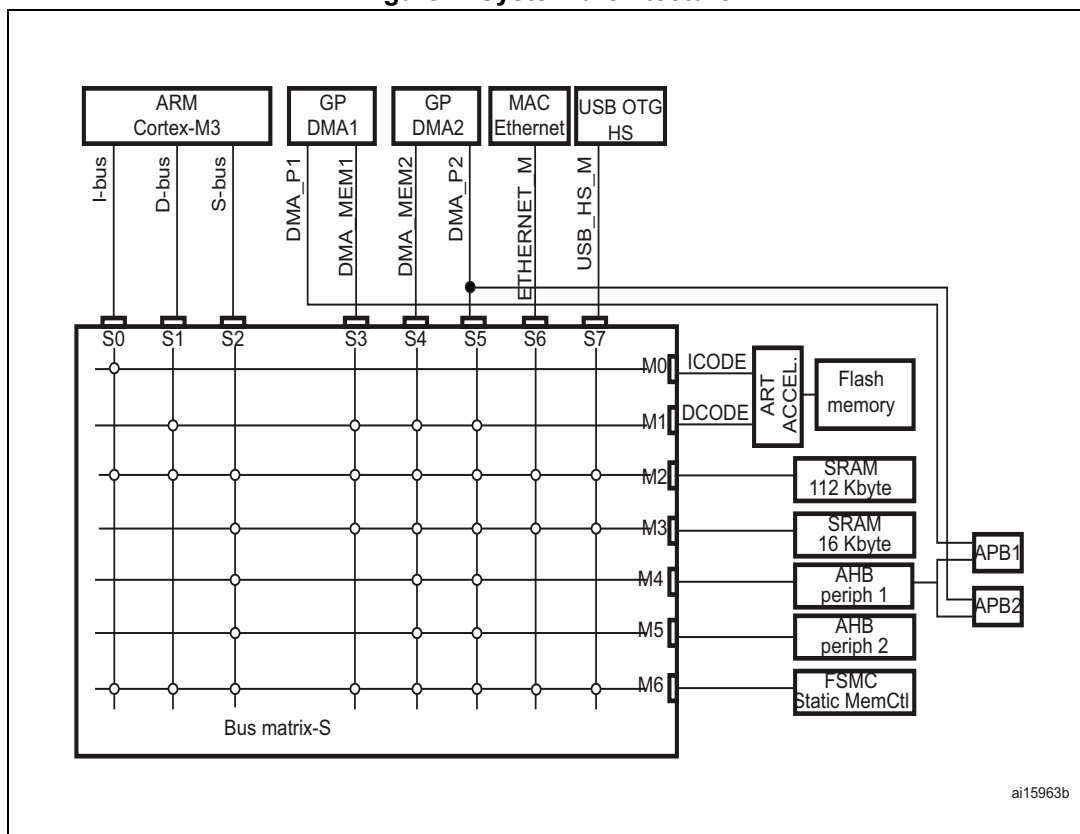
Figure 1. System architecture
