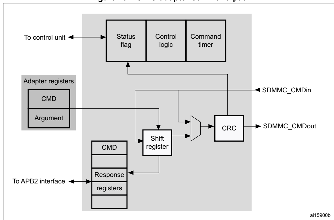
Figure 292. SDIO adapter command path
