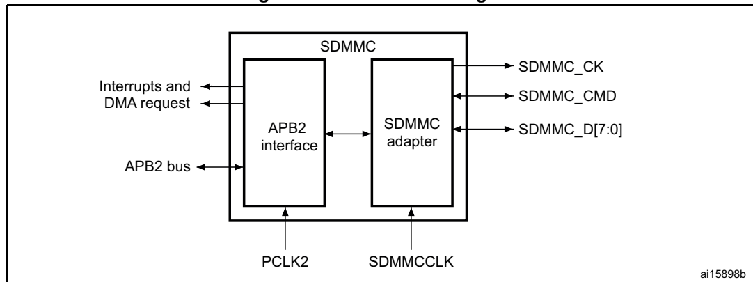
Figure 289. SDIO block diagram
