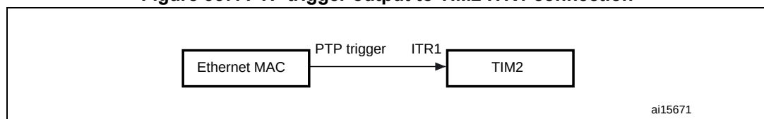
Figure 337. PTP trigger output to TIM2 ITR1 connection
