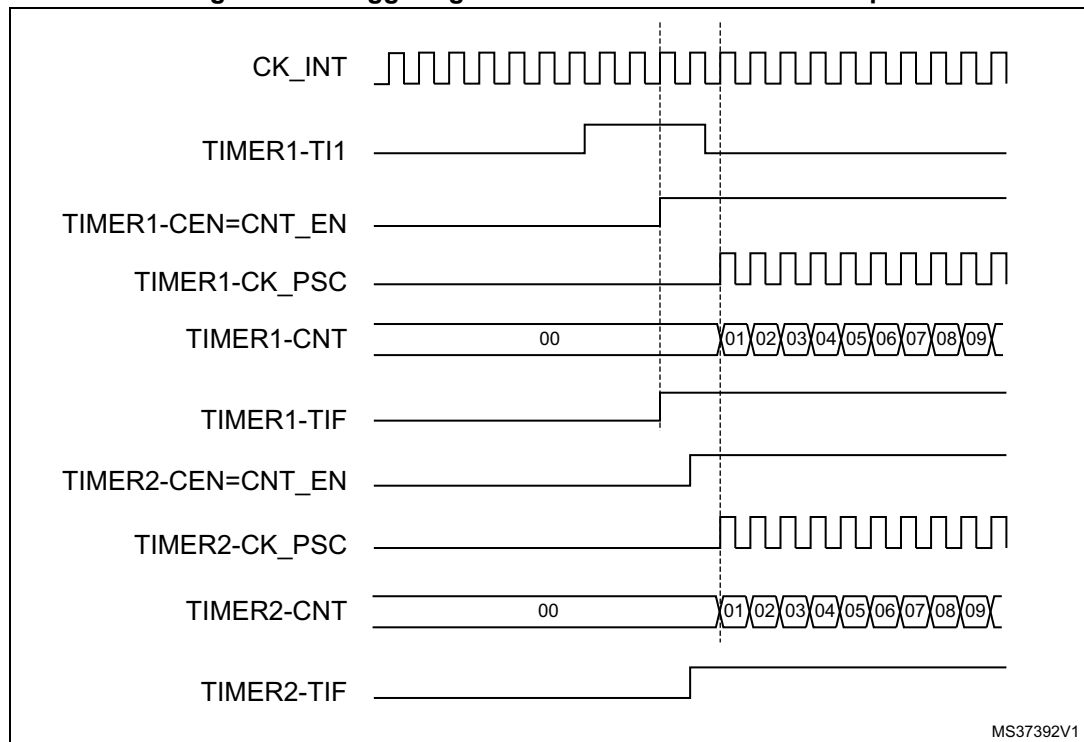
Figure 158. Triggering timer 1 and 2 with timer 1 TI1 input
