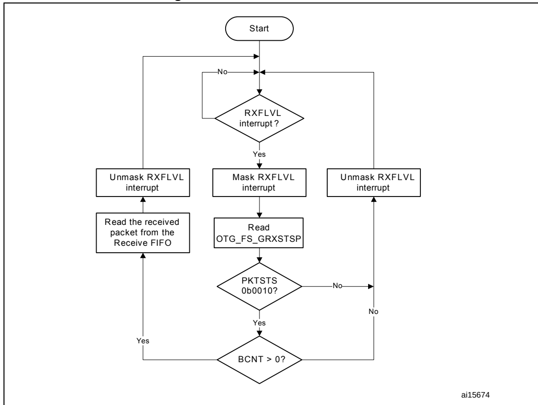
Figure 380. Receive FIFO read task
