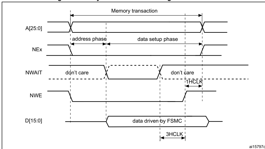
Figure 413. Asynchronous wait during a write access
