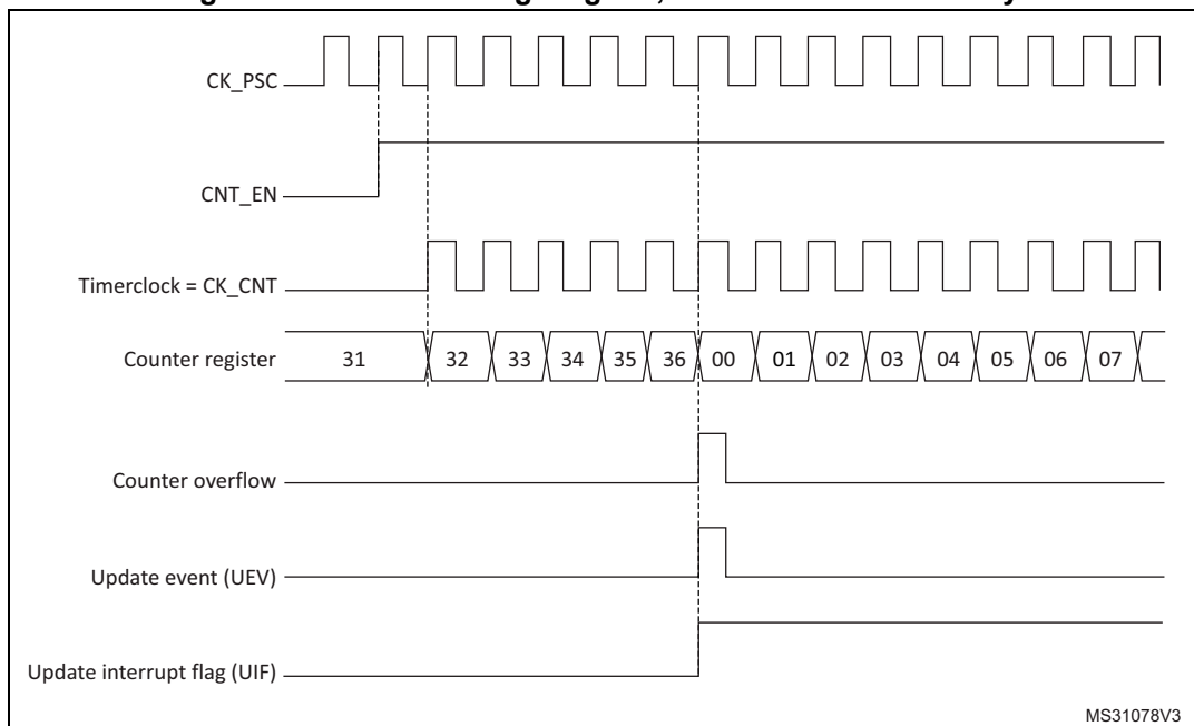
Figure 68. Counter timing diagram, internal clock divided by 1
