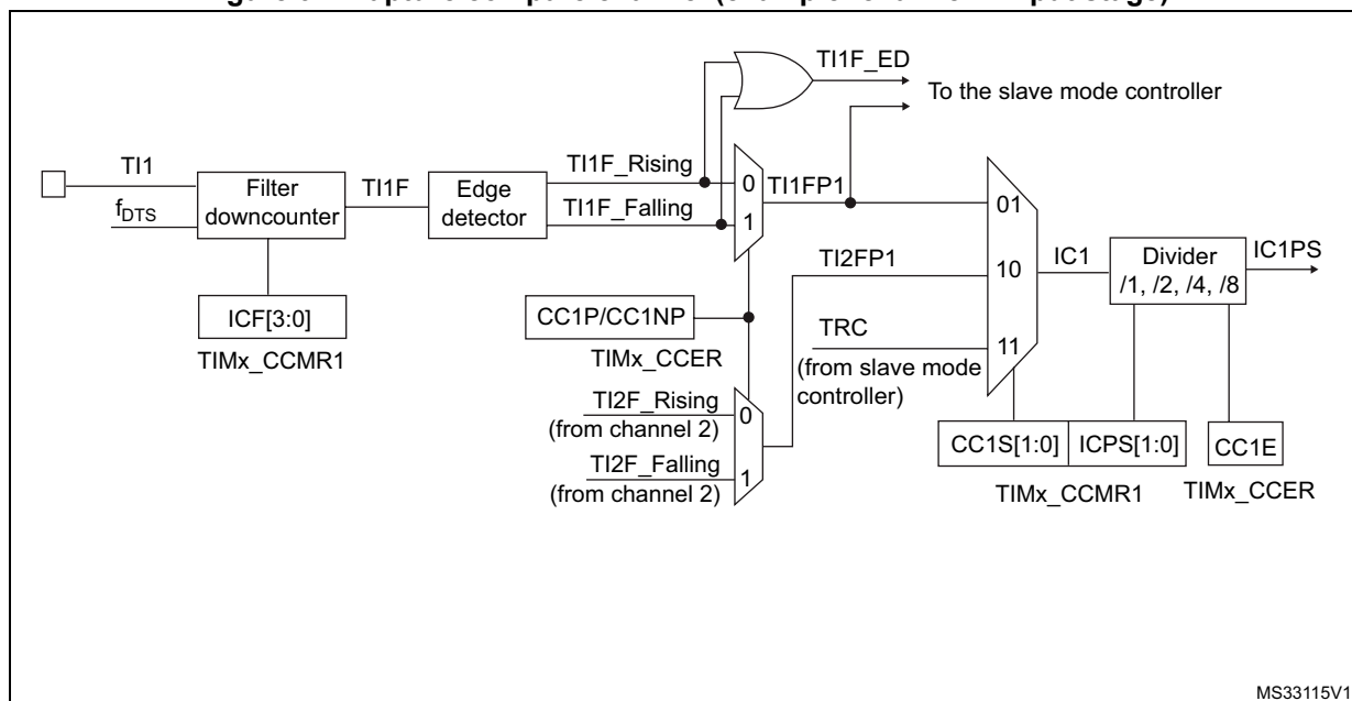
Figure 91. Capture/compare channel (example: channel 1 input stage)
