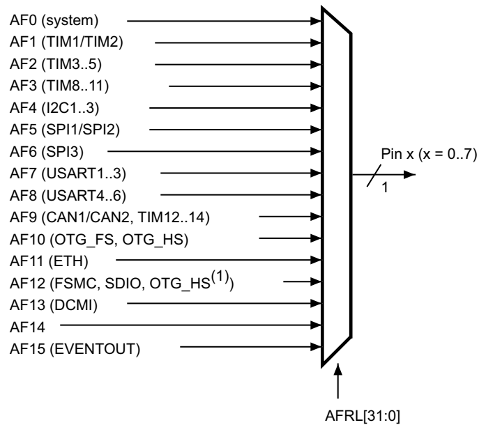
Figure 14. Selecting an alternate function
