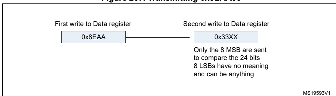
Figure 267. Transmitting 0x8EAA33
