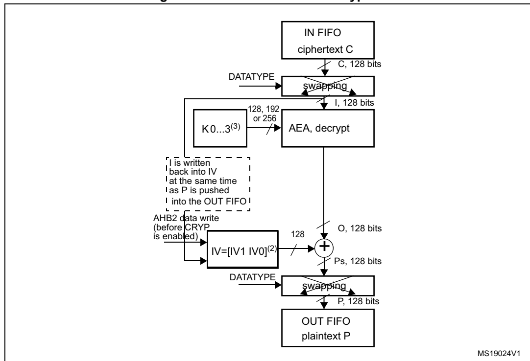
Figure 203. AES-CBC mode decryption
