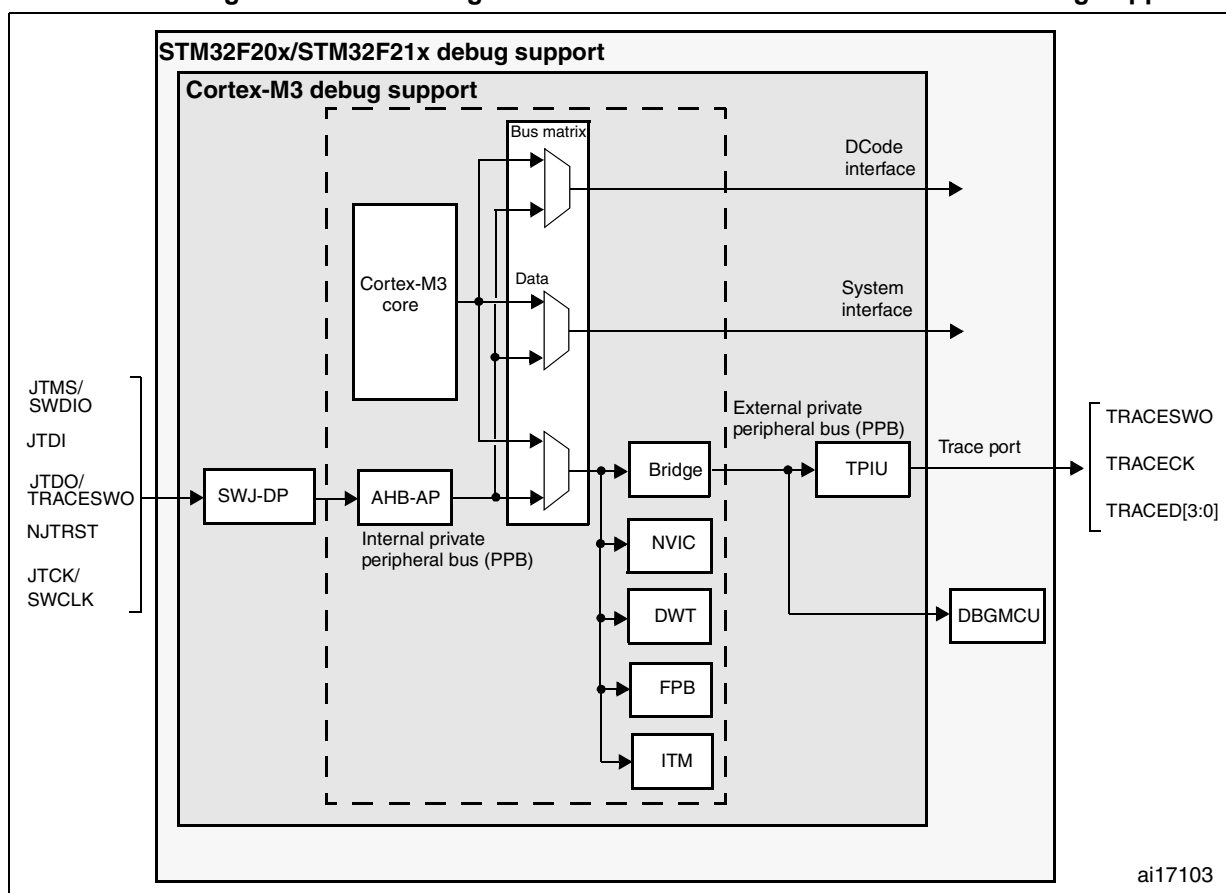
Figure 419. Block diagram of STM32 MCU and Cortex®-M3-level debug support
