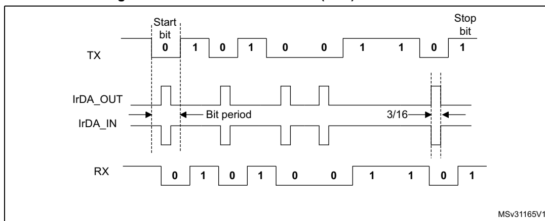
Figure 241. IrDA data modulation (3/16) -Normal mode
