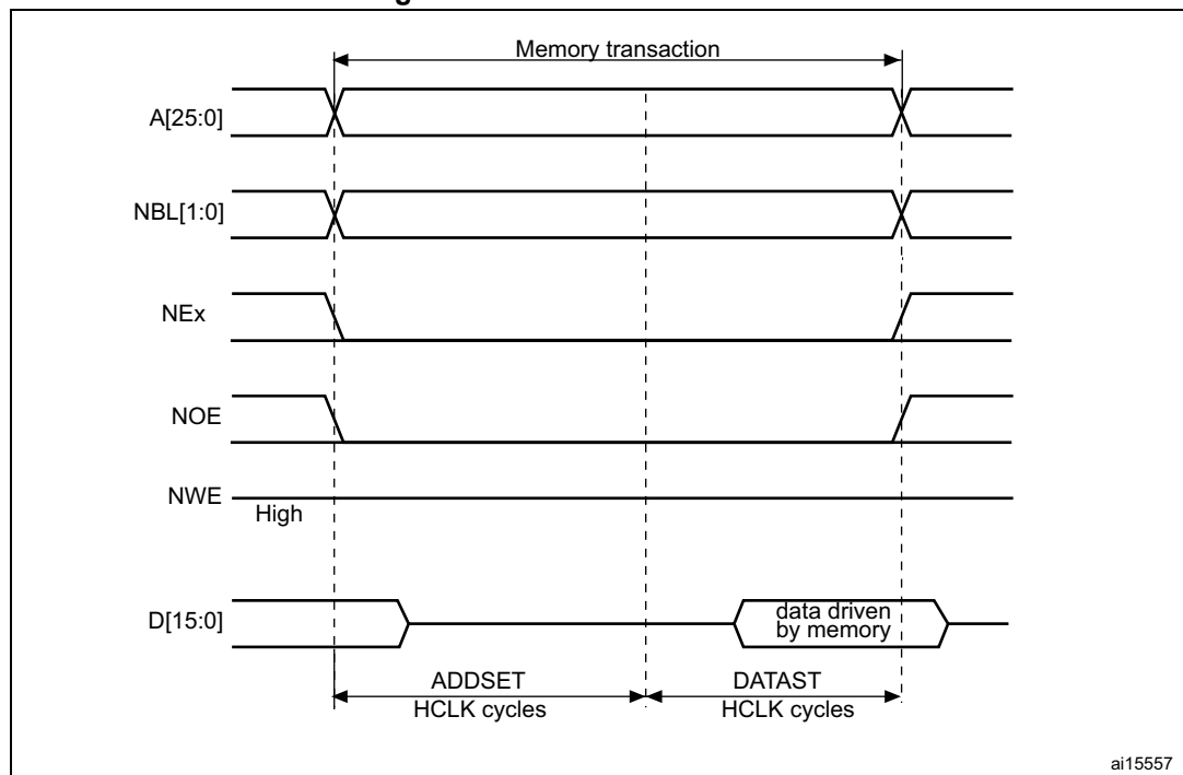
Figure 399. Mode1 read accesses
