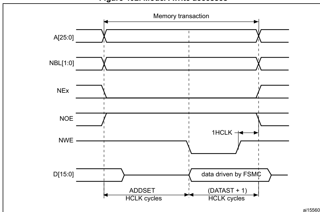
Figure 402. ModeA write accesses
