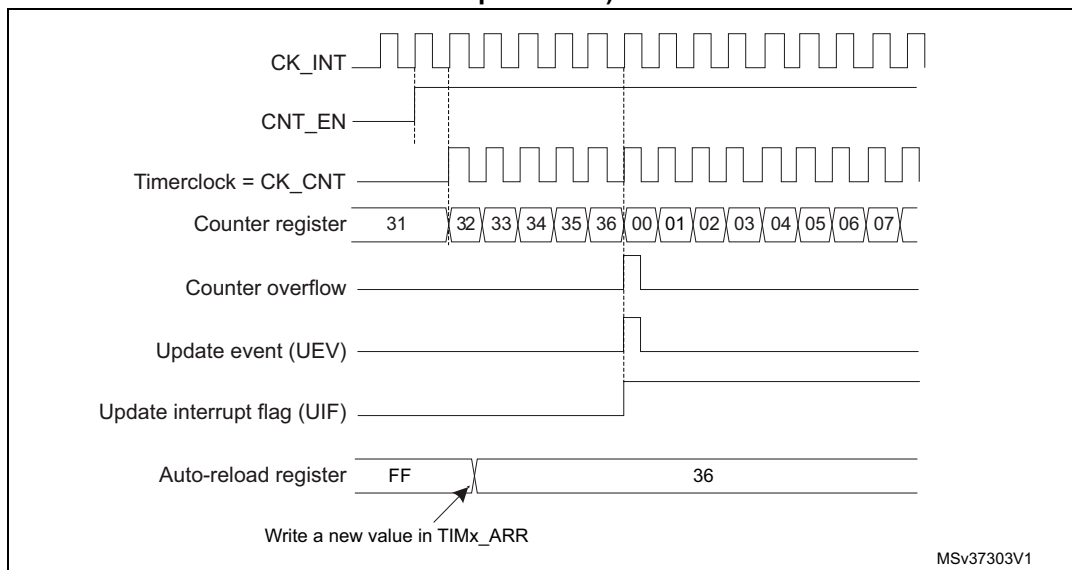
Figure 120. Counter timing diagram, Update event when ARPE=0 (TIMx_ARR not preloaded)
