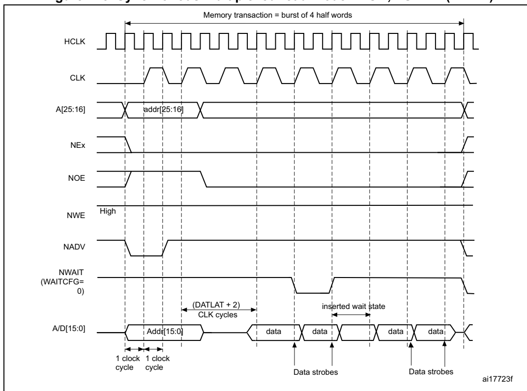
Figure 415. Synchronous multiplexed read mode - NOR, PSRAM (CRAM)
