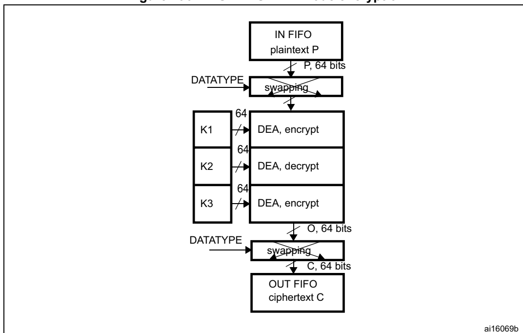
Figure 196. DES/TDES-ECB mode encryption
