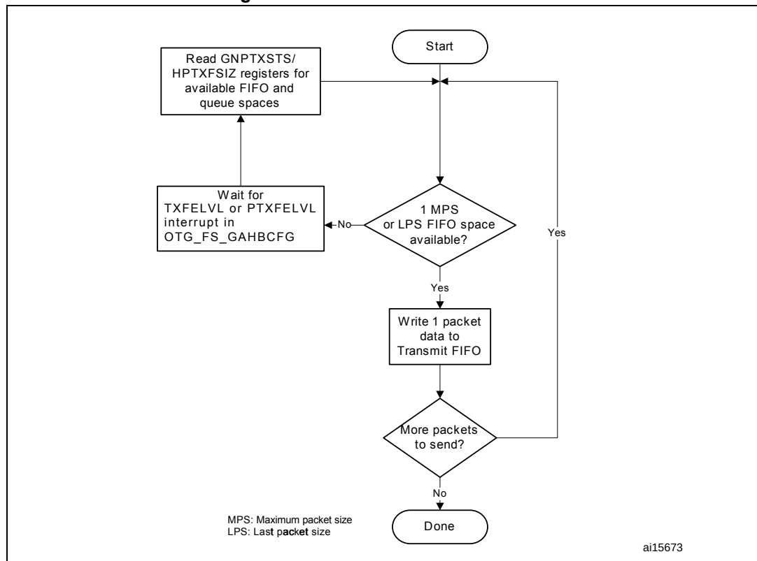
Figure 379. Transmit FIFO write task
