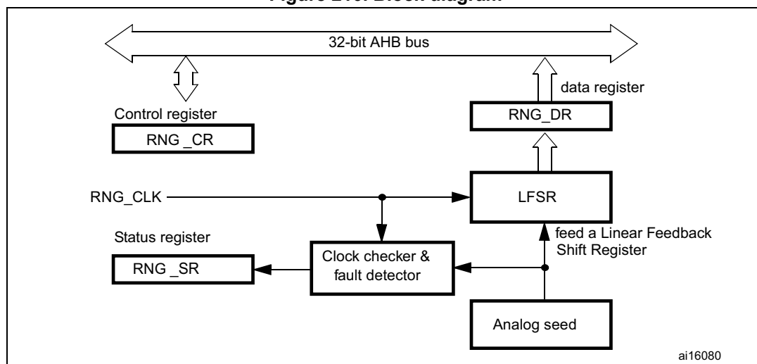
Figure 210. Block diagram
