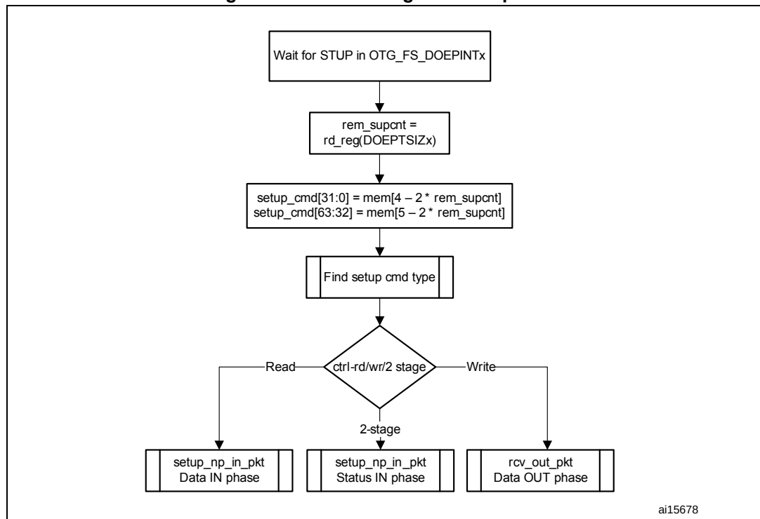
Figure 390. Processing a SETUP packet
