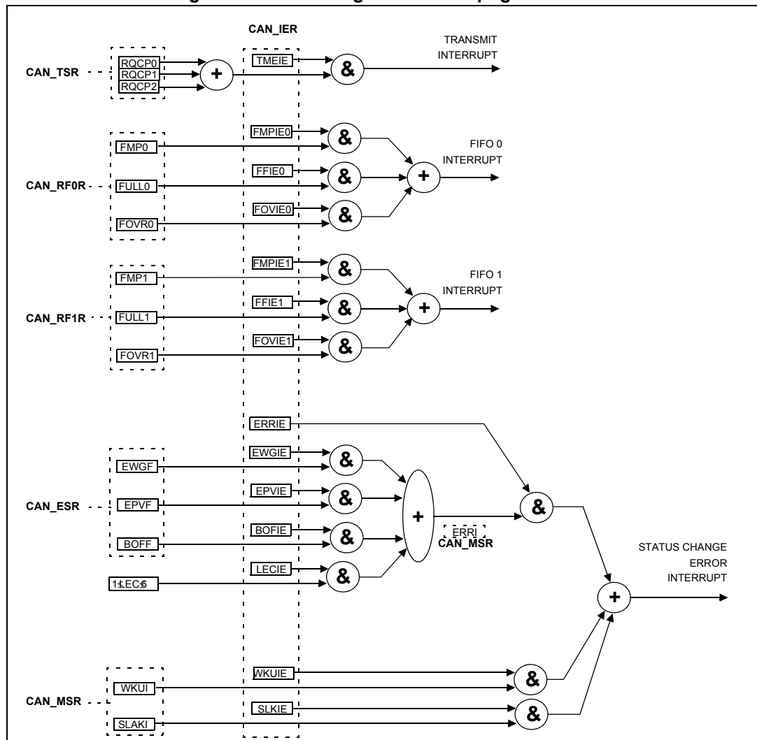
Figure 311. Event flags and interrupt generation
