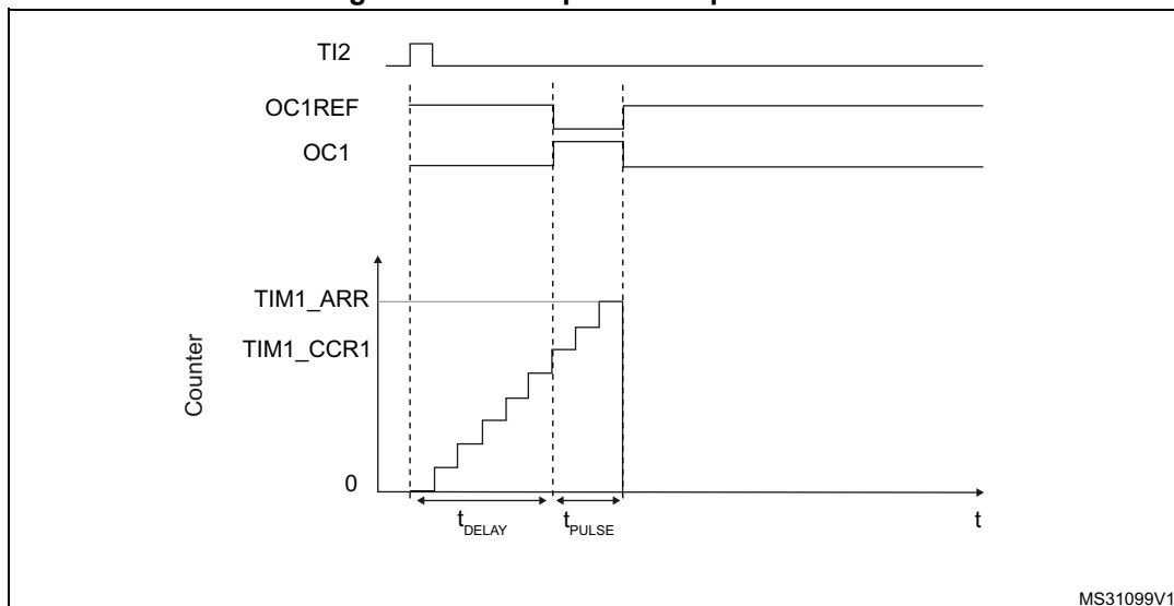
Figure 145. Example of one-pulse mode
