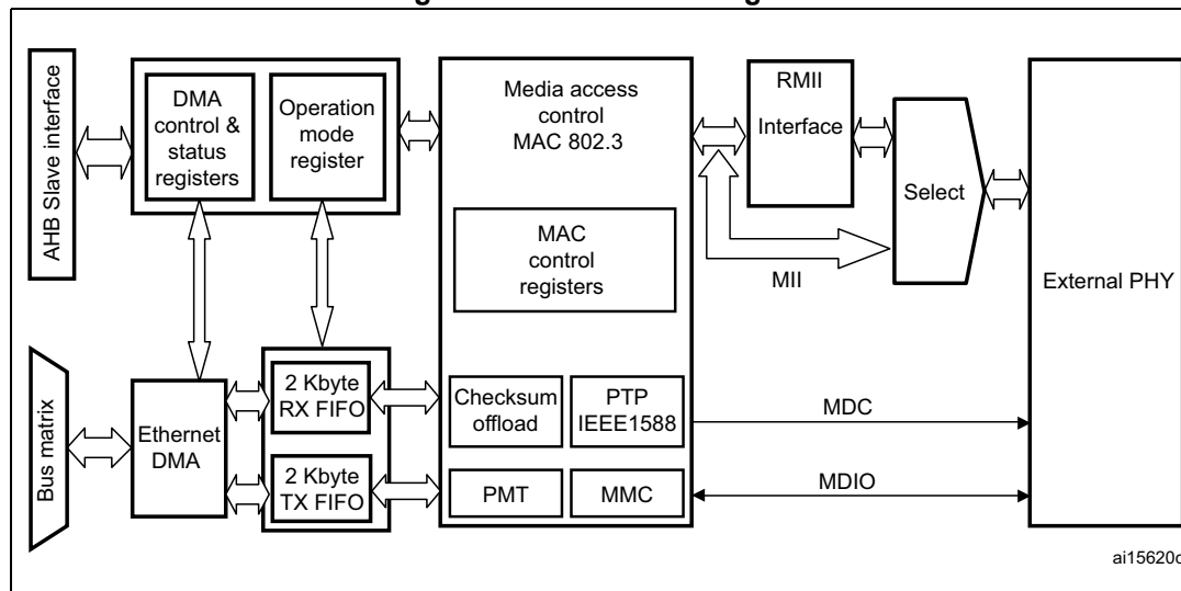
Figure 313. ETH block diagram
