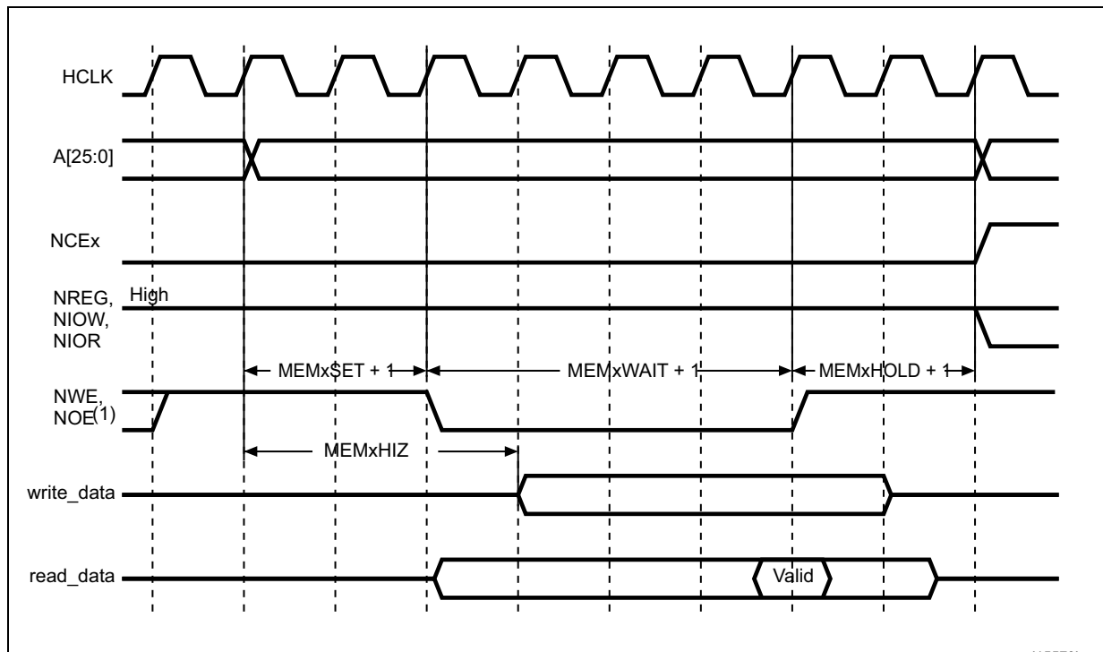
Figure 417. NAND/PC Card controller timing for common memory access
