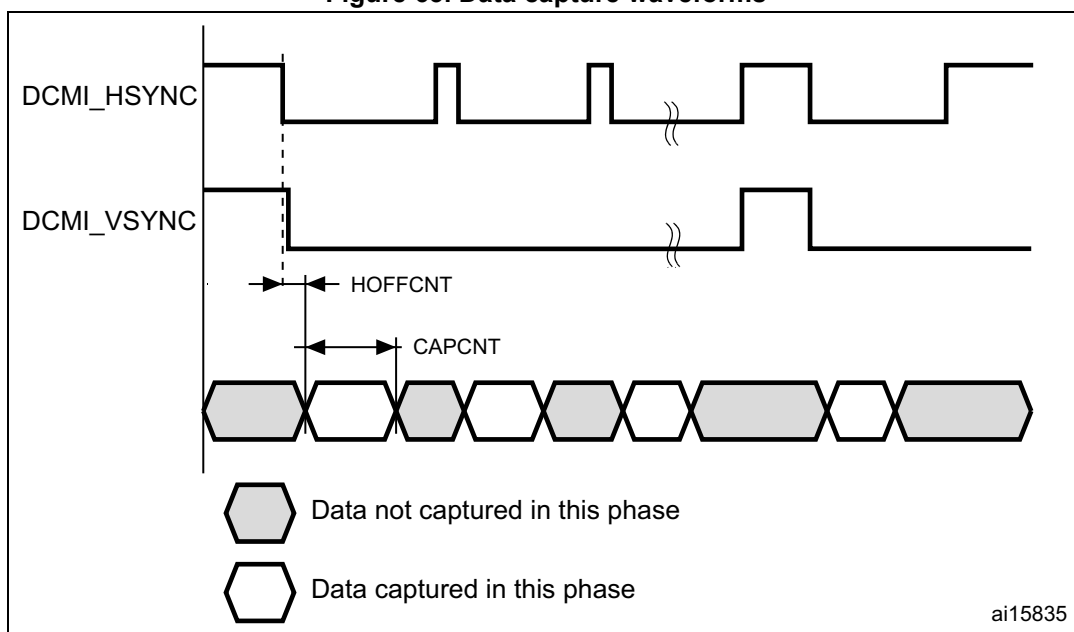
Figure 63. Data capture waveforms
