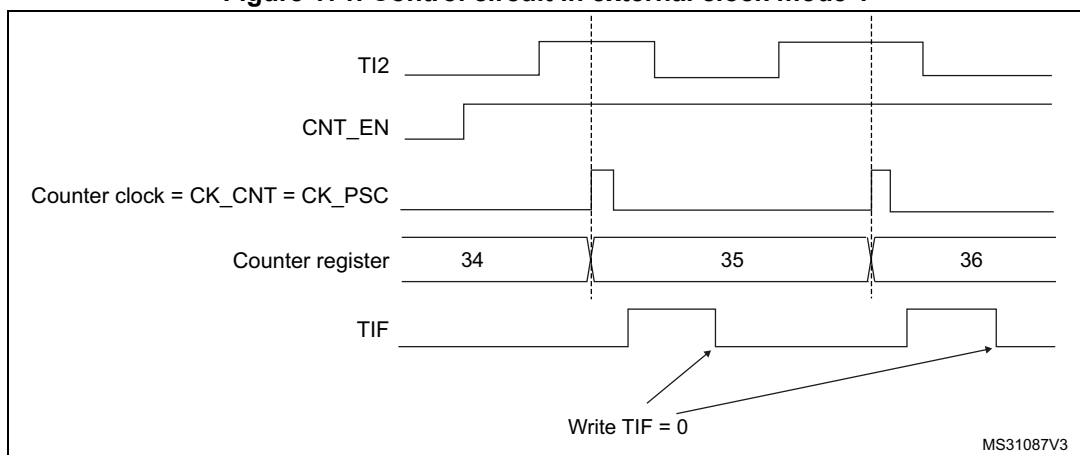
Figure 171. Control circuit in external clock mode 1
