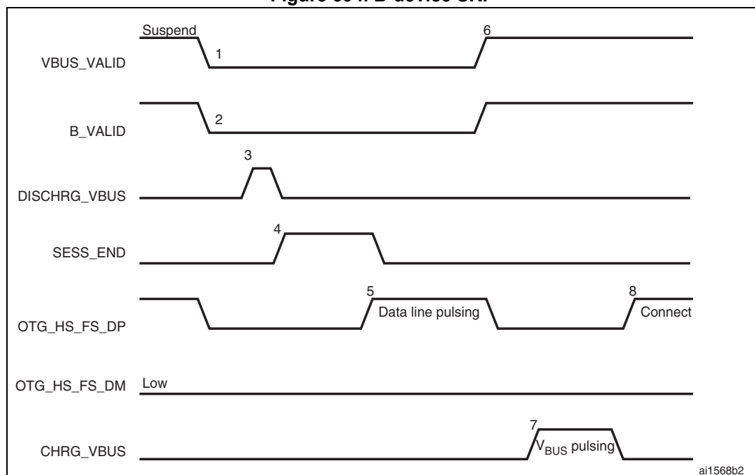
Figure 394. B-device SRP
