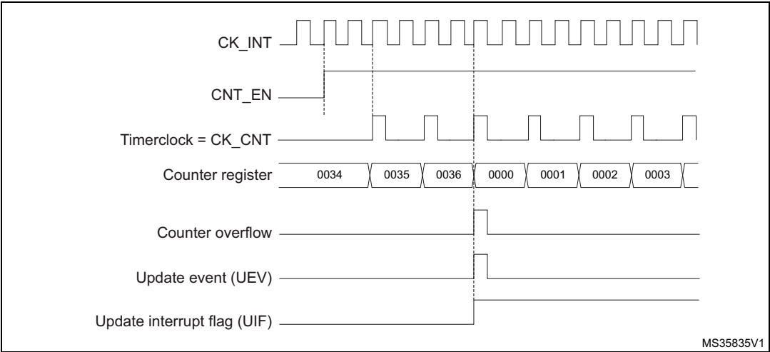
Figure 186. Counter timing diagram, internal clock divided by 2
