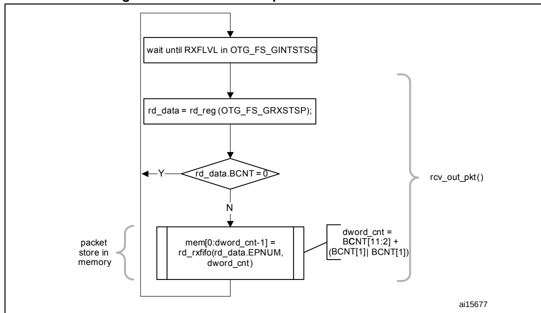
Figure 389. Receive FIFO packet read in slave mode
