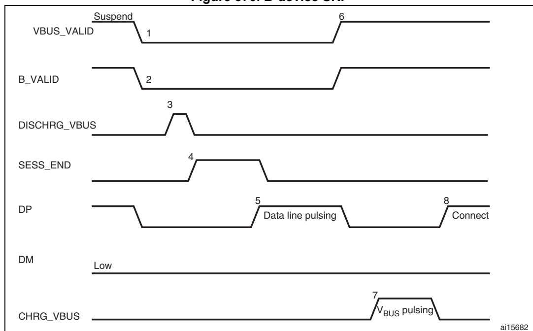
Figure 370. B-device SRP
