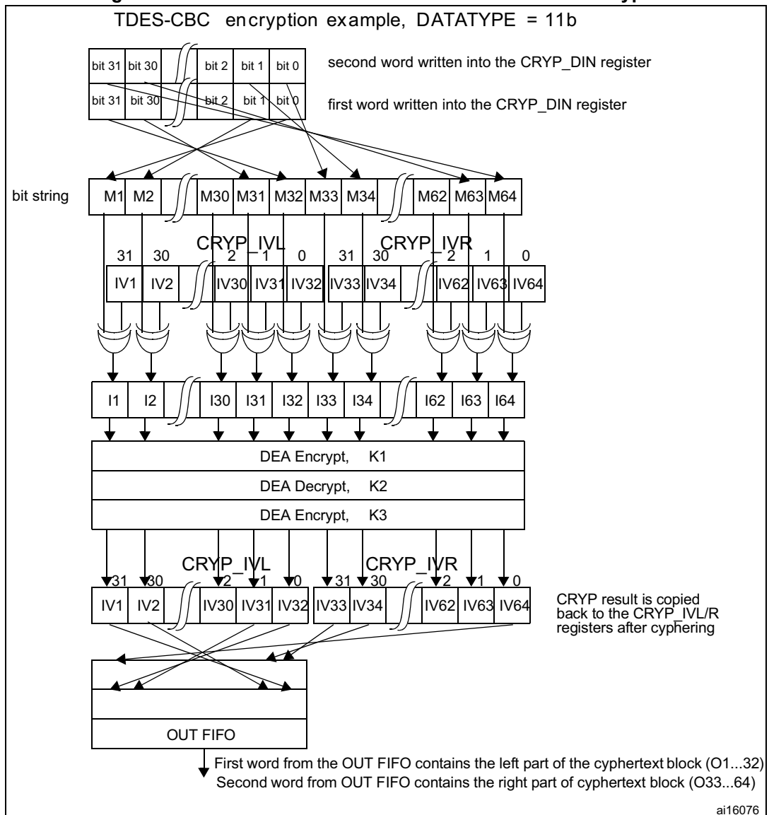
Figure 208. Initialization vectors use in the TDES-CBC encryption
