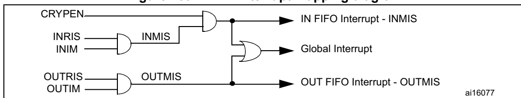
Figure 209. CRYP interrupt mapping diagram
