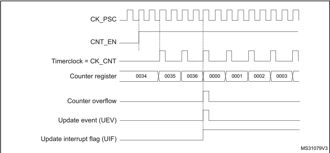
Figure 69. Counter timing diagram, internal clock divided by 2
