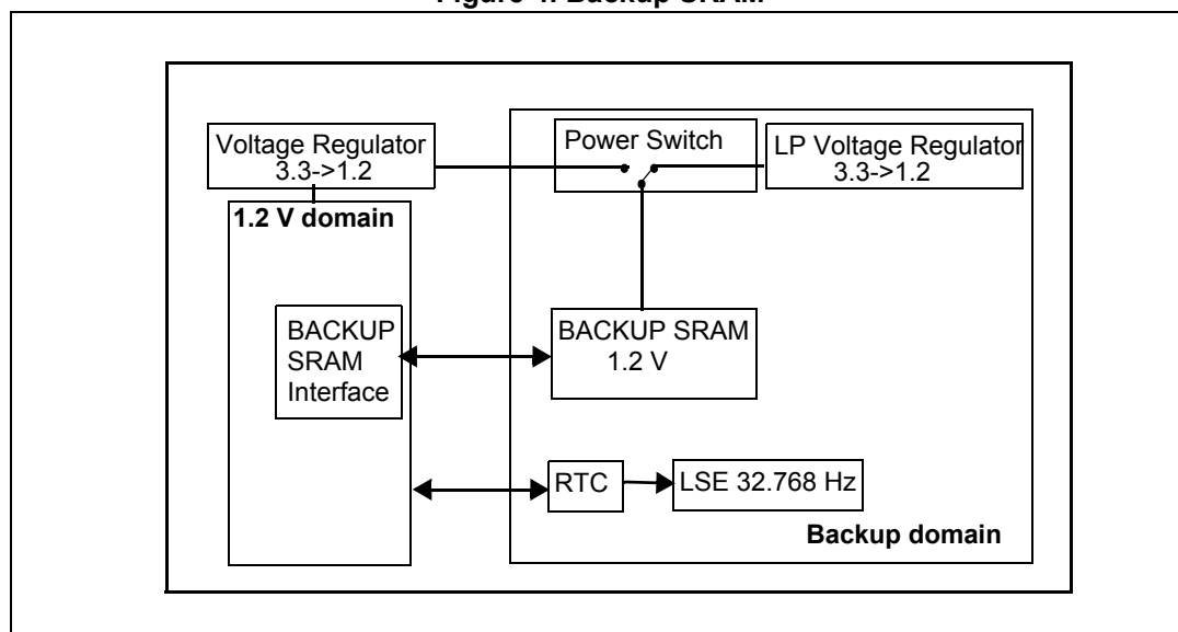
Figure 4. Backup SRAM
