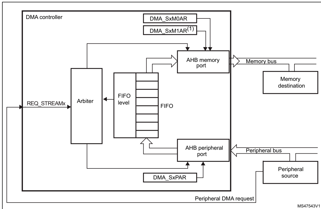
Figure 24. Peripheral-to-memory mode
