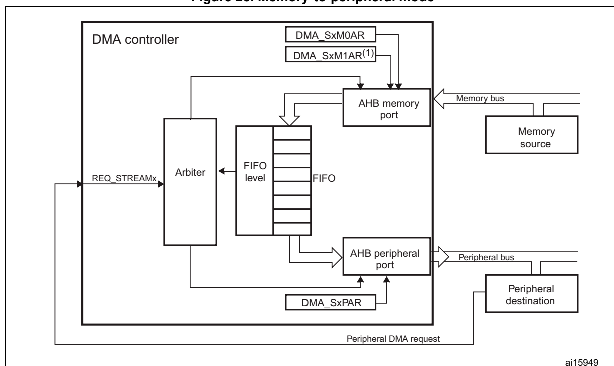
Figure 25. Memory-to-peripheral mode
