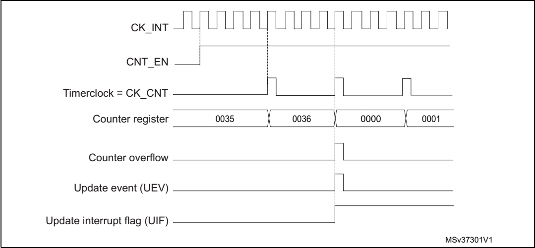
Figure 118. Counter timing diagram, internal clock divided by 4
