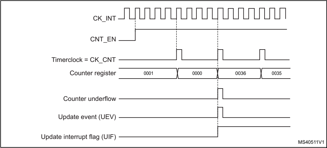
Figure 124. Counter timing diagram, internal clock divided by 4
