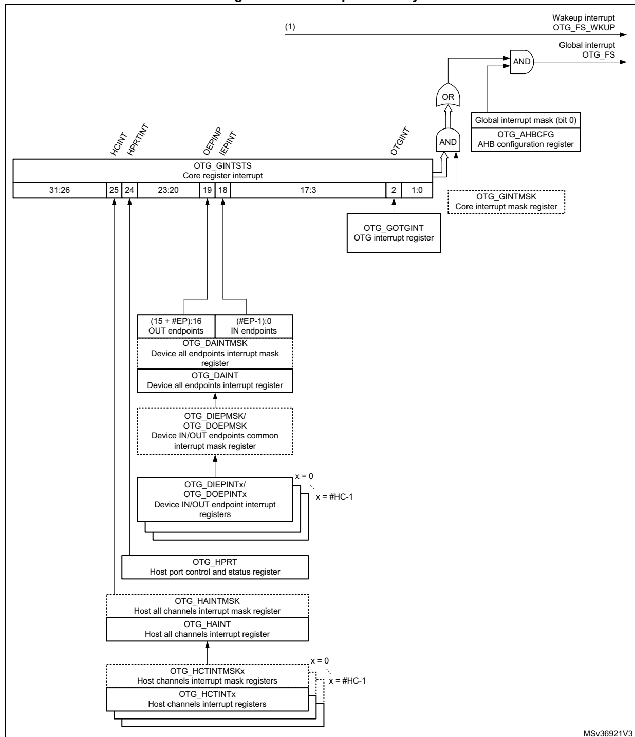
Figure 357. Interrupt hierarchy
