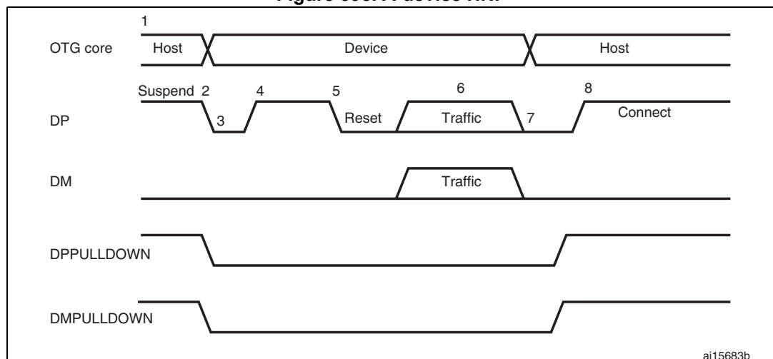
Figure 395. A-device HNP
