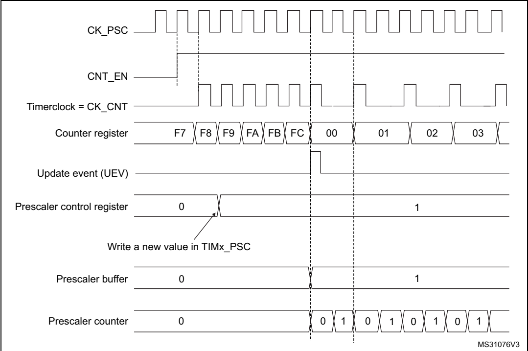
Figure 183. Counter timing diagram with prescaler division change from 1 to 2
