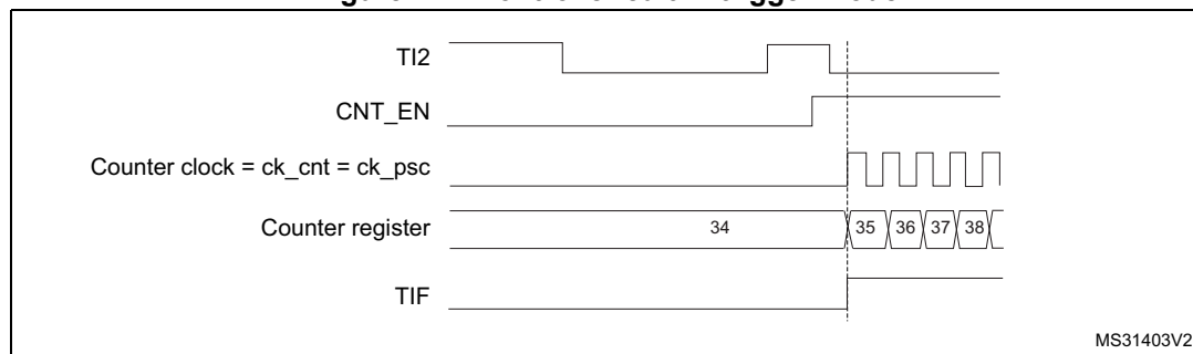
Figure 111. Control circuit in trigger mode
