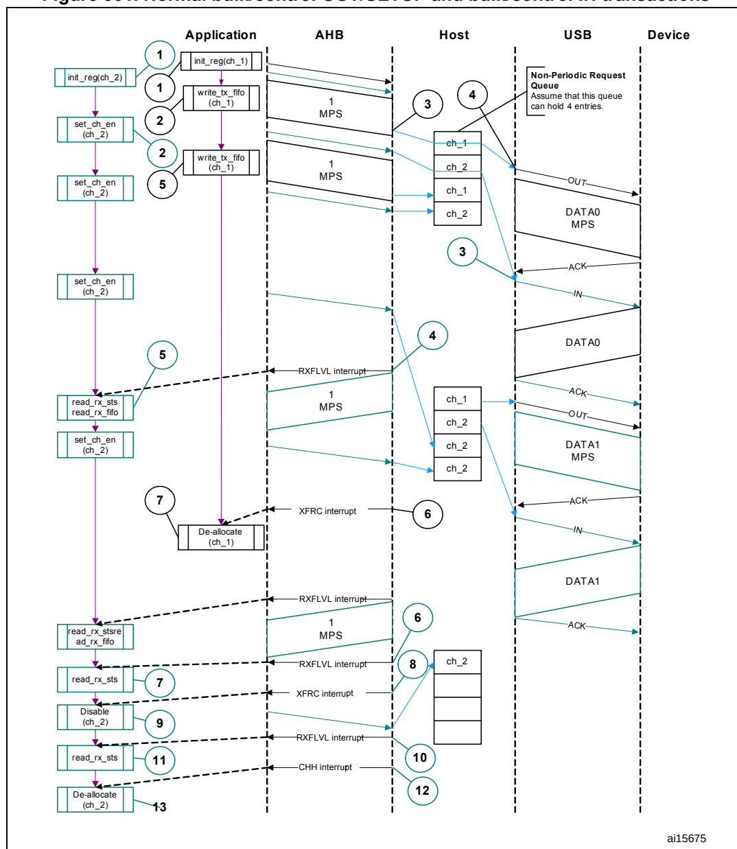
Figure 361. Normal bulk/control OUT/SETUP and bulk/control IN transactions
