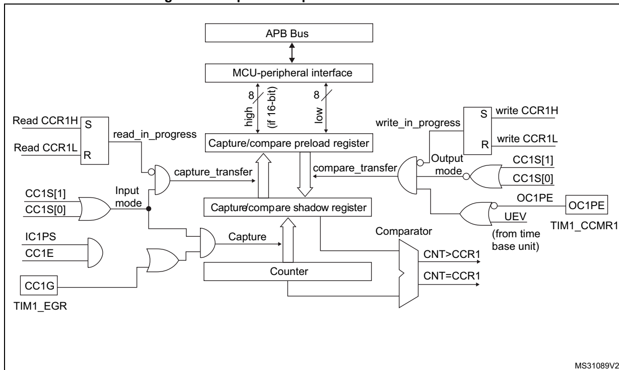
Figure 92. Capture/compare channel 1 main circuit
