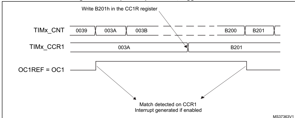
Figure 142. Output compare mode, toggle on OC1
