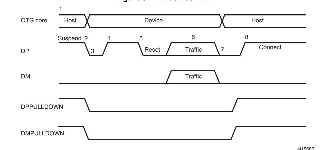
Figure 371. A-device HNP
