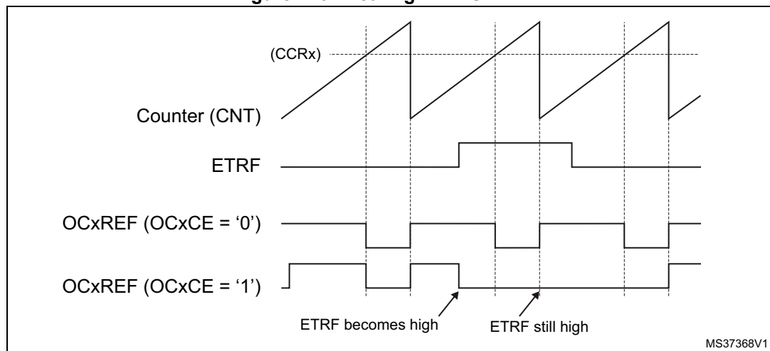
Figure 146. Clearing TIMx OCxREF
