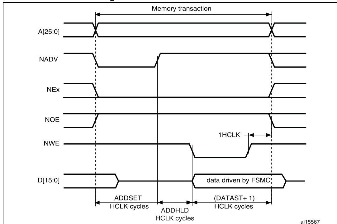
Figure 409. Mode D write accesses
