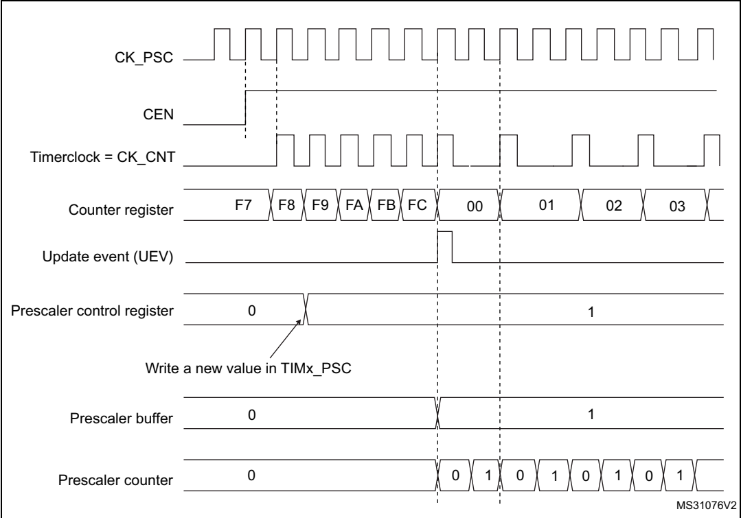
Figure 66. Counter timing diagram with prescaler division change from 1 to 2
