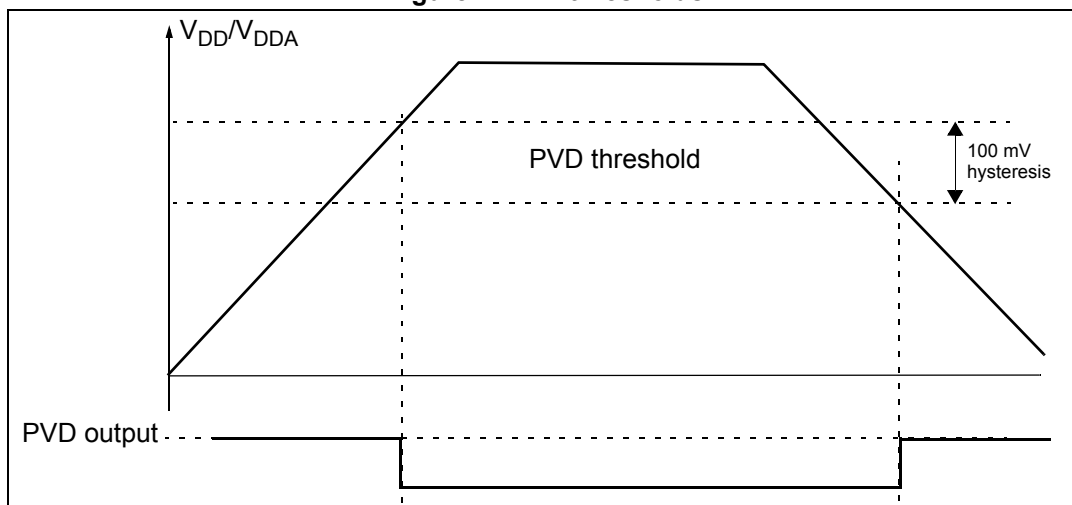
Figure 7. PVD thresholds
