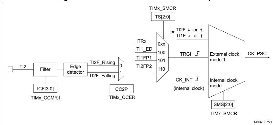
Figure 170. TI2 external clock connection example
