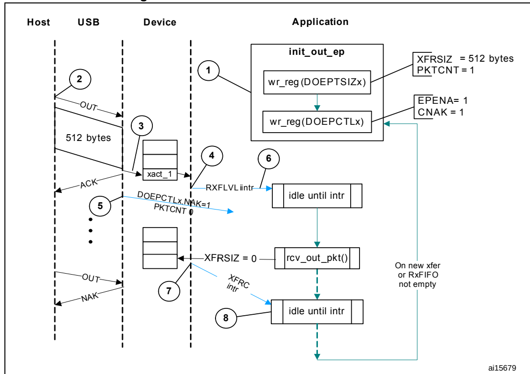
Figure 391. Slave mode bulk OUT transaction
