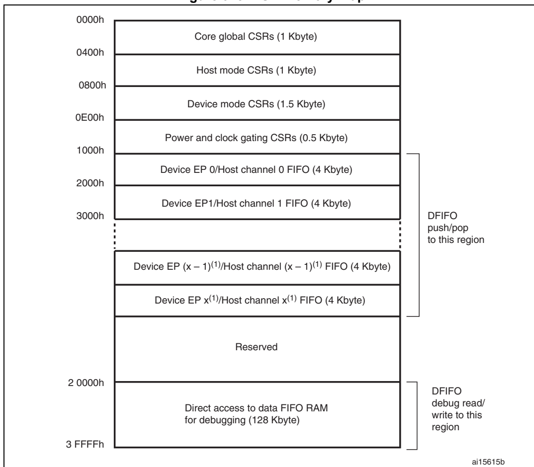
Figure 378. CSR memory map
