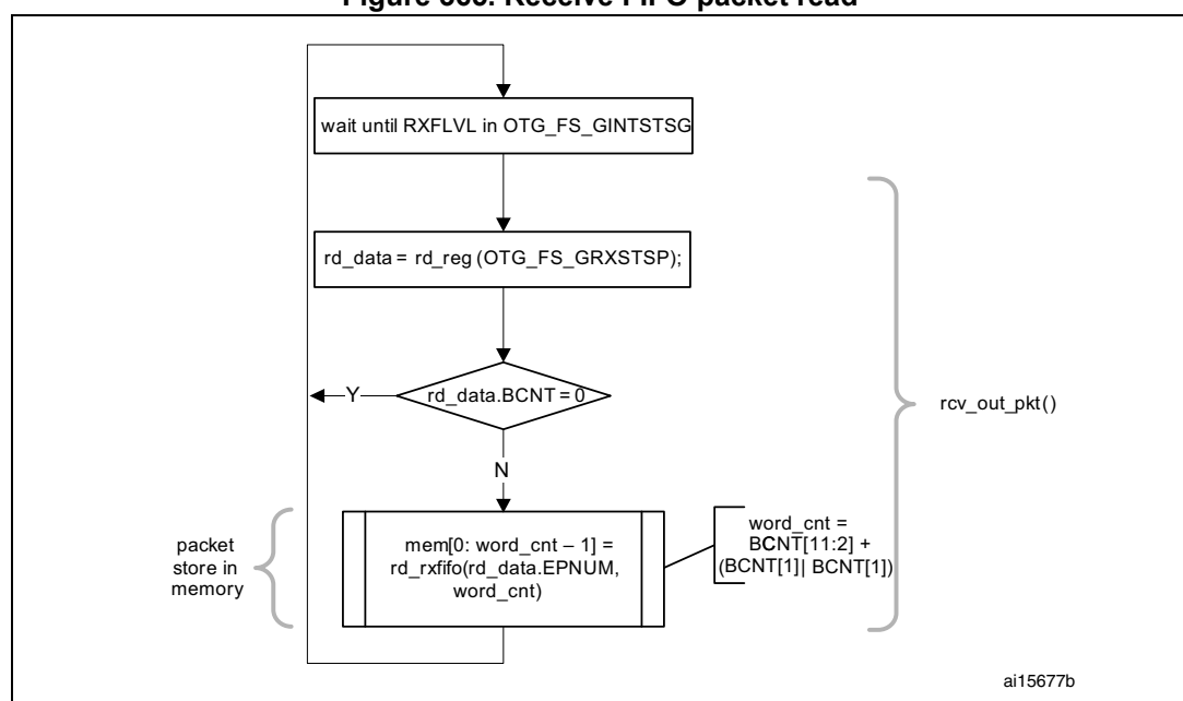
Figure 365. Receive FIFO packet read
