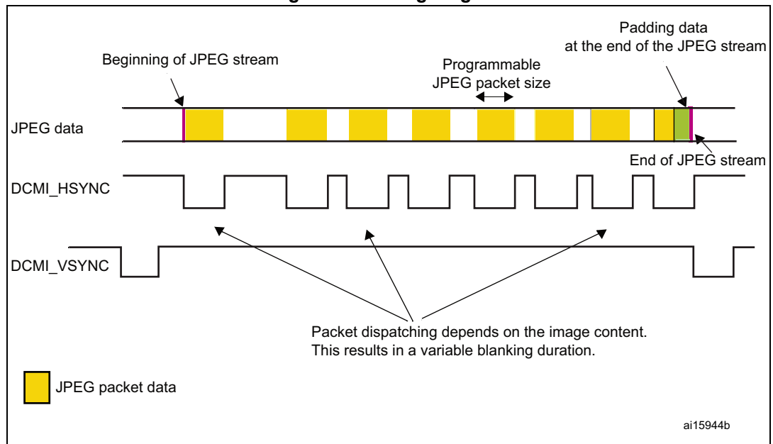
Figure 59. Timing diagram
