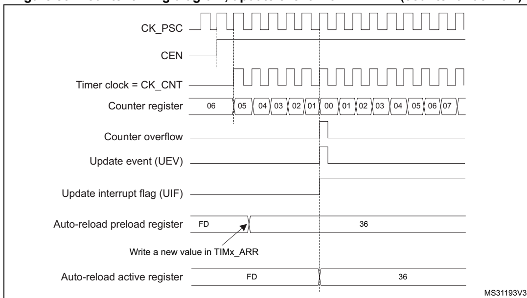
Figure 83. Counter timing diagram, update event with ARPE=1 (counter underflow)
