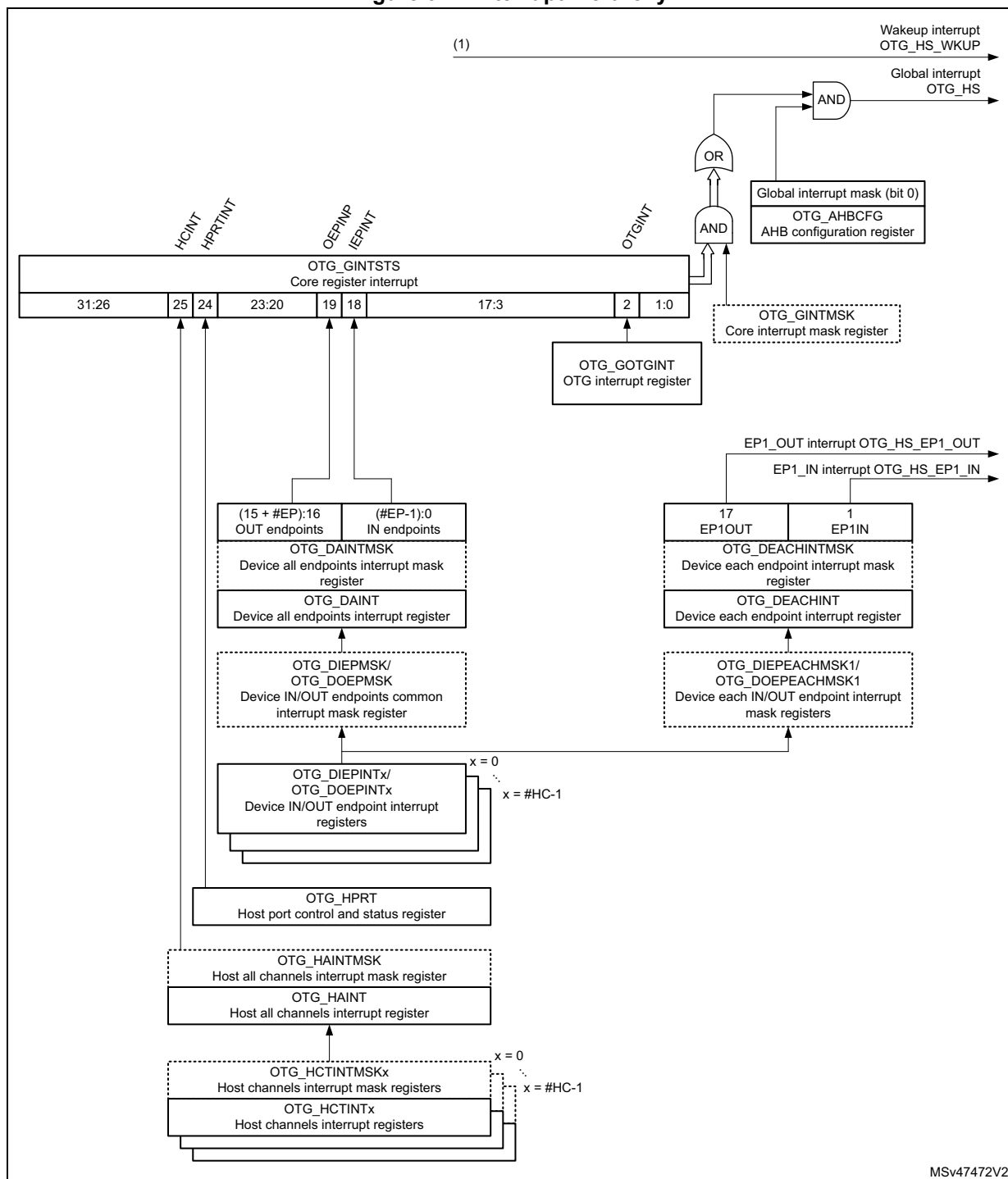
Figure 377. Interrupt hierarchy
