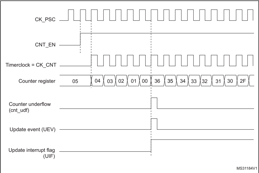
Figure 74. Counter timing diagram, internal clock divided by 1
