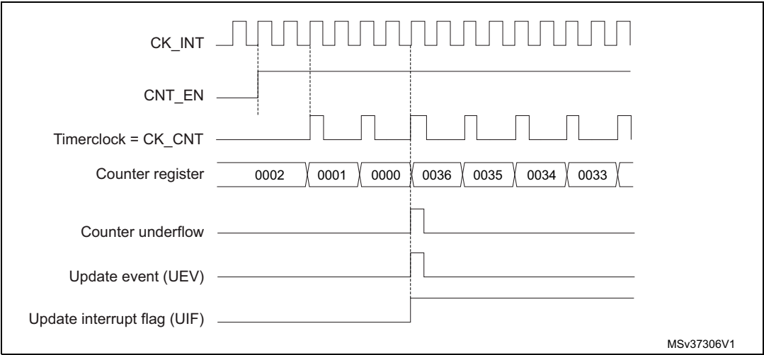
Figure 123. Counter timing diagram, internal clock divided by 2
