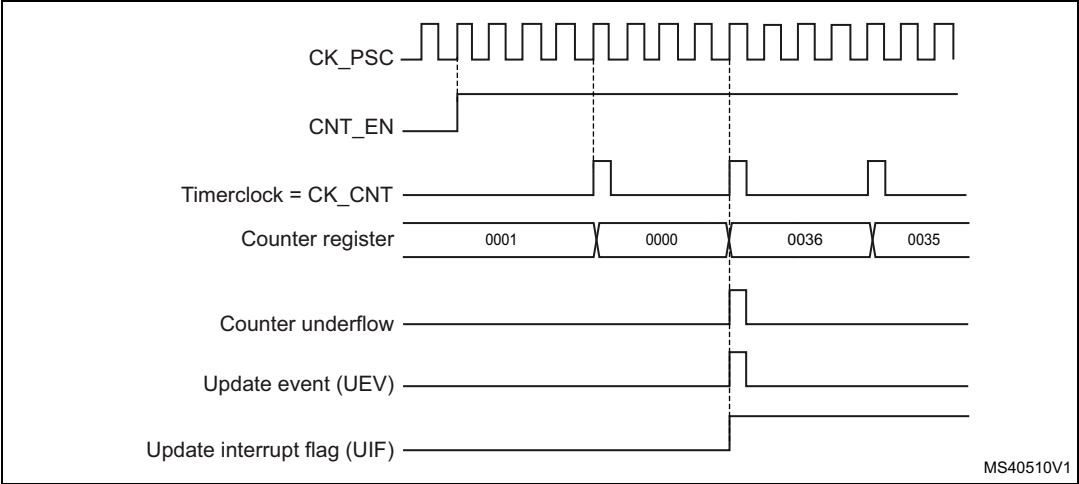
Figure 76. Counter timing diagram, internal clock divided by 4
