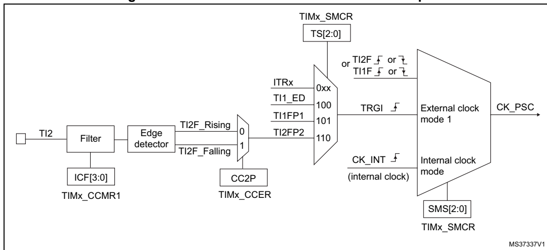
Figure 157. TI2 external clock connection example
