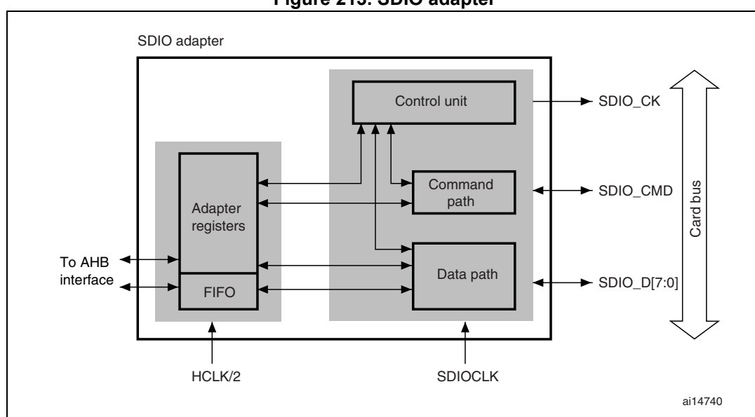
Figure 213. SDIO adapter
