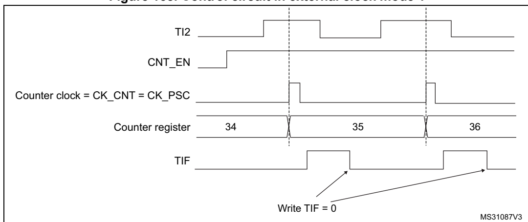
Figure 158. Control circuit in external clock mode 1
