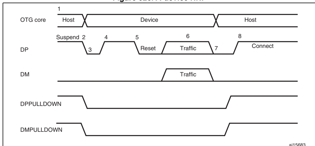
Figure 325. A-device HNP
