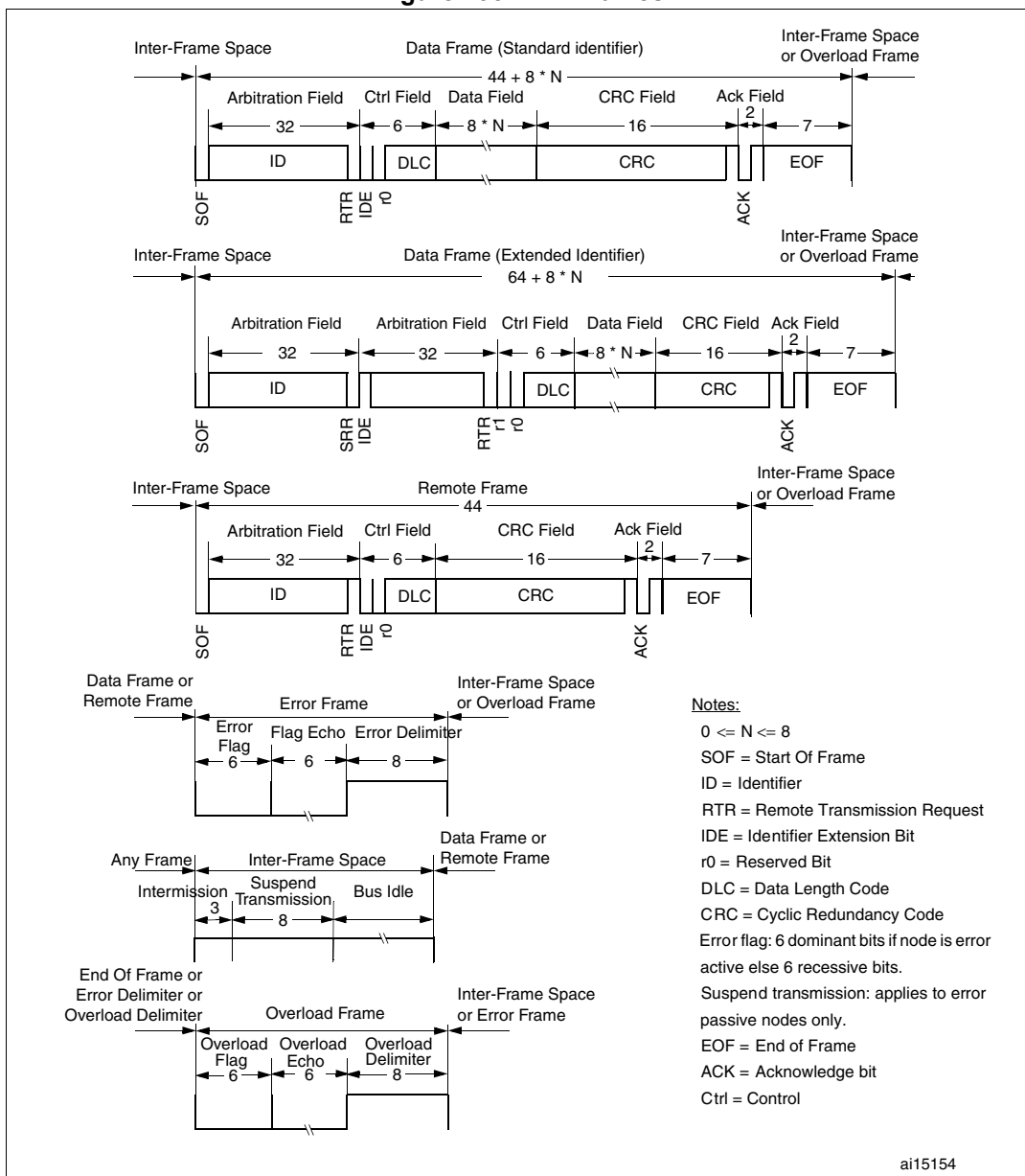
Figure 235. CAN frames
