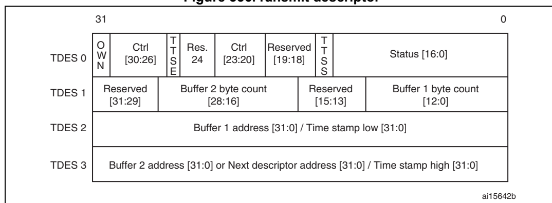
Figure 356. ransmit descriptor
