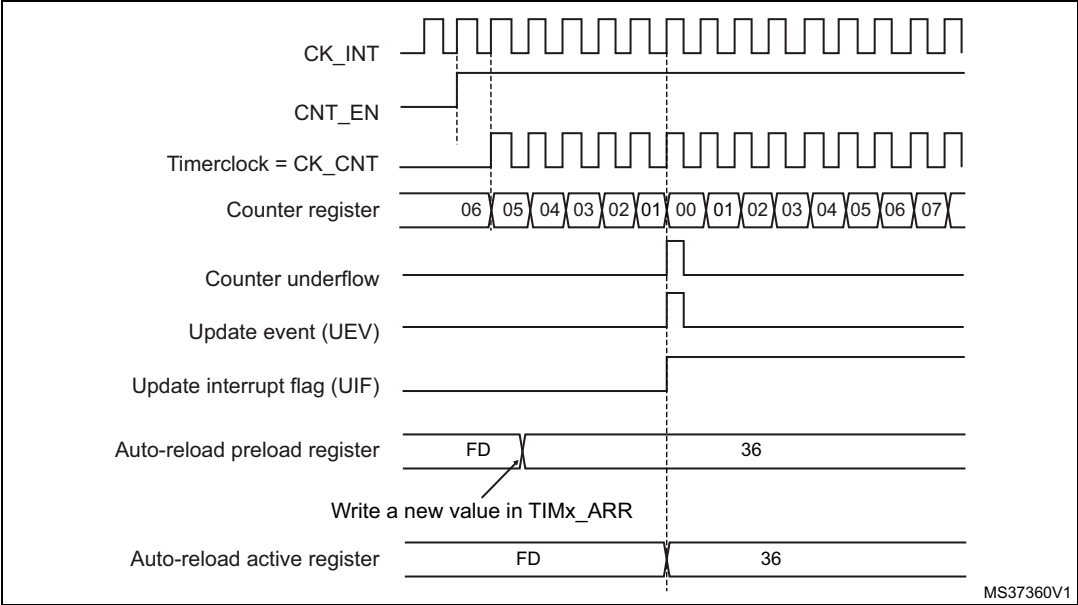
Figure 118. Counter timing diagram, Update event with ARPE=1 (counter underflow)
