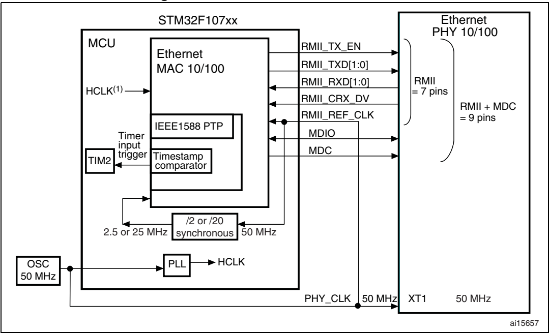
Figure 54. RMII with a 50 MHz oscillator
