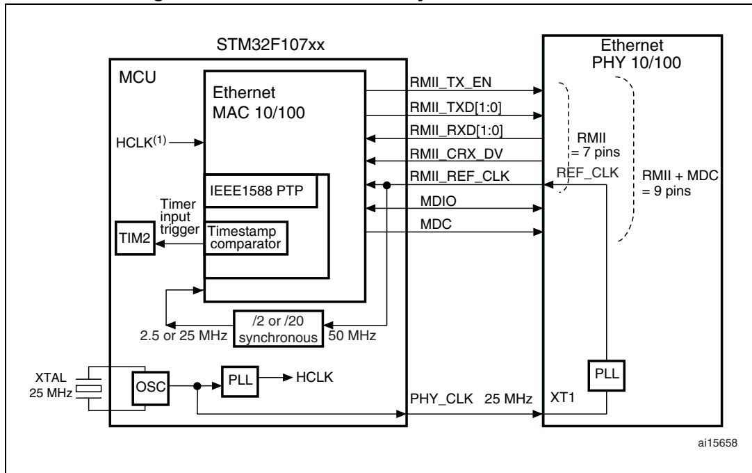
Figure 55. RMI with a 25 MHz crystal and PHY with PLL
