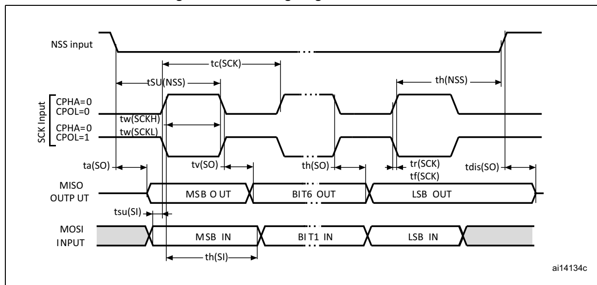
Figure 47. SPI timing diagram - slave mode and CPHA = 0
