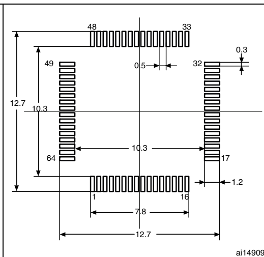
Figure 67. Recommended footprint (1)(2)
