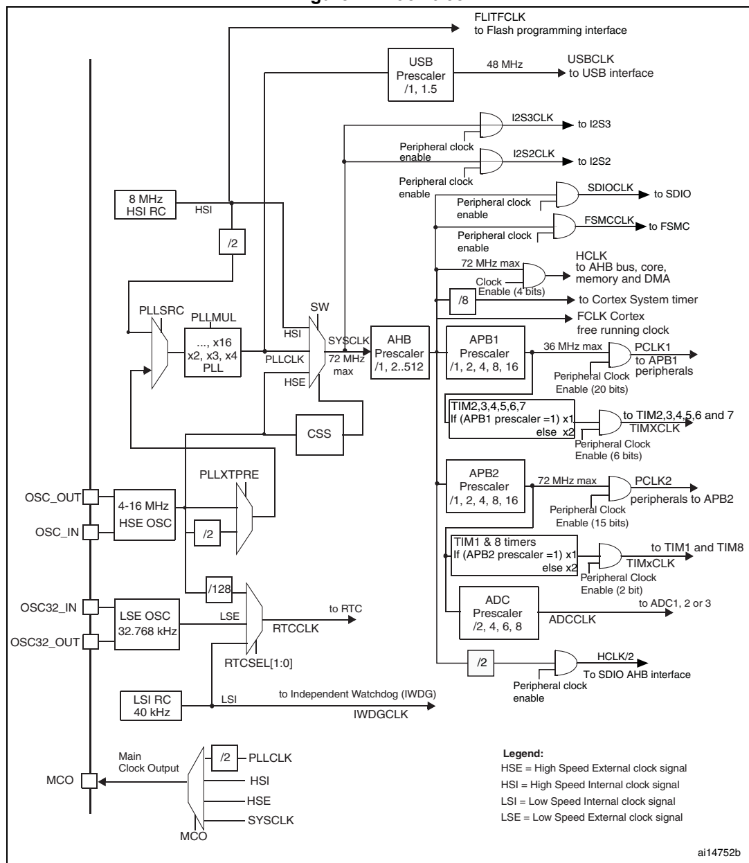
Figure 2. Clock tree
