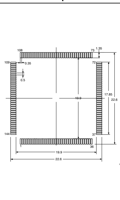
Figure 39. Recommended footprint
