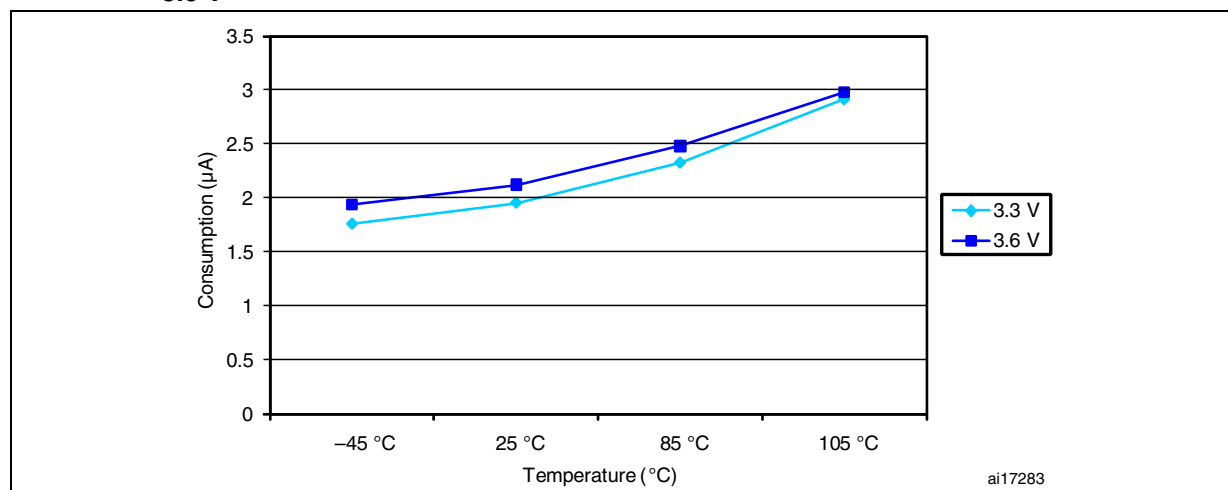
Figure 16. Typical current consumption in Standby mode versus temperature at V_{DD} = 3.3\text{ V} and 3.6\text{ V}
