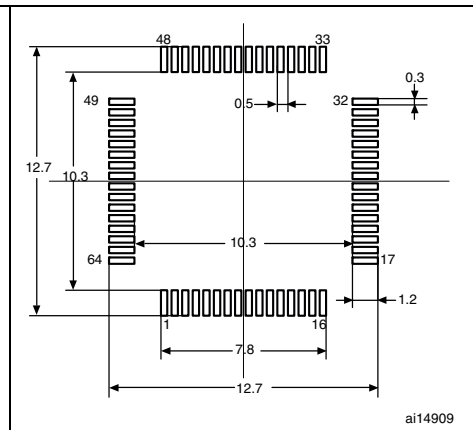
Figure 39. Recommended footprint (1)(2)
