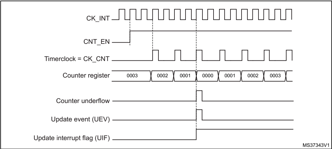
Figure 103. Counter timing diagram, internal clock divided by 2
