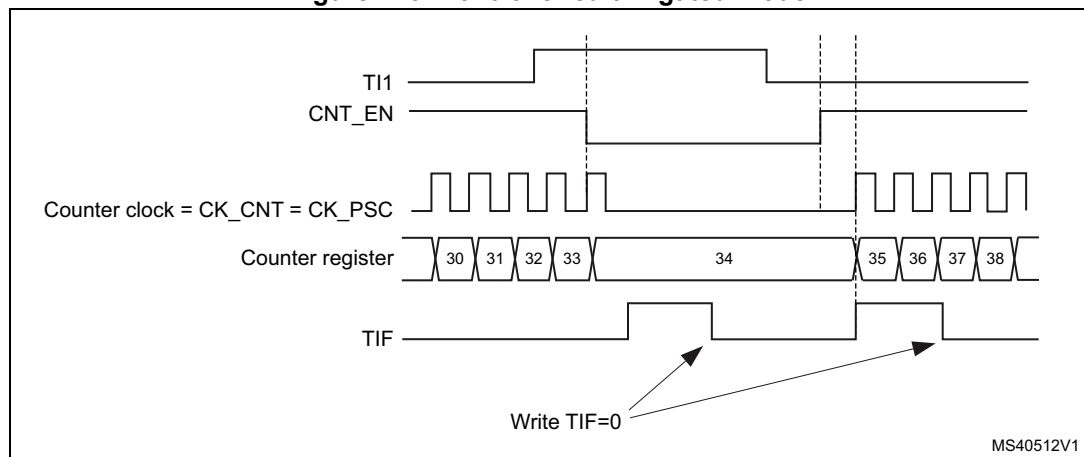
Figure 125. Control circuit in gated mode
