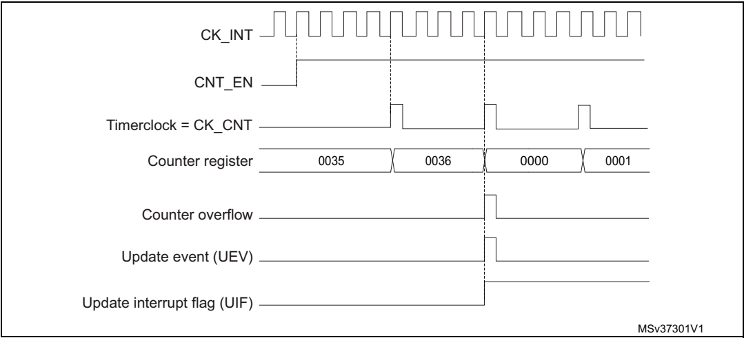
Figure 192. Counter timing diagram, internal clock divided by N
