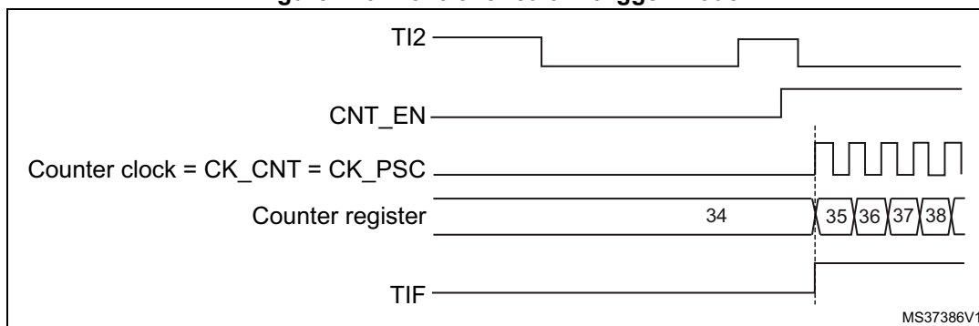
Figure 126. Control circuit in trigger mode
