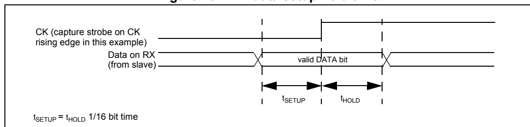
Figure 257. RX data setup/hold time
