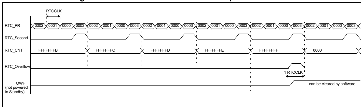
Figure 198. RTC Overflow waveform example with PR=0003
