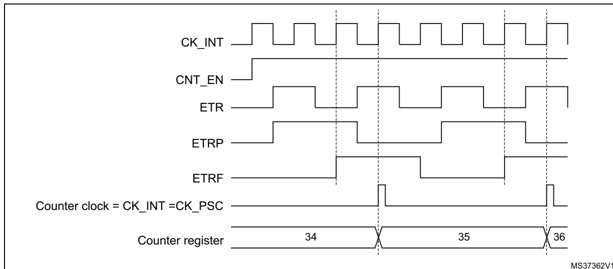
Figure 112. Control circuit in external clock mode 2
