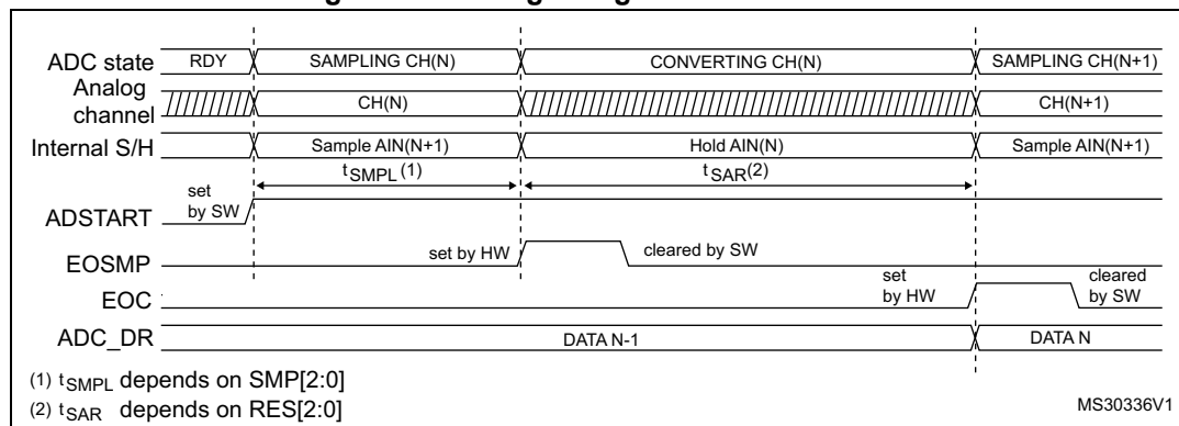
Figure 30. Analog to digital conversion time
