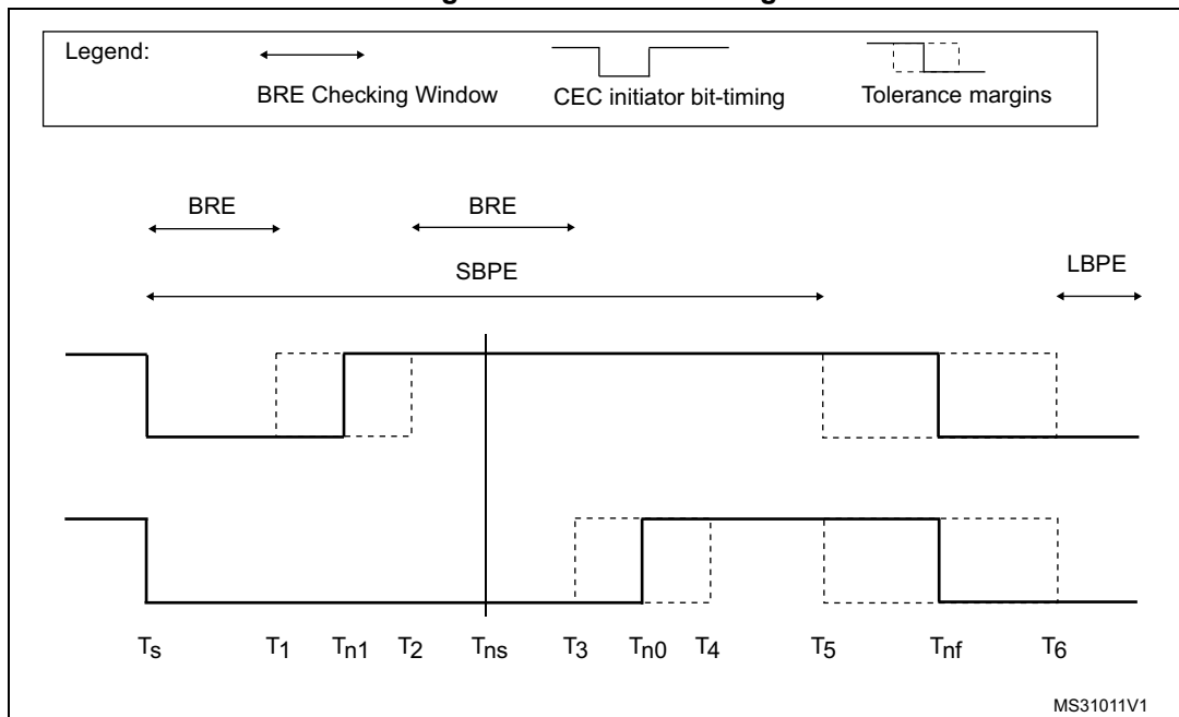
Figure 333. Error handling
