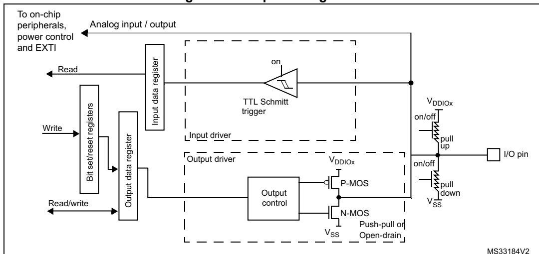
Figure 18. Output configuration
