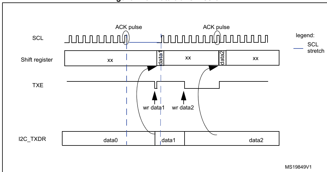
Figure 219. Data transmission
