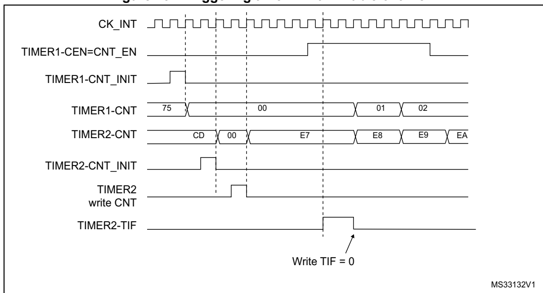
Figure 151. Triggering timer 2 with Enable of timer 1
