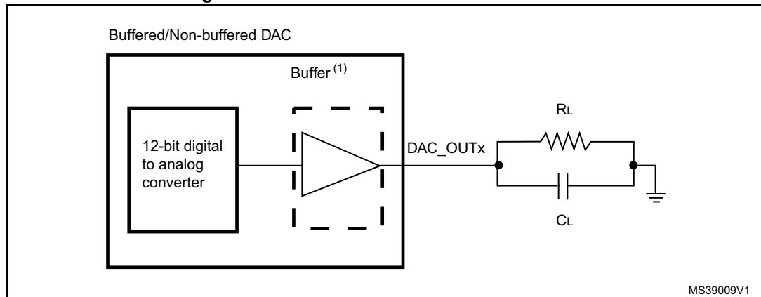
Figure 28. 12-bit buffered / non-buffered DAC
