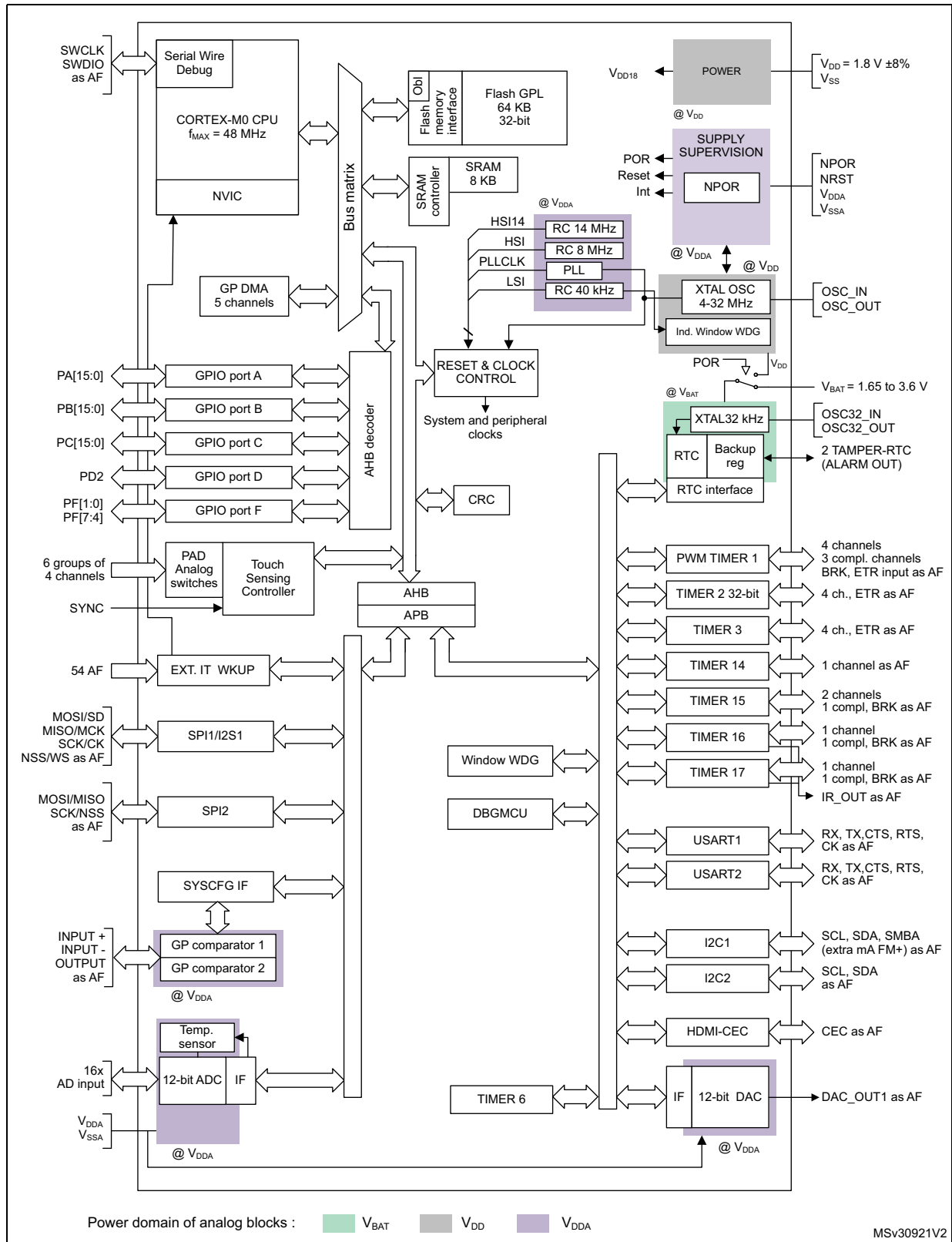
Figure 1. Block diagram
