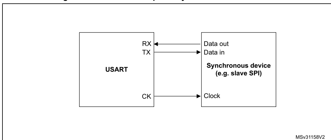
Figure 235. USART example of synchronous transmission
