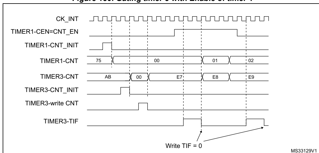
Figure 130. Gating timer 3 with Enable of timer 1
