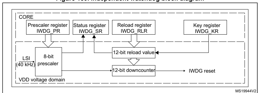
Figure 189. Independent watchdog block diagram
