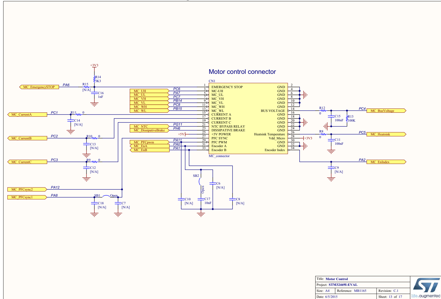
Figure 35. Motor control
