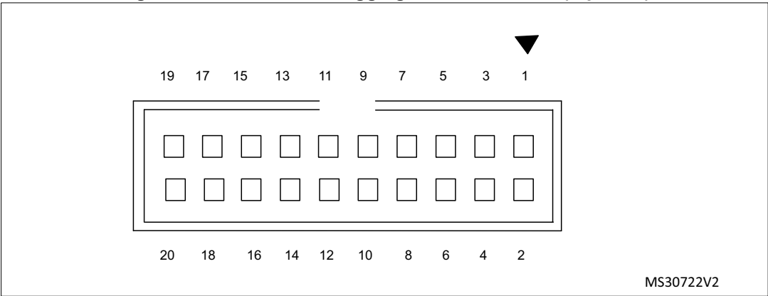
Figure 14. ETM trace debugging connector CN12 (top view)
