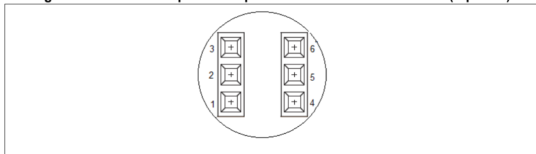
Figure 22. MEMS microphone coupon connectors CN25 and CN28 (top view)
