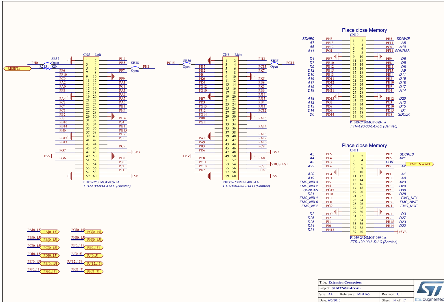
Figure 36. Extension connectors
