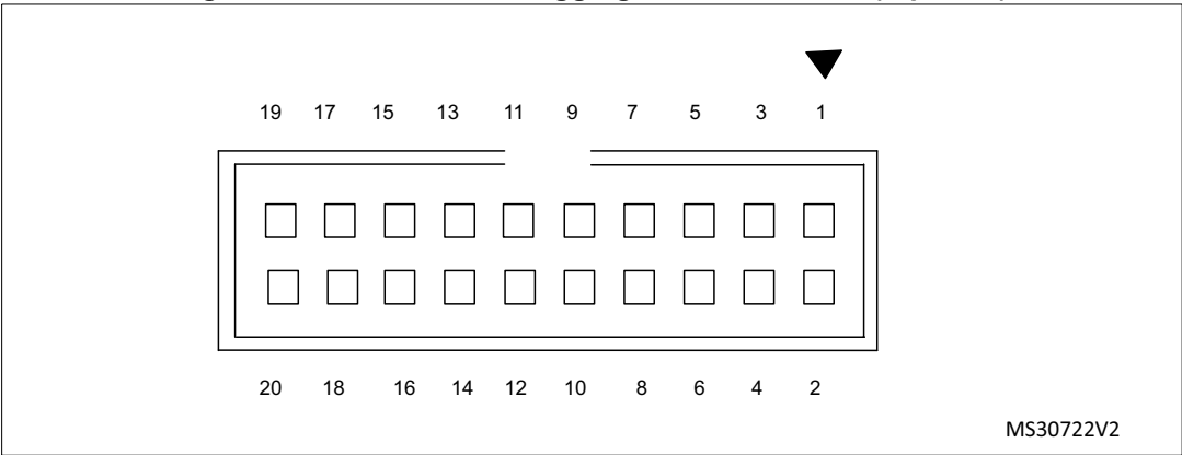
Figure 17. JTAG/SWD debugging connector CN15 (top view)
