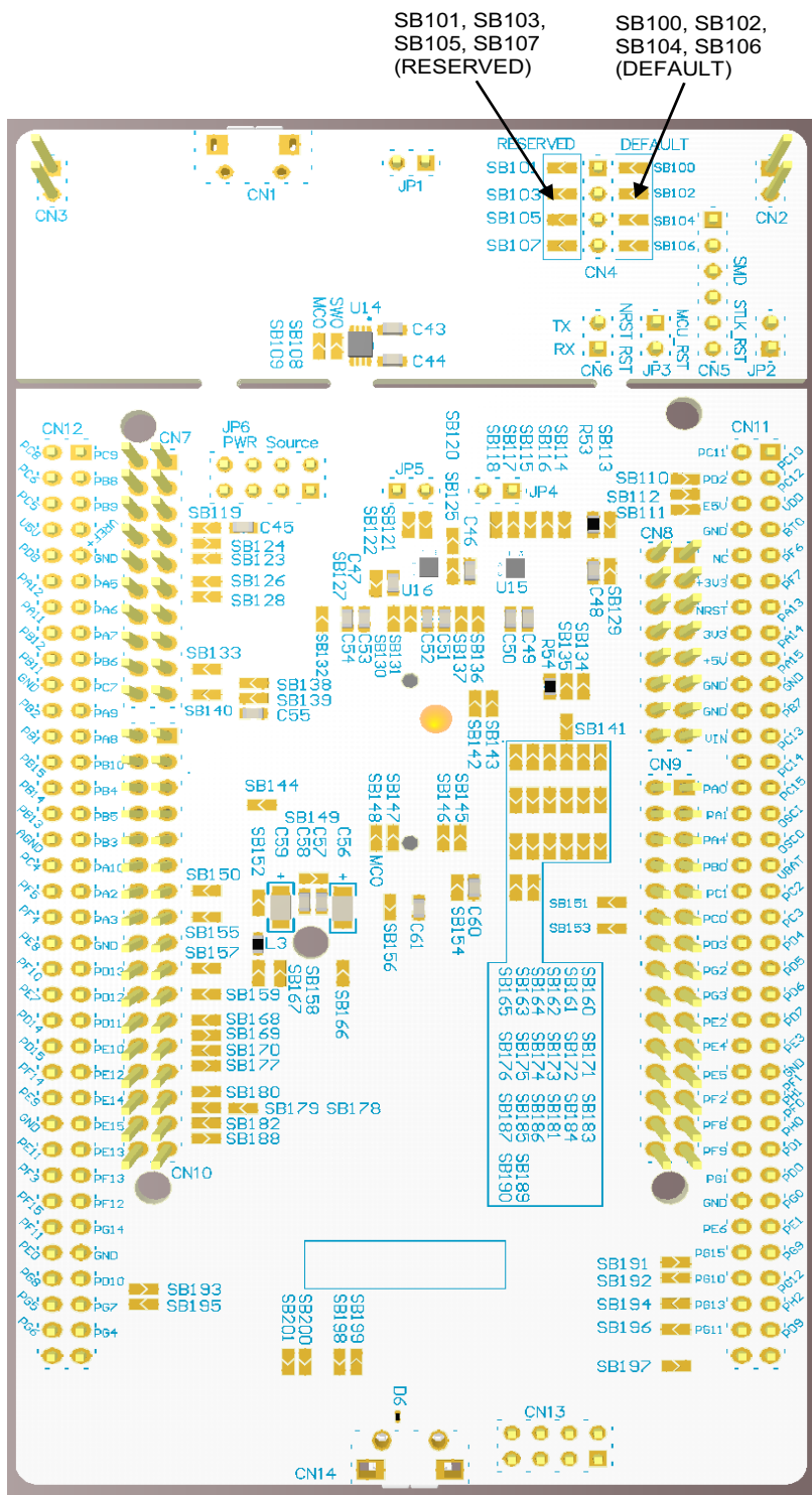
Figure 5. STM32 Nucleo-144 board bottom layout
