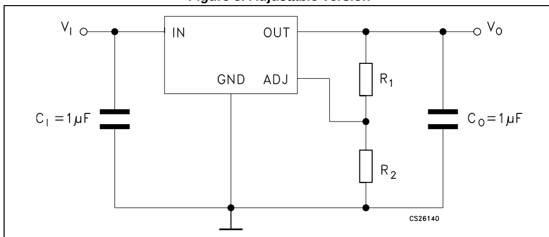
Figure 5. Adjustable version
