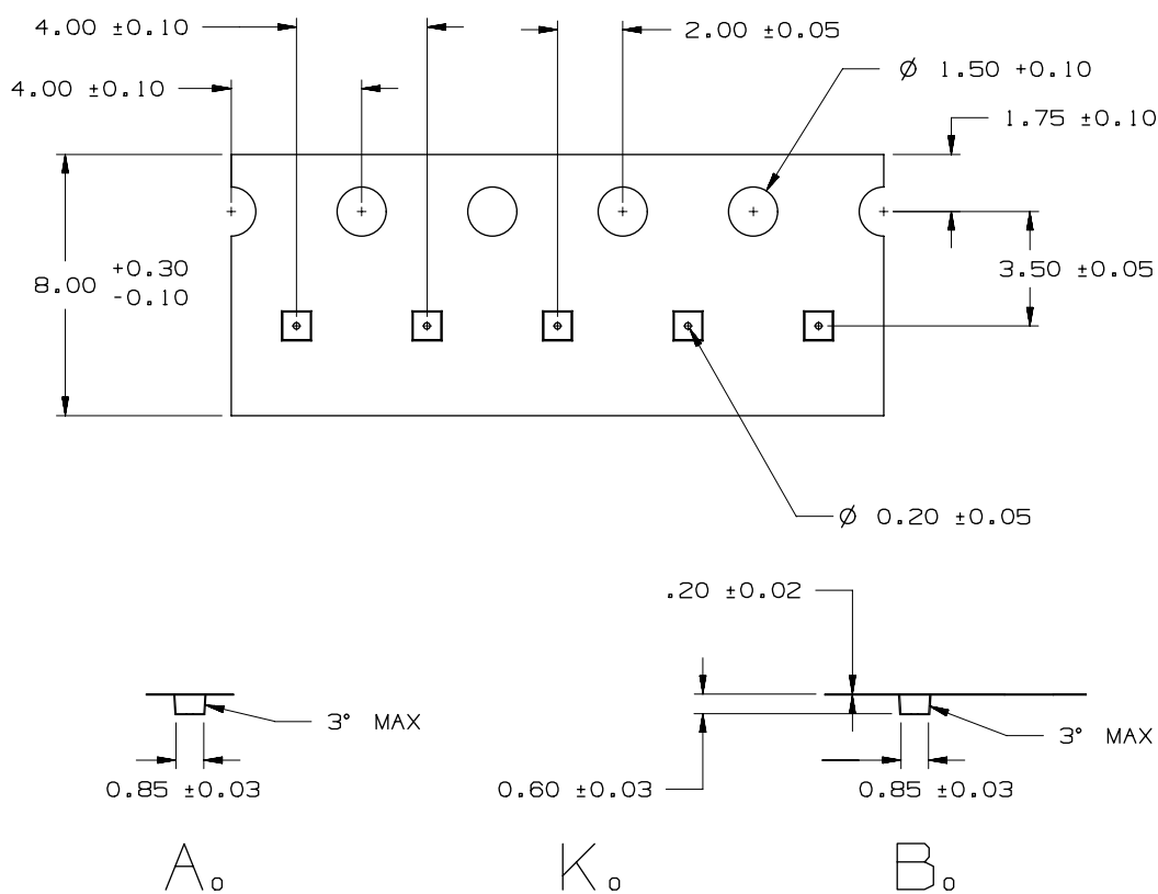
Figure 41. Flip-Chip4 tape outline
