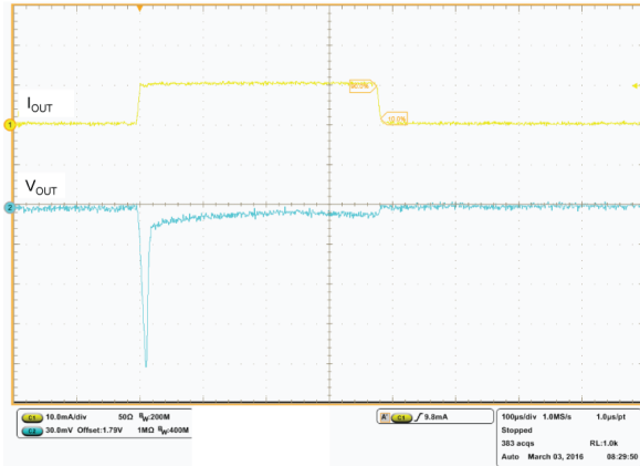
Figure 28. Load transient
