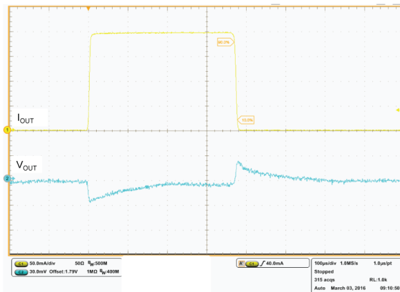
Figure 30. Load transient ( V_{OUT} = 1.8 V )
