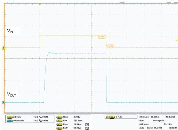
Figure 32. Startup transient
