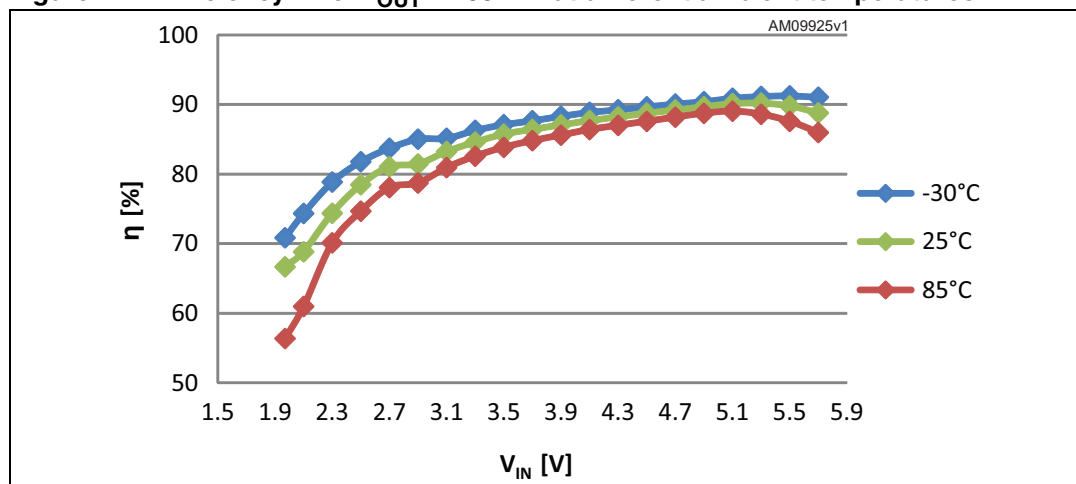
Figure 7. Efficiency when I_{OUT} = 100 mA at different ambient temperatures
