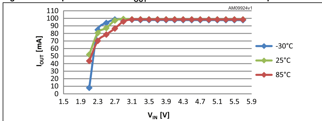
Figure 6. Output current when V_{OUT} = 8.5 V at different ambient temperatures
