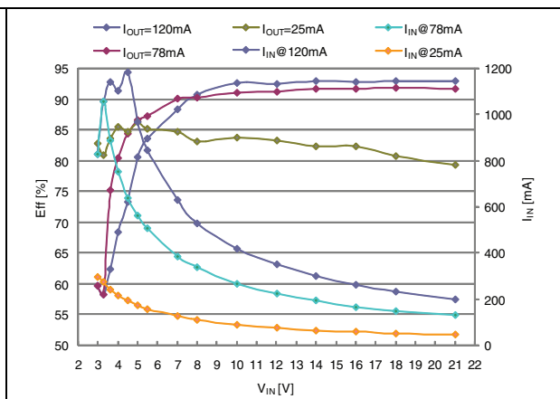
Figure 10. Application eff. vs. V_{IN} , matrix 4 x 10 LEDs
