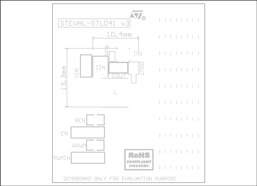
Figure 6. Top overlay
