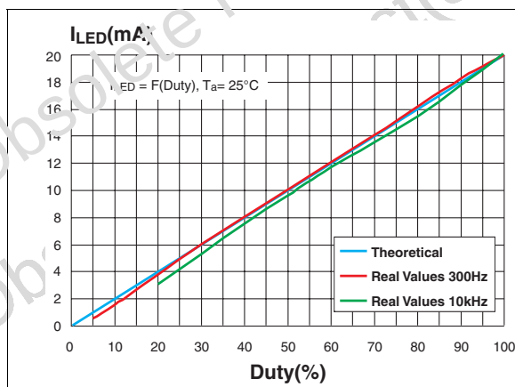
Figure 14. I_{LED} versus duty cycle
