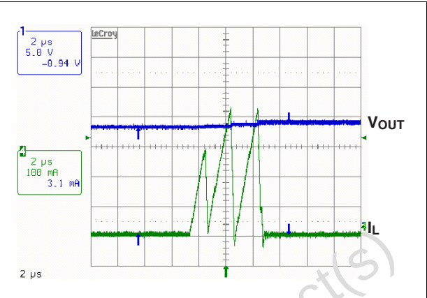
Figure 17. Overvoltage protection
