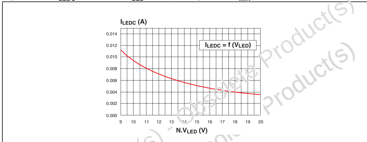
Figure 23. I_{LED} current vs N.V_{LED} corresponding at the DC_{MIN}
