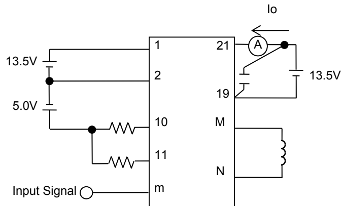
Figure 19 ISD Measurement Circuit
