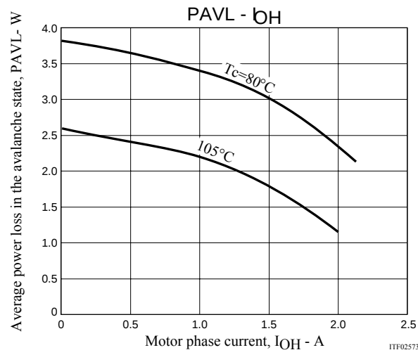
Figure 3 Allowable Loss Range, PAVL-I_{OH} During STK672-630C-E Avalanche Operations
