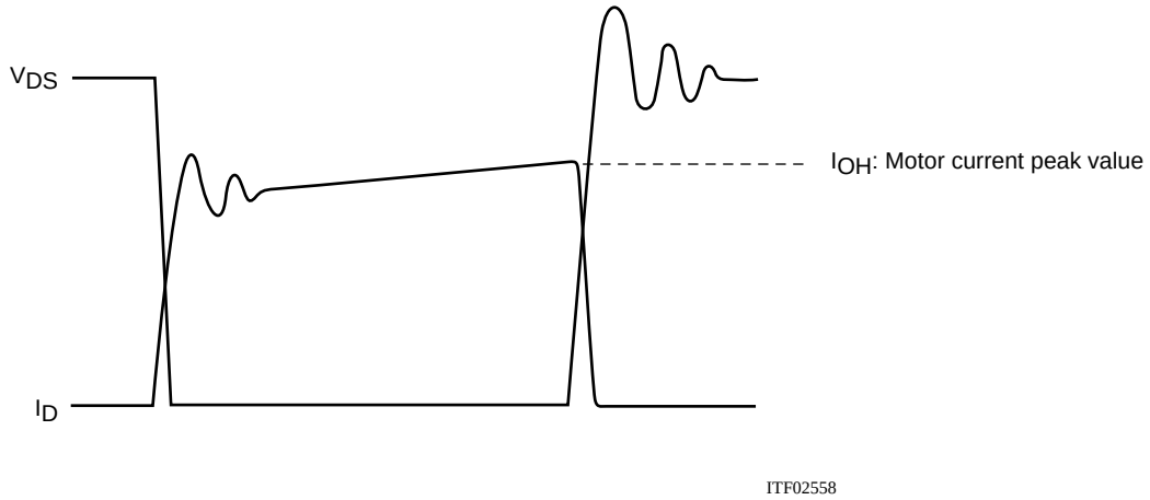
Figure 2 Output Current, I_D , and Voltage, V_{DS} , Waveforms 2 of the STK672-410C-E when Driving a 2-Phase Stepping Motor with Constant Current Chopping
