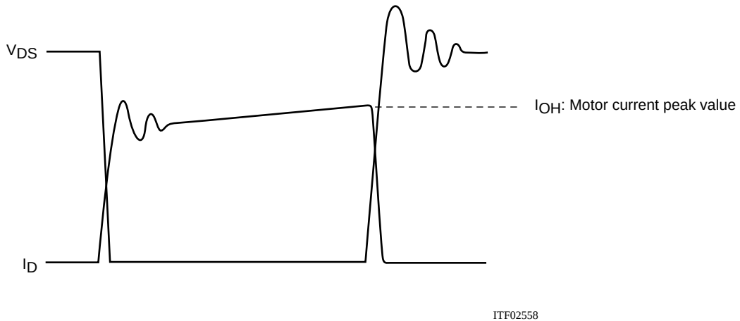
Figure 2 Output Current, I_D , and Voltage, V_{DS} , Waveforms 2 of the STK672-400C-E when Driving a 2-Phase Stepping Motor with Constant Current Chopping
