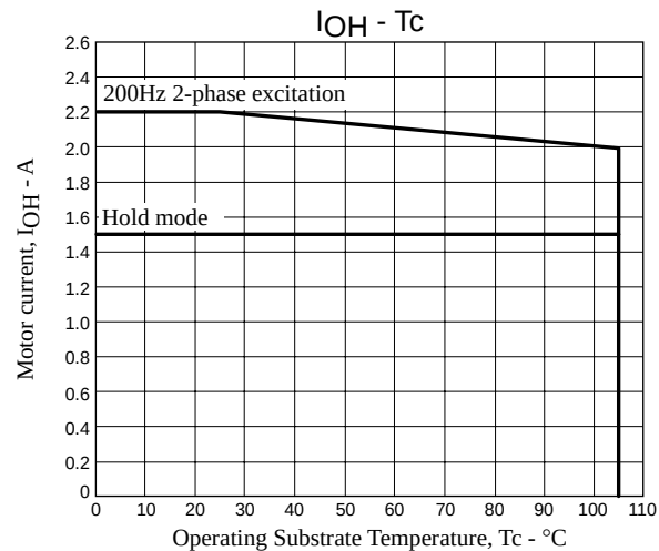
Derating Curve of Motor Current, I_{OH} , vs. STK672-400C-E Operating Substrate Temperature, T_c
