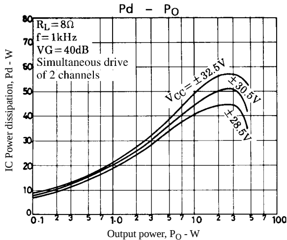
Figure 1. STK4161V P_d - P_O ( R_L = 8\Omega )
