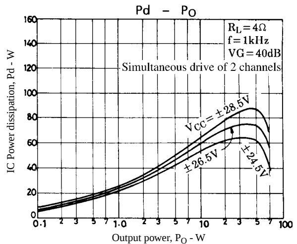
Figure 2. STK4161V P_d - P_O ( R_L = 4\Omega )
