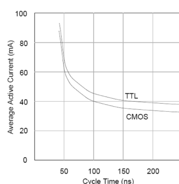
Figure 5. Current Versus Cycle Time (WRITE)
