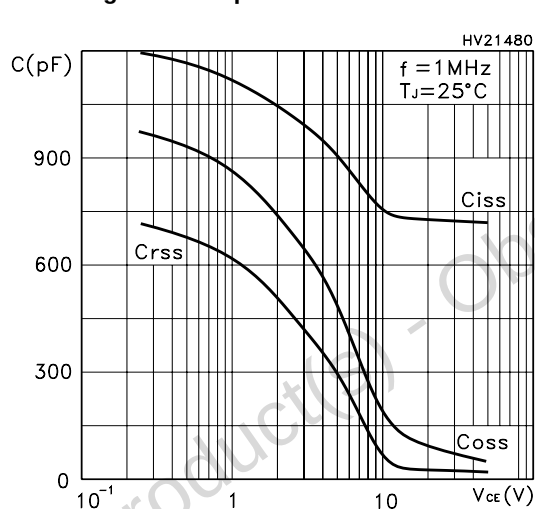
Figure 10: Capacitance variations
