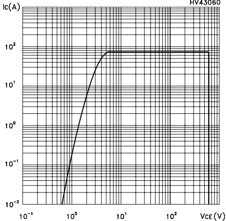
Figure 13: Turn-off SOA
