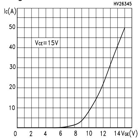
Figure 3: Transfer characteristics
