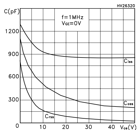
Figure 7: Capacitance variations
