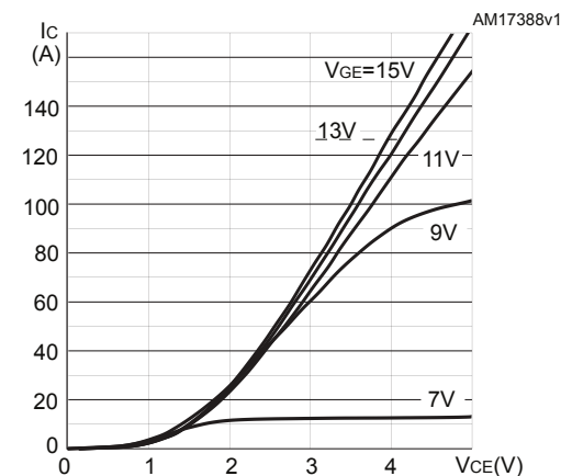
Figure 6. Output characteristics (T J = 175 °C)
