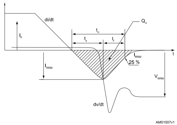
Figure 36. Diode reverse recovery waveform
