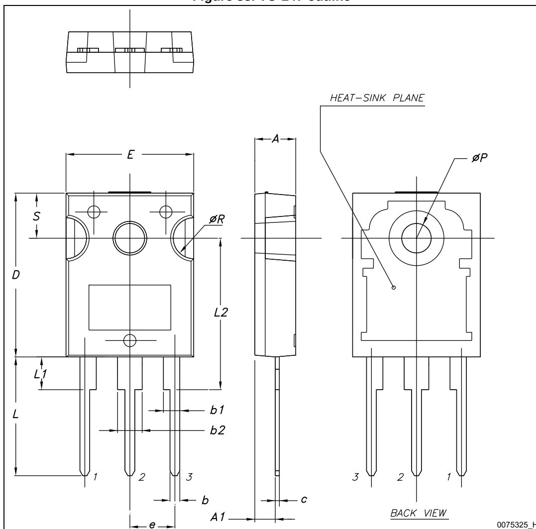
Figure 33. TO-247 outline
