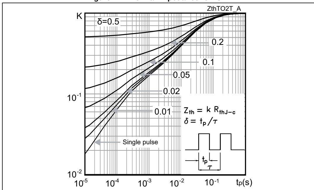
Figure 27. Thermal impedance for IGBT
