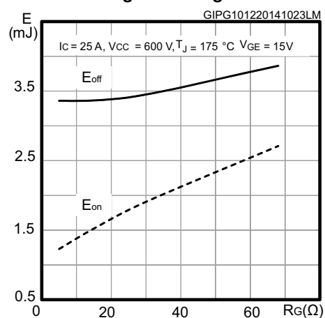
Figure 17. Switching loss vs. gate resistance
