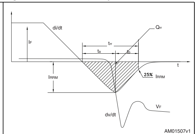
Figure 22. Diode recovery time waveform
