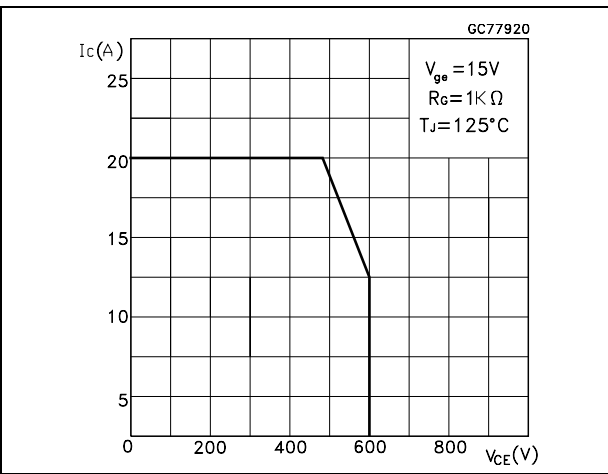
Figure 16. Turn-off SOA
