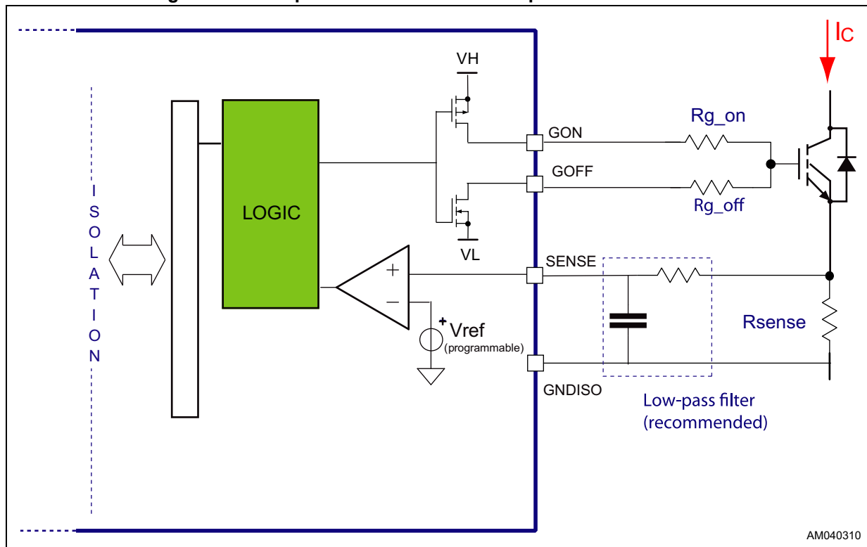
Figure 15. Example of SENSE overcurrent protection connection
