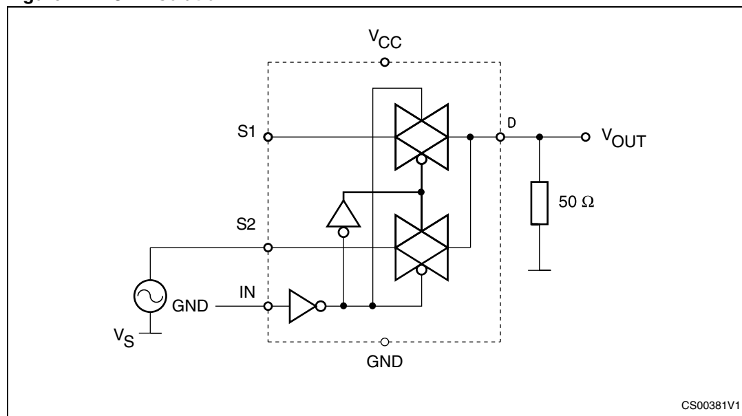
Figure 7. OFF isolation
