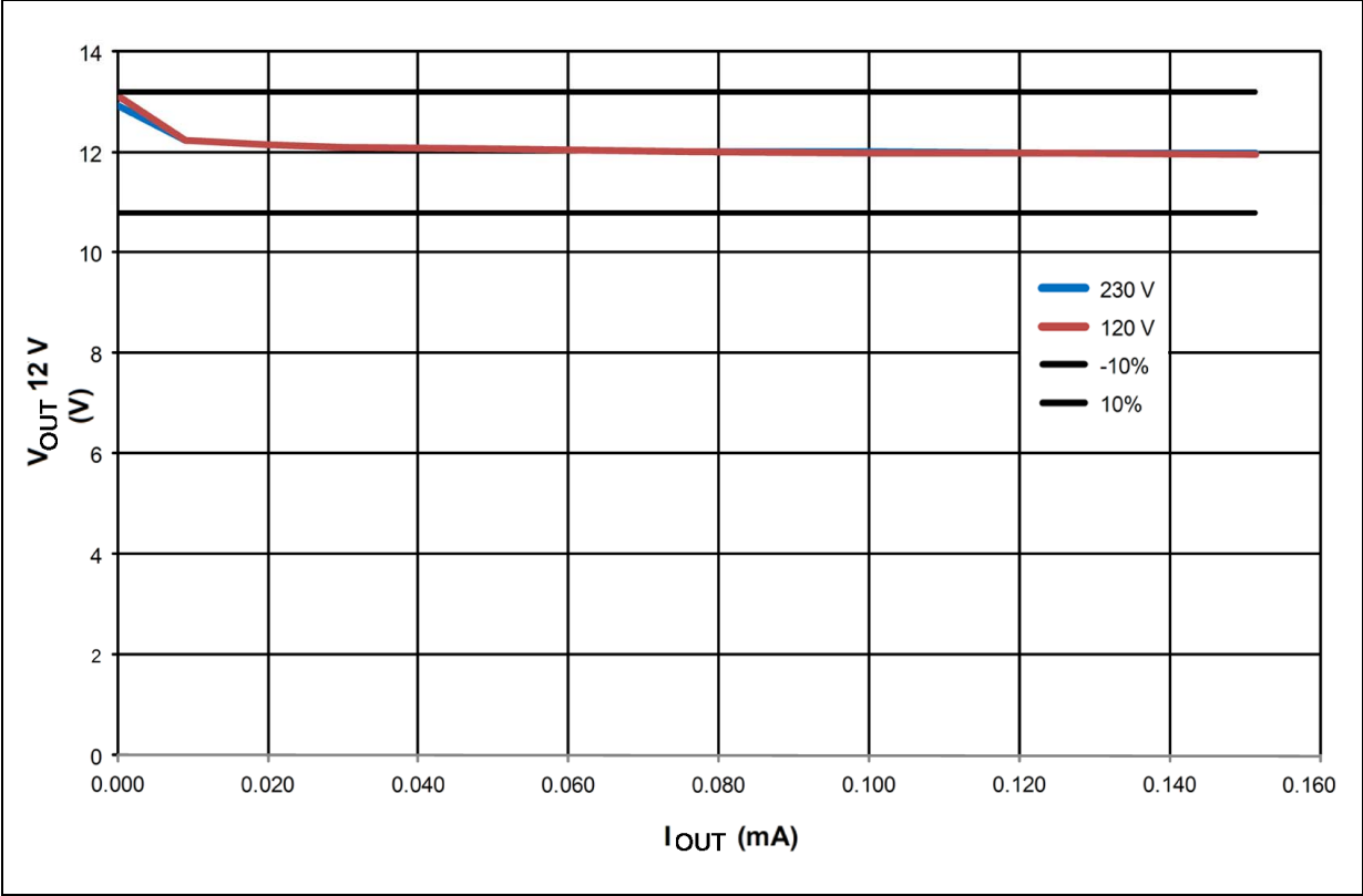
Figure 8. The 12 V output load characteristics
