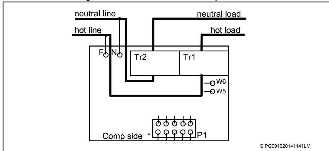
Figure 1: Connection of two CTs to the power line
