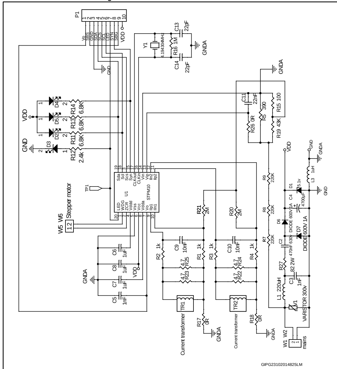
Figure 7: STEVAL-IPE015V1 schematic
