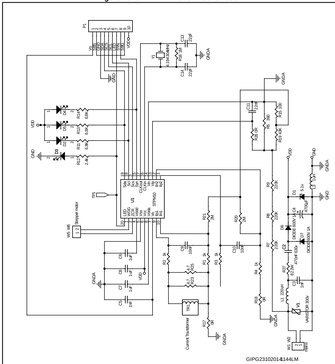
Figure 10: STEVAL-IPE018V1 schematic
