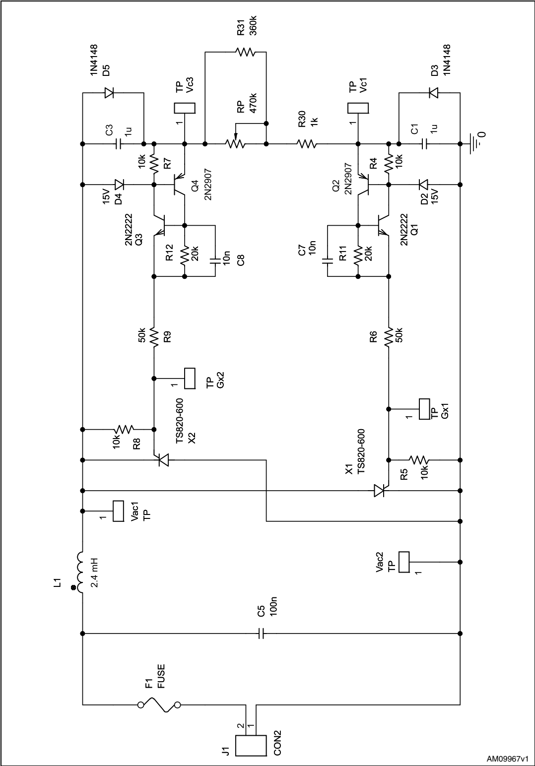
Figure 1. STEVAL-ILD003V1 schematic
