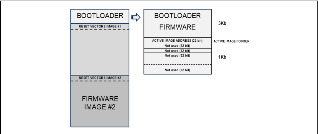
Figure 7. Memory organization
