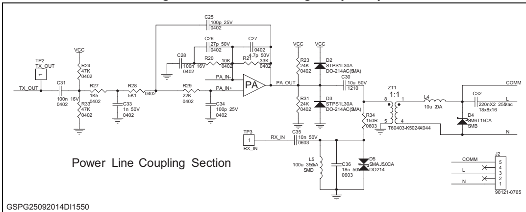
Figure 15. Schematic diagram (4 of 5)
