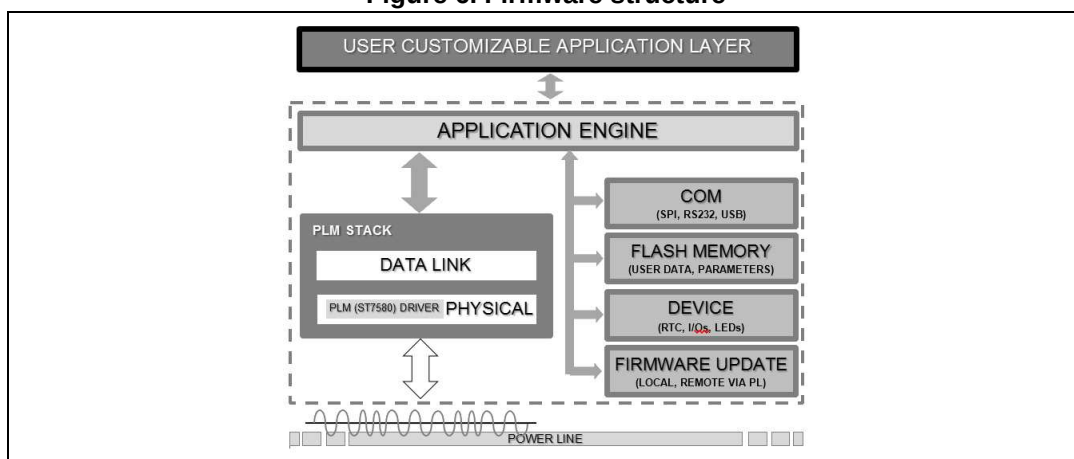
Figure 6. Firmware structure
