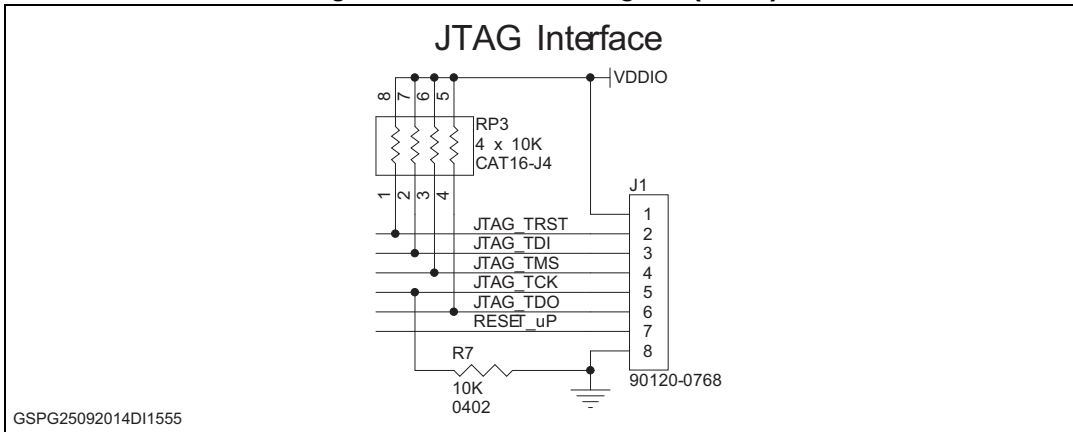
Figure 16. Schematic diagram (5 of 5)
