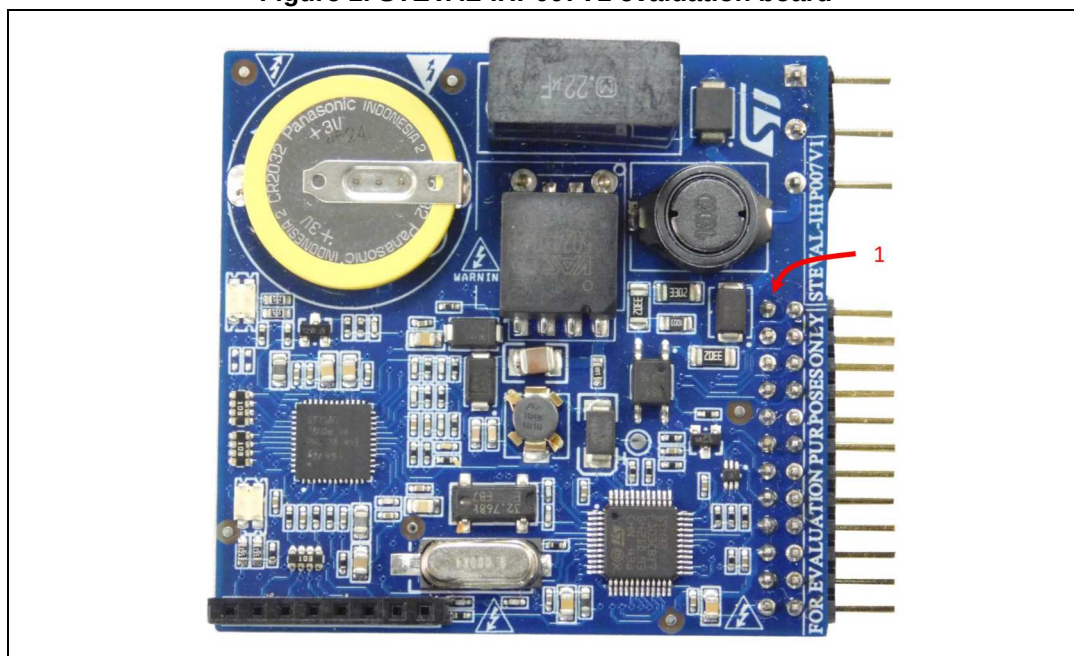
Figure 1. STEVAL-IHP007V1 evaluation board
