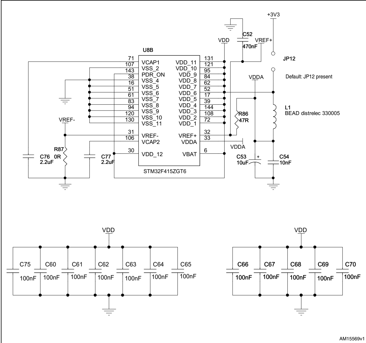
Figure 9. Power (2 of 2)
