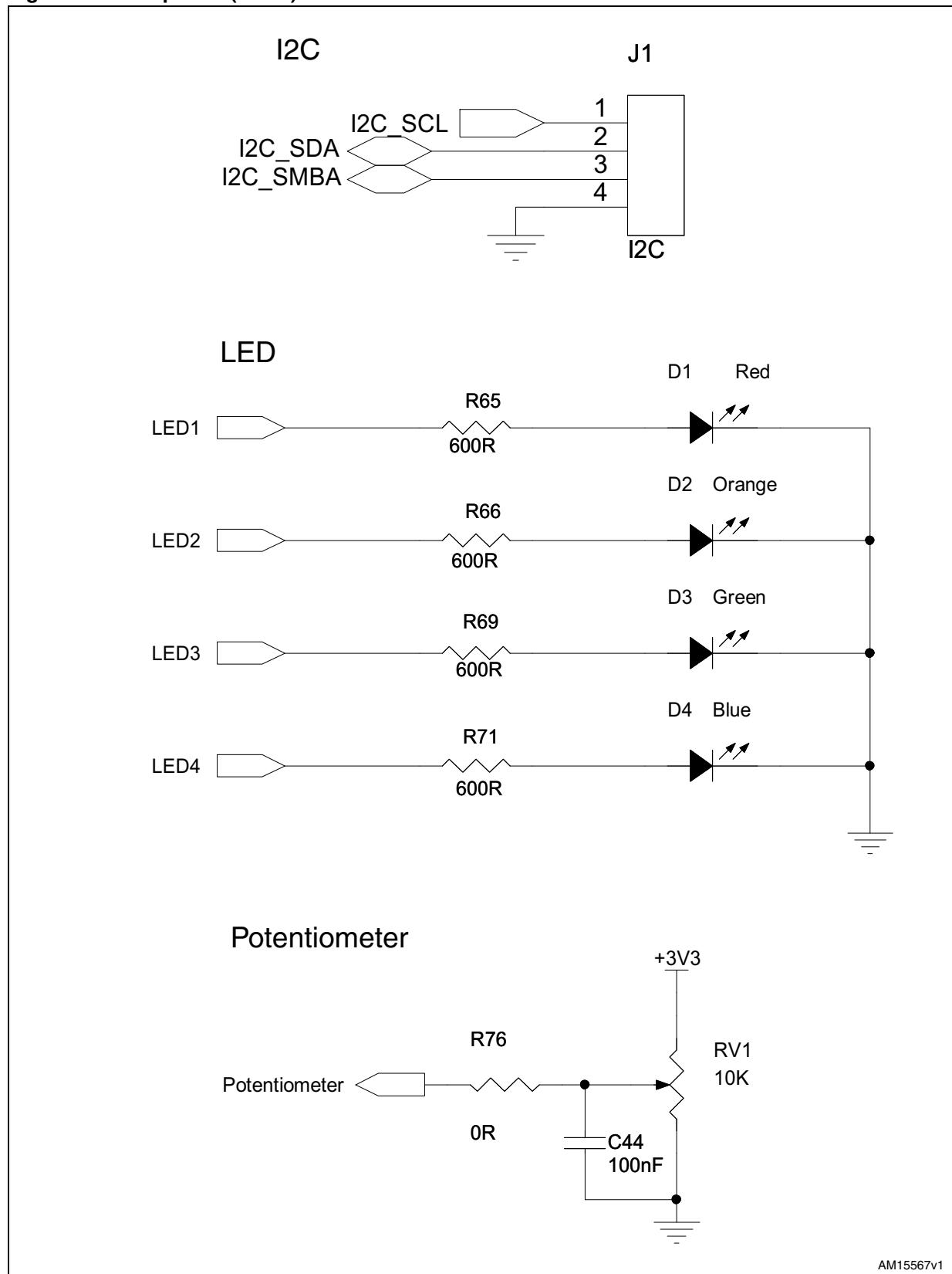
Figure 7. Peripheral (2 of 2)
